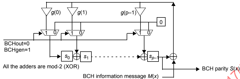
Figure 115-19—BCH encoder
