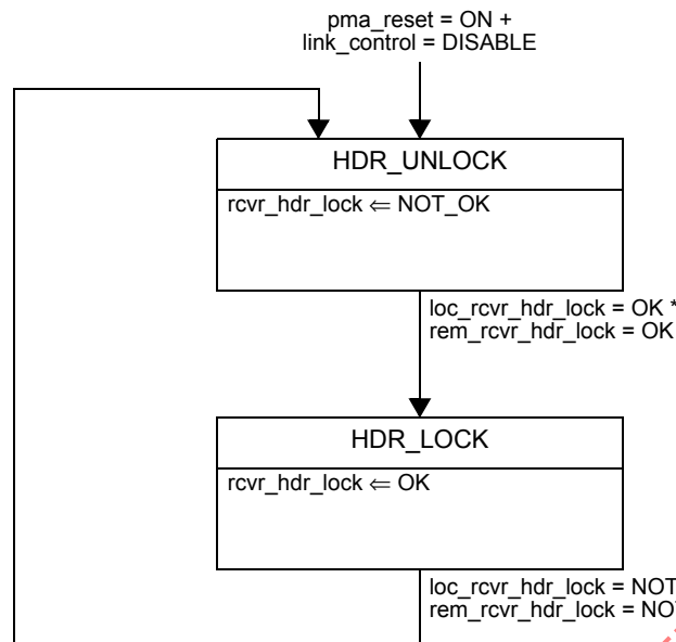
Figure 115-27—PHD monitor state diagram
