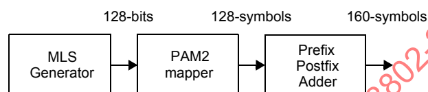
Figure 115–6—Pilot S1 generator
