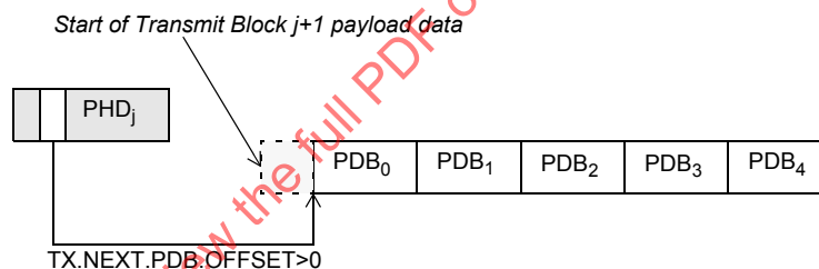
Figure 115–15—PDB alignment
