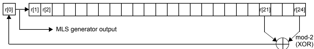
Figure 115-7—MLS generator
