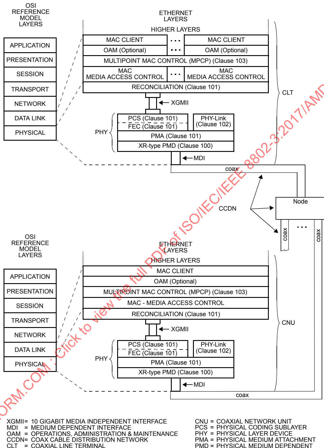
Figure 56-4a—Architectural positioning of EFM: P2MP EPoC architecture (up to 10 Gb/s downstream, up to 1.6 Gb/s upstream)
