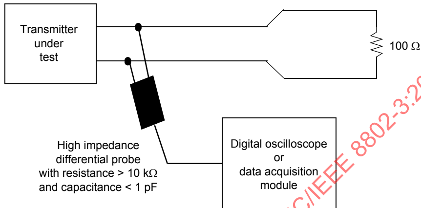
Figure 97–29—Transmitter test fixture 1 for transmitter droop measurement
