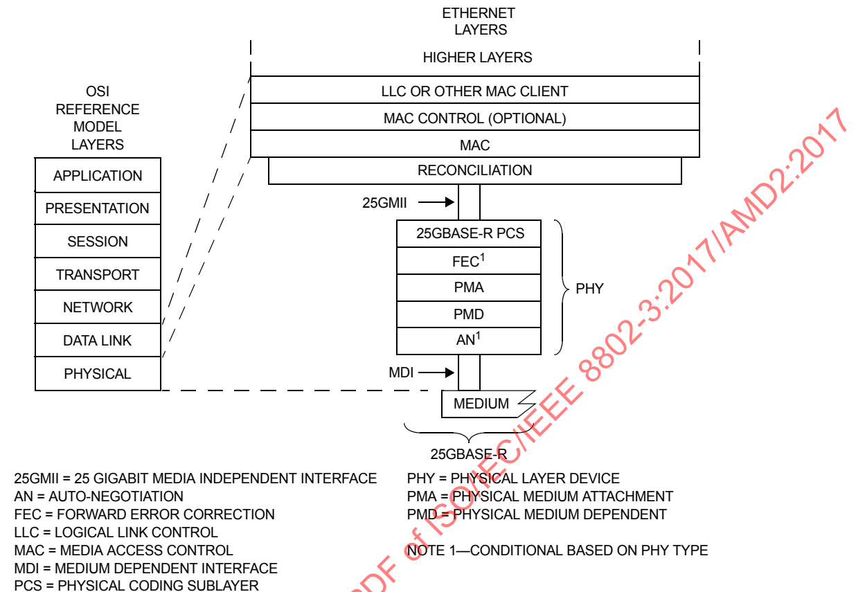
Figure 105-1—Architectural positioning of 25 Gigabit Ethernet
