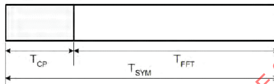
Figure 160e—OFDM symbol format
