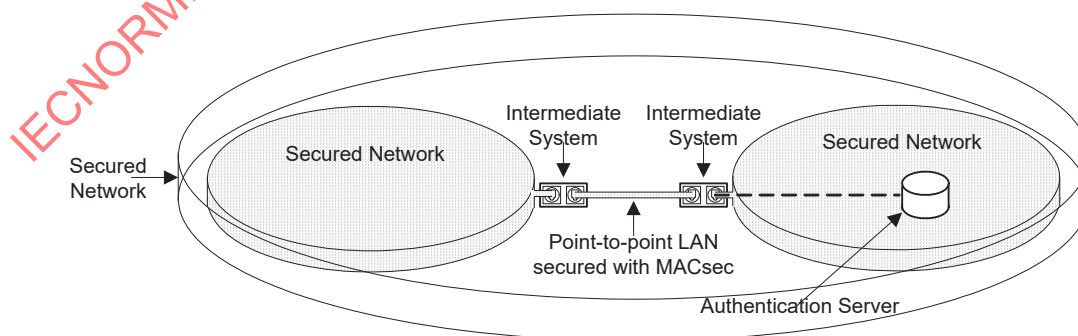
Figure 7-8—Point-to-point LAN within a secured network
