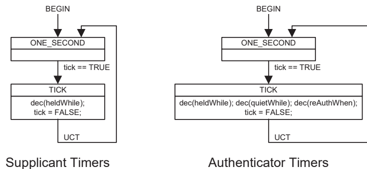
Figure 8-5—PAE Timer state machines
