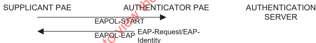
Figure 8-3—Supplicant-initiated EAP exchange
