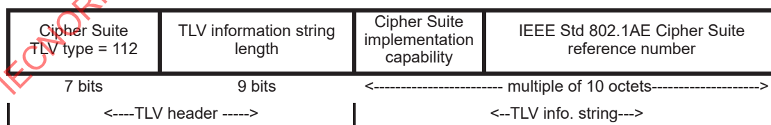
Figure 11-22—MACsec Cipher Suites TLV format
