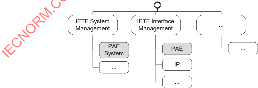
Figure 14-2—YANG object hierarchy with IEEE Std 802.1X
