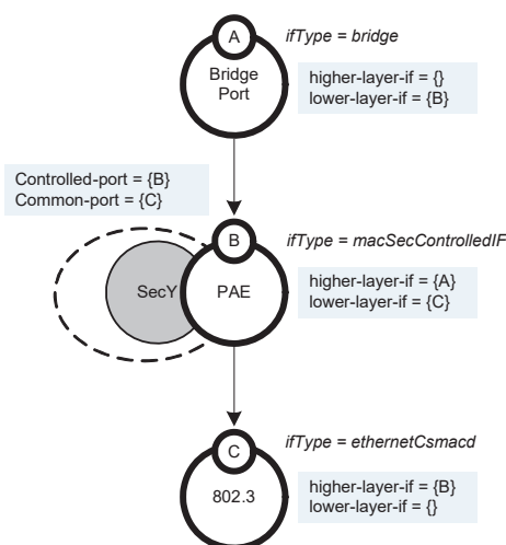
Figure 14-8—Bridge Port YANG Interface stack model with MACsec
