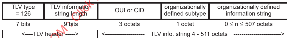
Figure 11-25—Organizationally Specific Set TLV format
