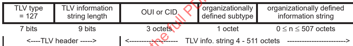
Figure 11-24—Organizationally Specific TLV format
