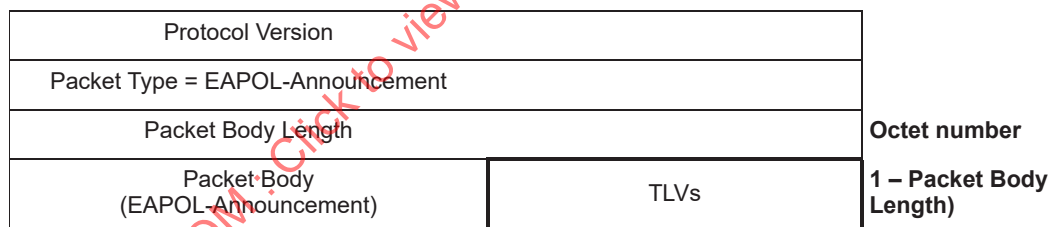
Figure 11-18—EAPOL-Announcement
