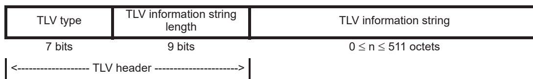
Figure 11-19—EAPOL-Announcement TLV format
