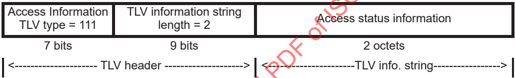
Figure 11-21—Access Information TLV format
