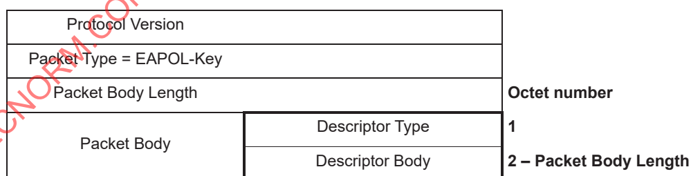
Figure 11-5—EAPOL-Key Packet Body with Key Descriptor format
