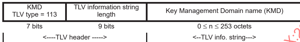
Figure 11-23—Key Management Domain TLV format
