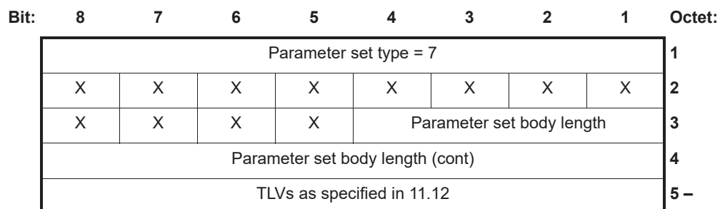
Figure 11-15—Announcement parameter set
