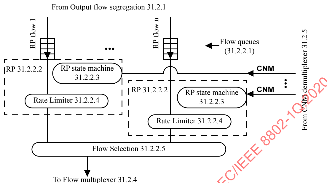
Figure 31-3—Per-CNPV station function
