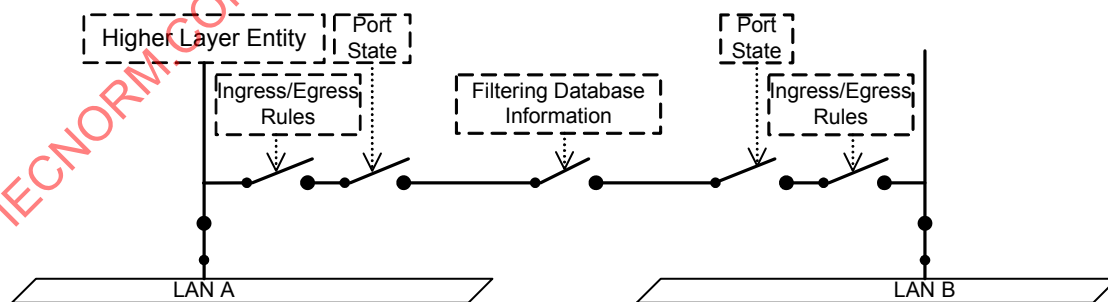
Figure 8-26—Ingress/egress control information in the forwarding path
