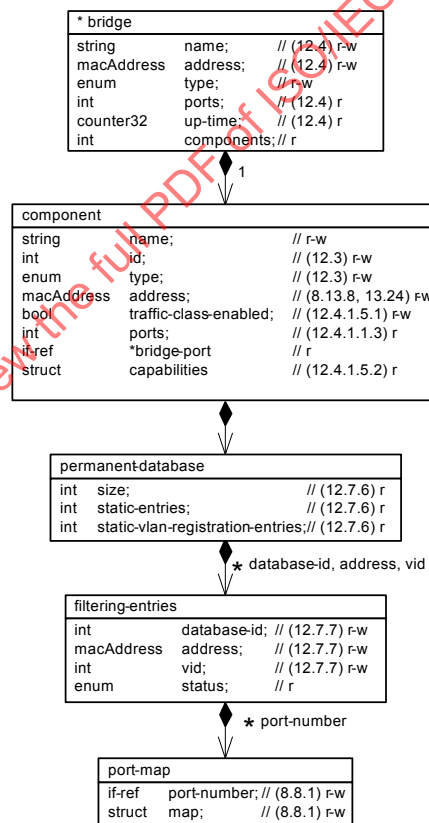
Figure 48-6—TPMR model
