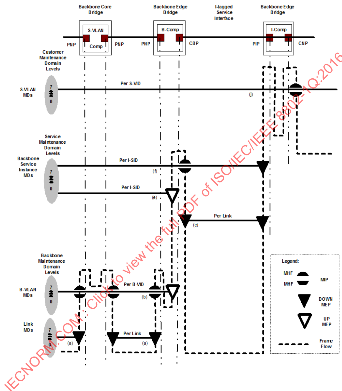
Figure 26-4—CFM example applied to an I-tagged Service Interface
