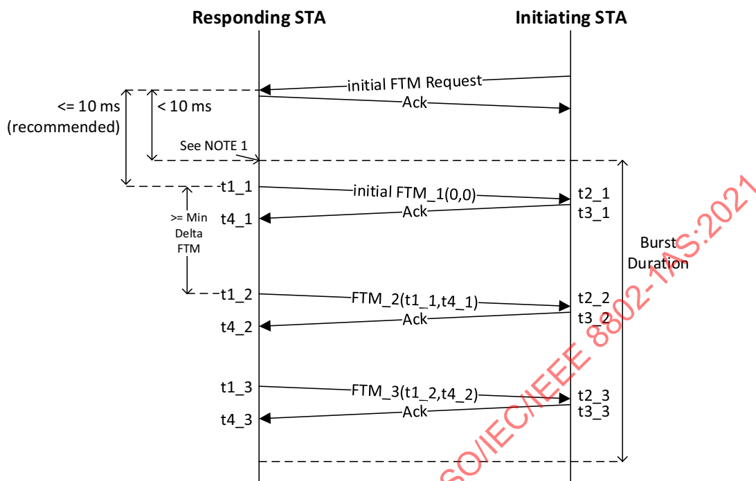
Figure 12-3—Illustration of Fine Timing Measurement burst
