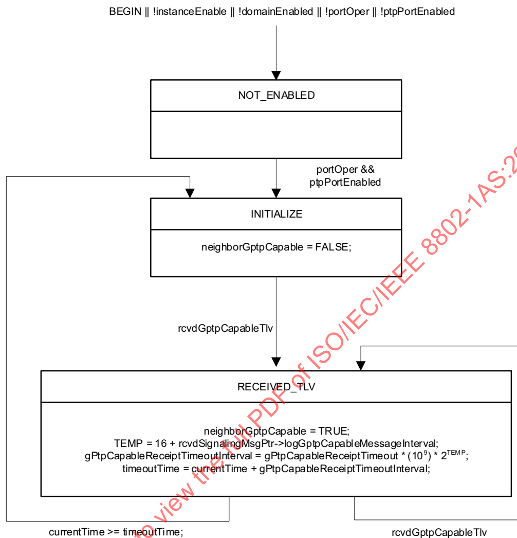
Figure 10-22—GtpCapableReceive state machine
