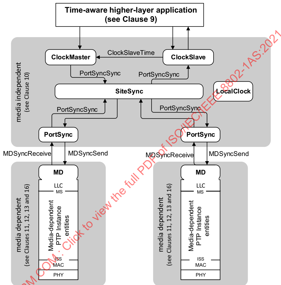
Figure 7-8—PTP Instance model
