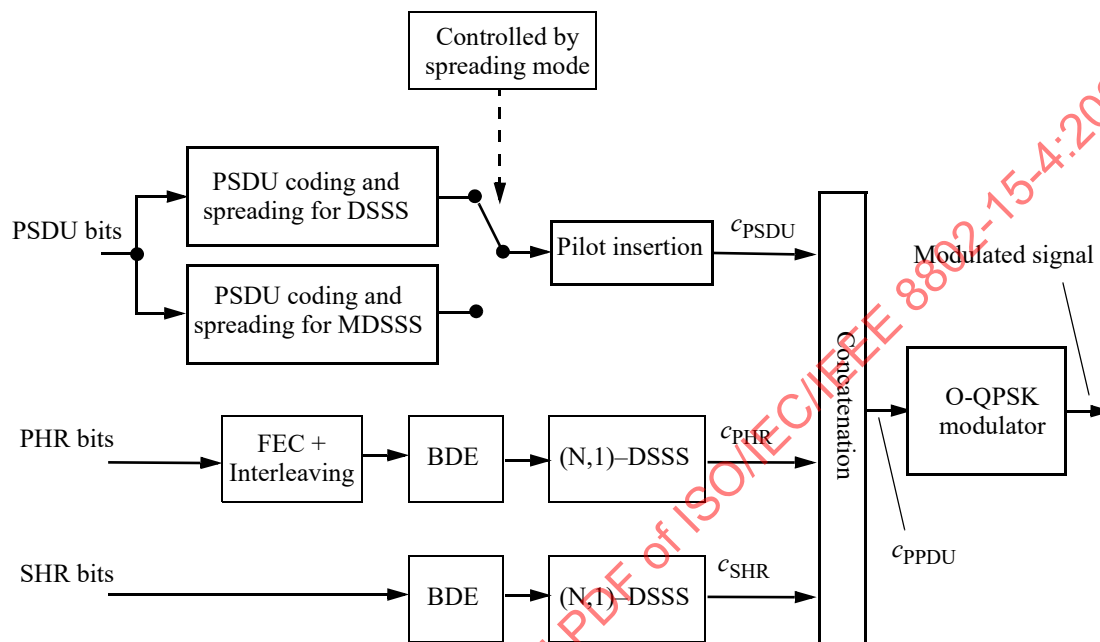
Figure 21-7—Reference modulator diagram
