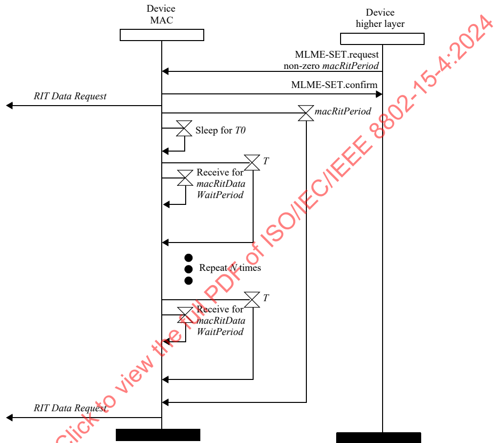
Figure 6-68—Message sequence chart for RIT with the RIT Data Request carrying a payload
