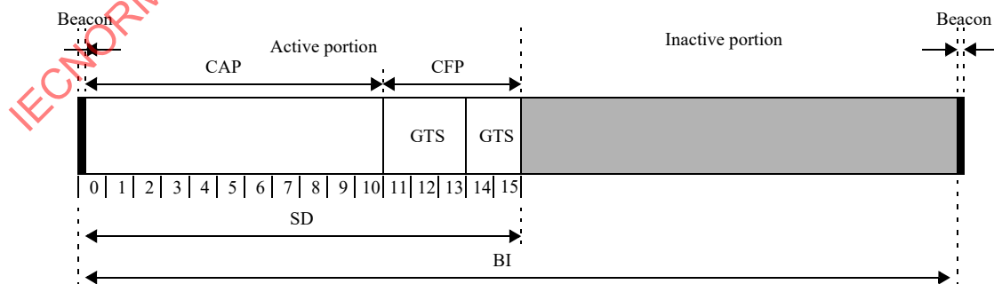
Figure 6-1—An example of the superframe structure
