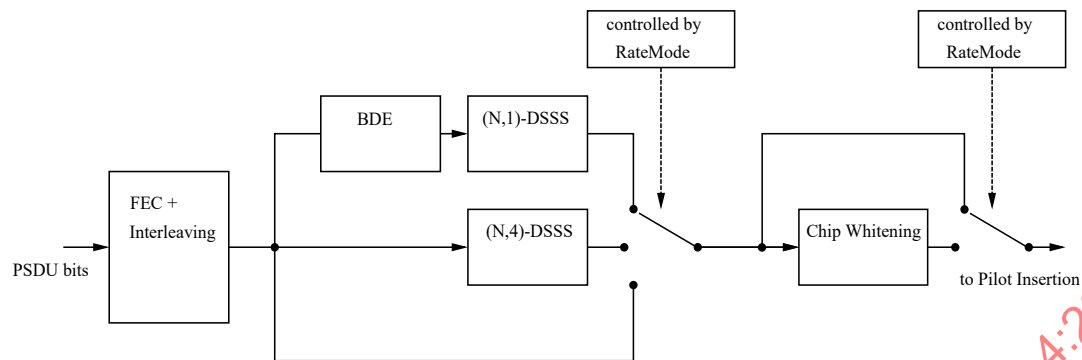
Figure 21-8—PSDU processing for DSSS
