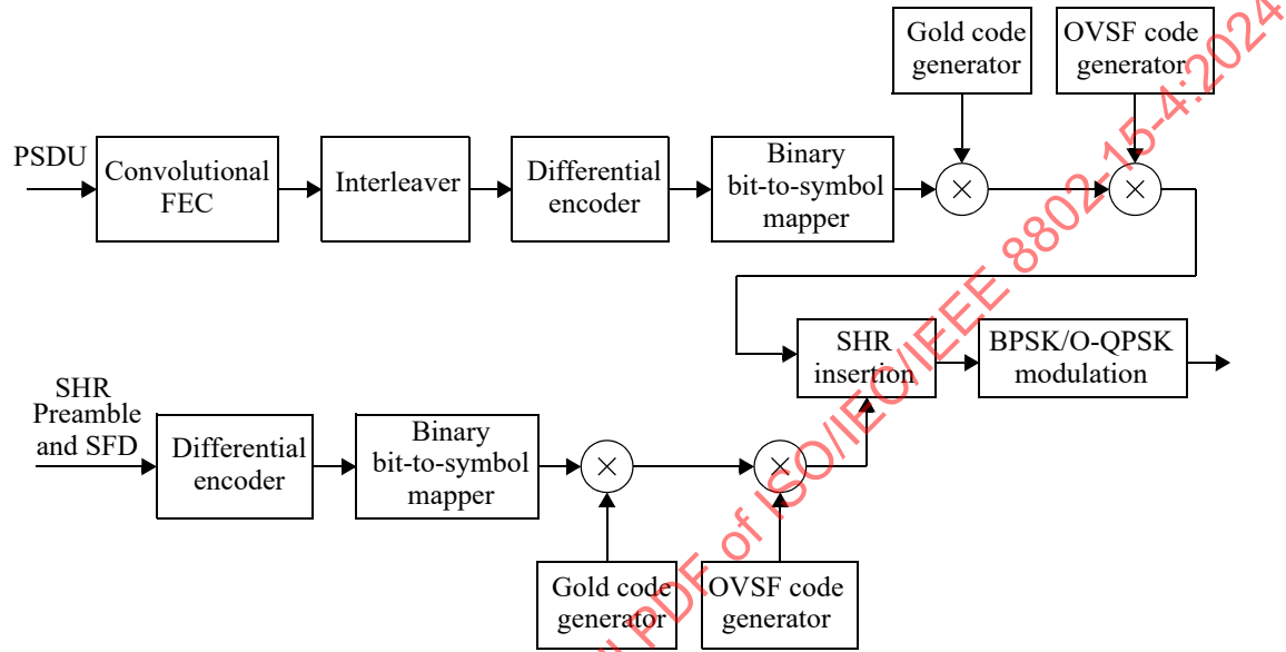
Figure 22-2—LECIM DSSS reference modulator diagram
