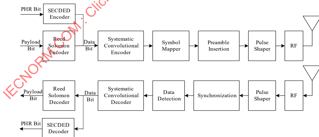
Figure 15-1—HRP UWB PHY signal flow
