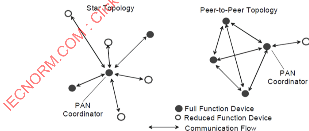
Figure 5-1—Star and peer-to-peer topology examples
