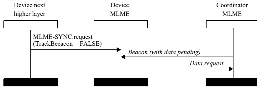
Figure 6-27—Synchronizing to a coordinator in a beacon-enabled PAN without tracking beacons
