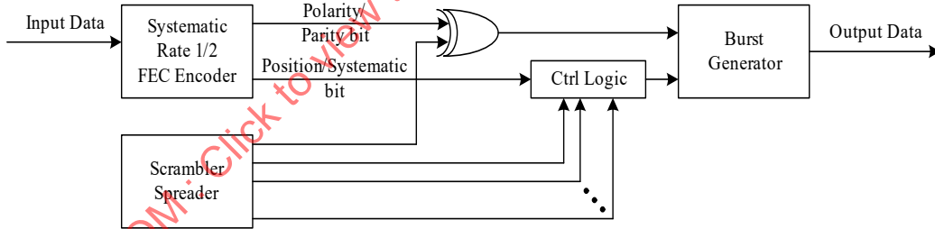
Figure 15-8—Reference modulator
