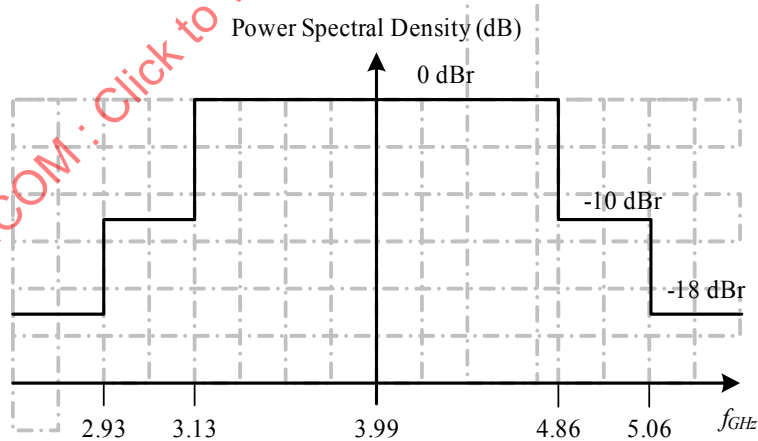
Figure 16-14—Transmit spectrum mask for band 4
