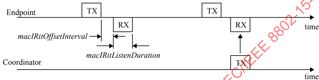
Figure 6-71—I-RIT transmission
