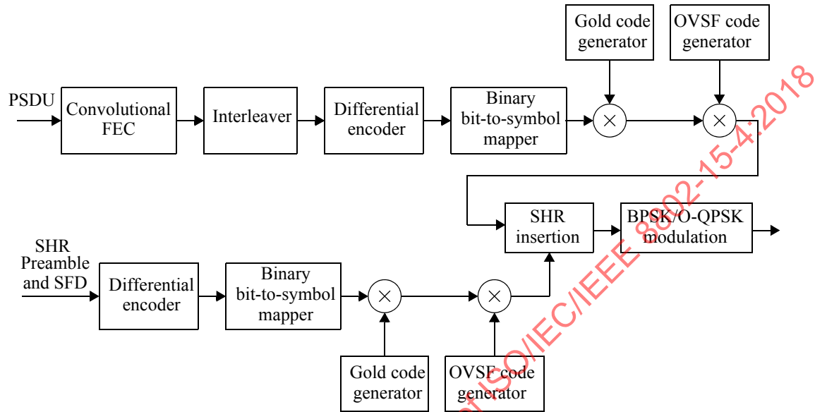
Figure 23-2—LECIM DSSS reference modulator diagram
