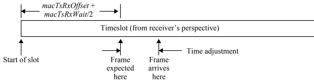
Figure 6-31—Time synchronization
