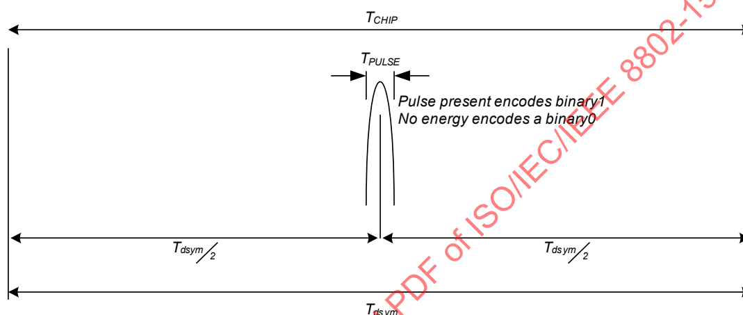
Figure 19-1—Base mode LRP UWB PHY symbol structure
