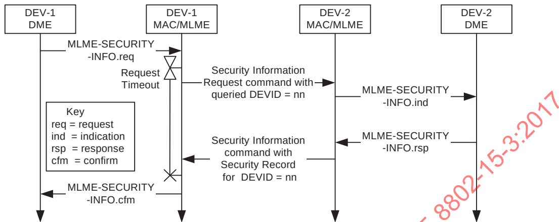
Figure 8-1—MSC for DEV-DEV Security Information request
