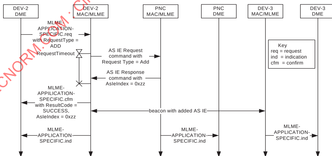
Figure 7-74—MSC for a DEV adding an AS IE to the beacon
