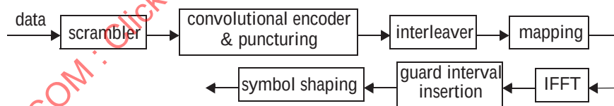
Figure 11-40—LRP reference implementation block diagram
