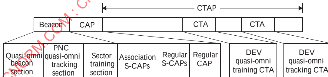
Figure 7-42—Superframe structure for quasi-omni capable PHYs
