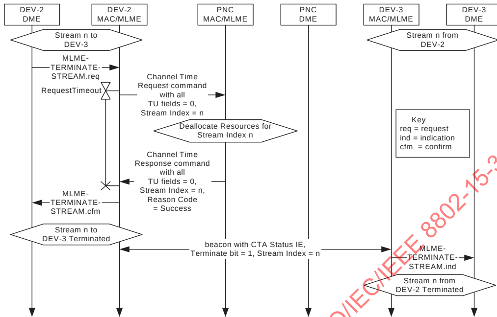
Figure 7-35—MSC of source DEV-2 requesting termination of its stream
