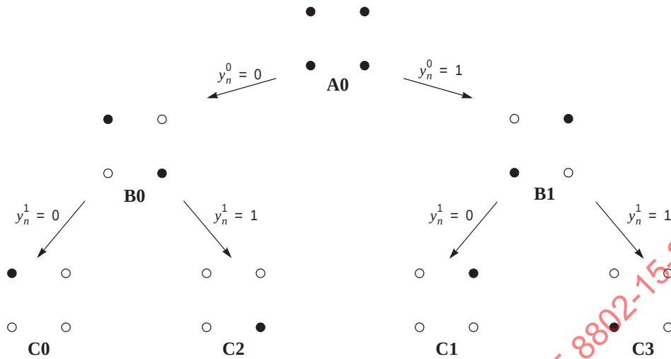
Figure 10-5—QPSK set partitioning
