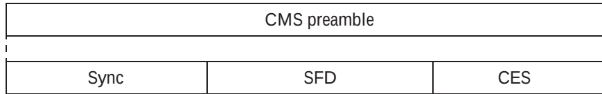
Figure 11-7—PHY preamble structure for CMS
