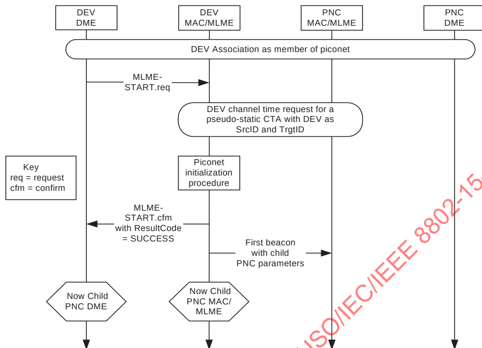
Figure 7-11—MSC for creating a child piconet
