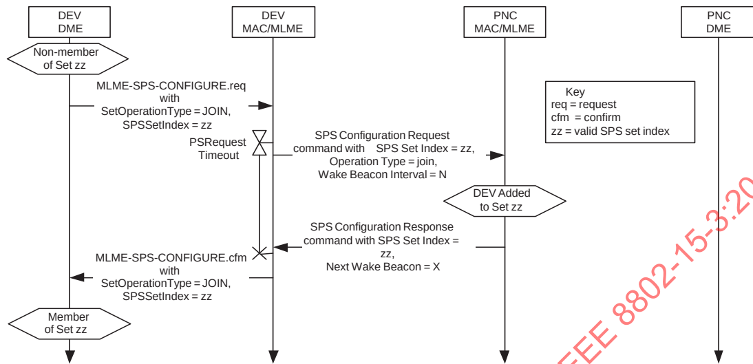
Figure 7-68—MSC showing a DEV joining an existing SPS set
