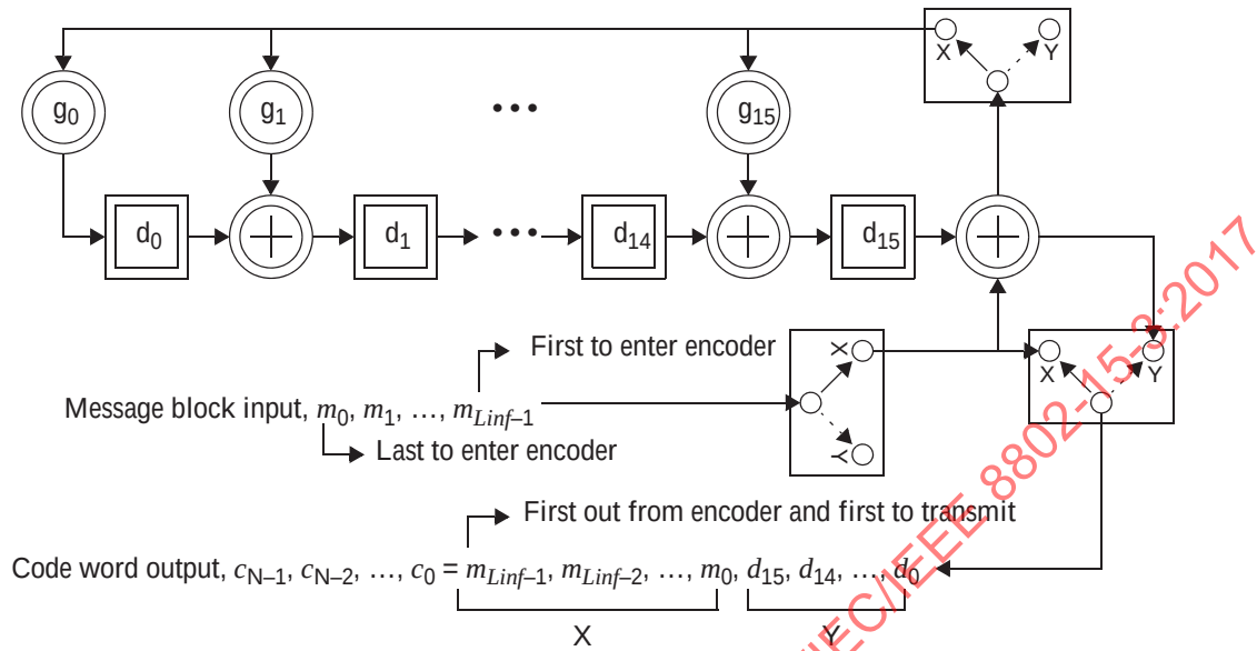
Figure 11-12—Reed Solomon encoder GF(2 8 )
