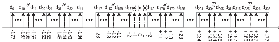
Figure 11-30—Subcarrier frequency allocation
