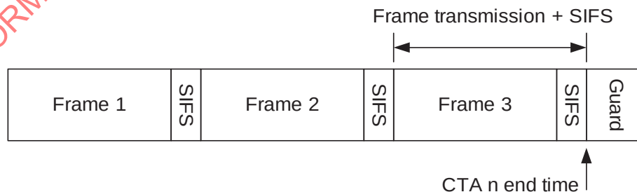
Figure 7-23—SIFS and Guard time at the end of a CTA—no-ACK
