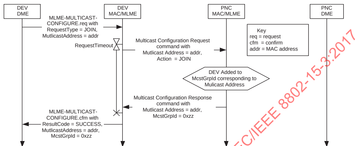
Figure 7-39—MSC for a DEV successfully joining a multicast group
