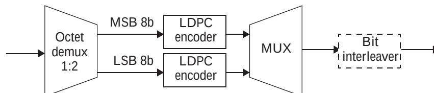
Figure 11-26—FEC process for the HSI PHY
