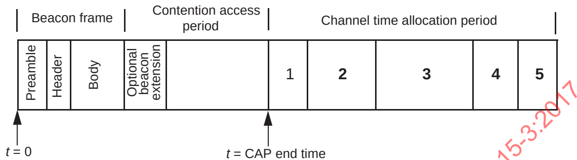
Figure 7-41—Piconet timing relative to the beacon
