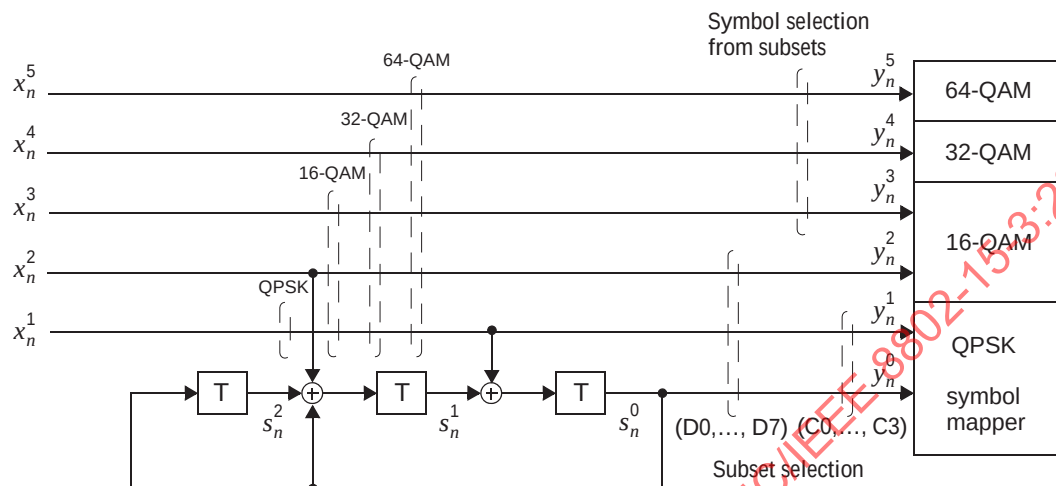
Figure 10-4—QPSK, 16/32/64-QAM 8-state trellis encoder
