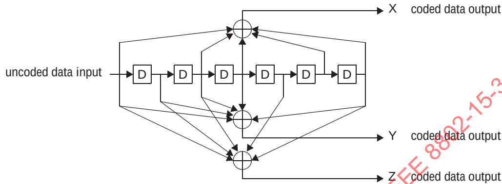
Figure 11-42—Convolutional encoder reference implementation
