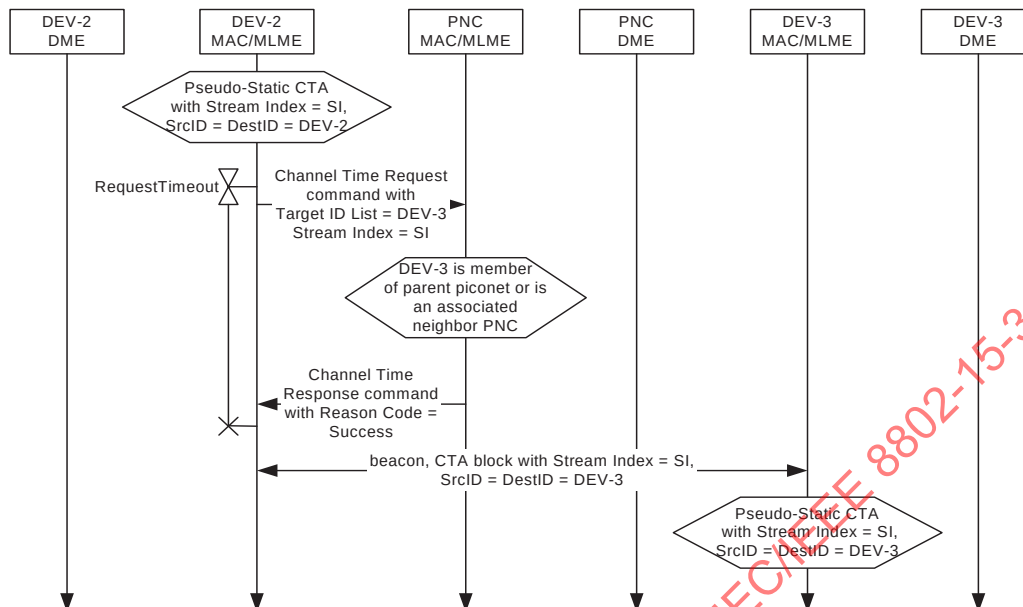
Figure 7-34—MSC for handing over control of a private, pseudo-static CTA
