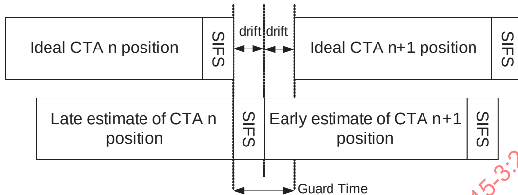
Figure 7-22—Guard time
