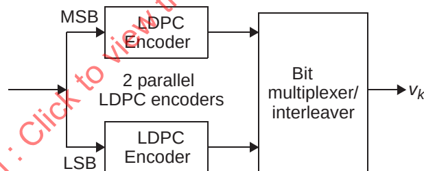
Figure 11-15—Parallel encoders for UEP
