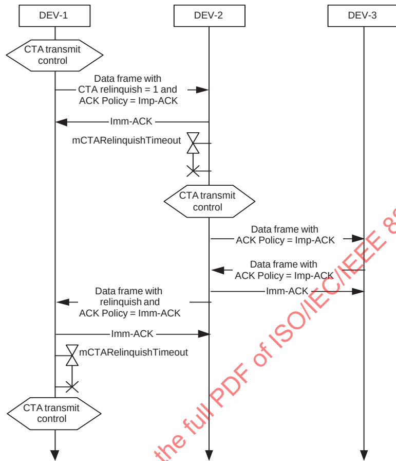
Figure 7-29—MSC for relinquishing CTA time when the target DEV has data to send
