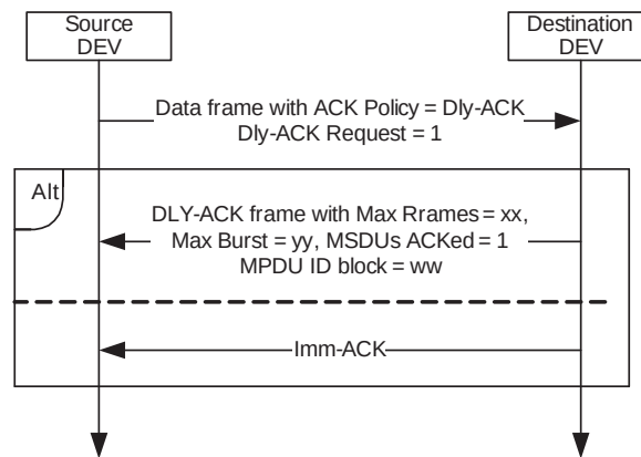
Figure 7-55—MSC for Dly-ACK negotiation
