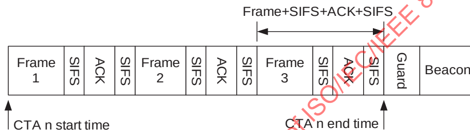
Figure 7-25—Guard time at the end of the superframe
