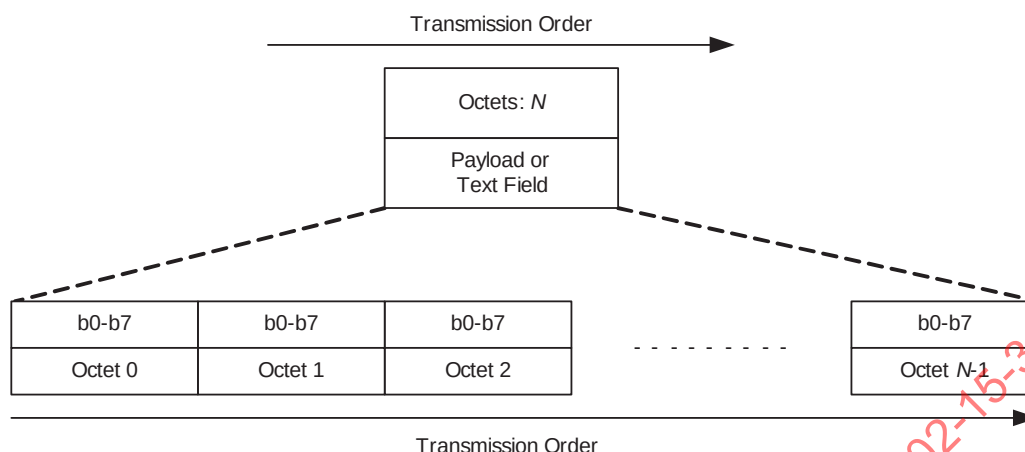
Figure 6-2—Example of payload transmission order
