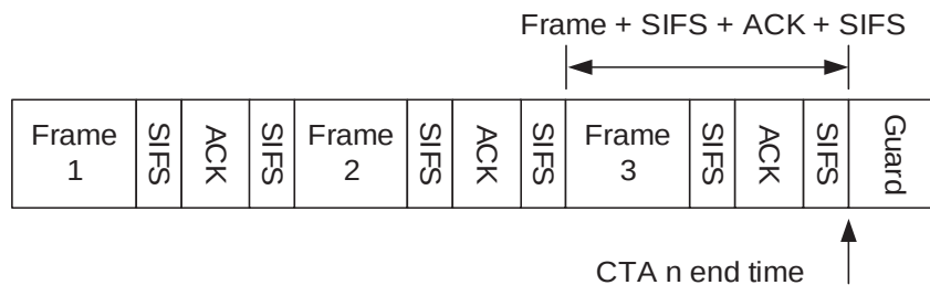
Figure 7-24—SIFS, ACK, SIFS, and Guard time at the end of a CTA—Imm-ACK
