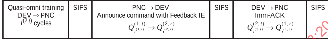
Figure 7-48—CTA structure for DEV quasi-omni transmit direction training
