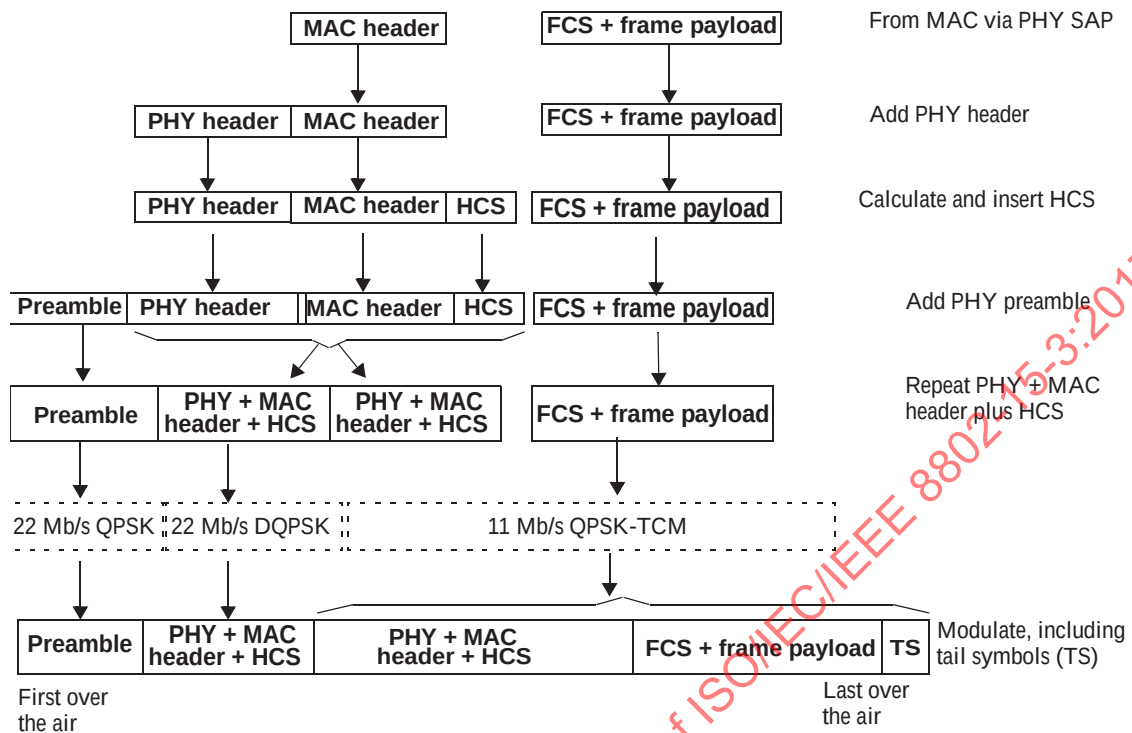
Figure 10-14—PHY frame formatting for 11 Mb/s mode
