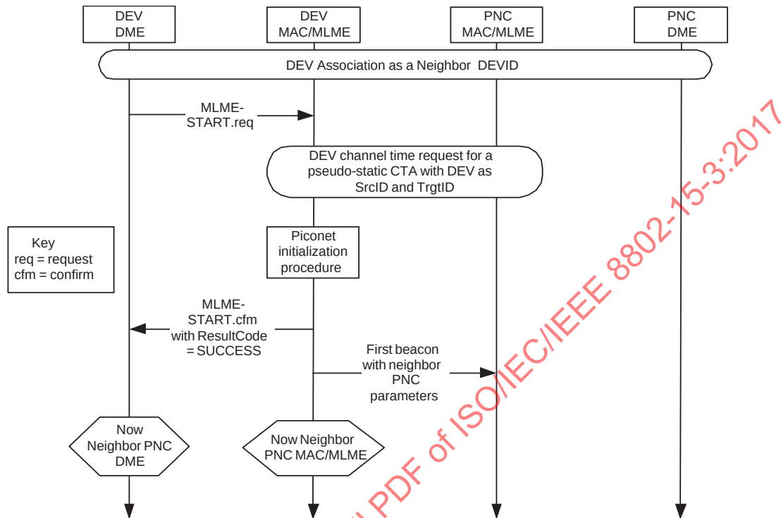
Figure 7-13—MSC for initiating a neighbor piconet
