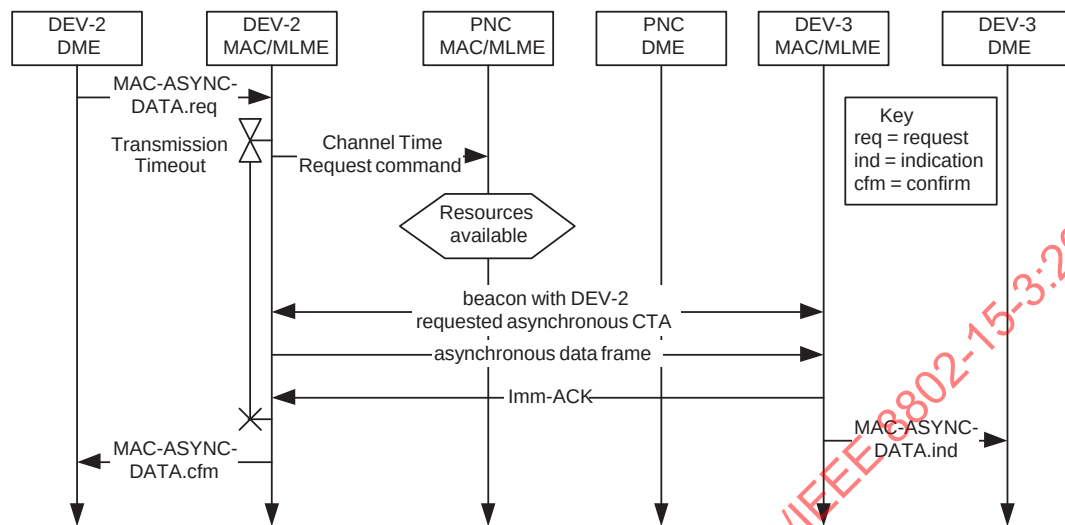
Figure 7-38—MSC for reserving asynchronous data channel time
