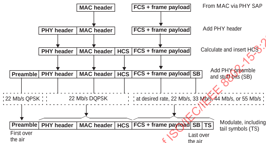
Figure 10-13—PHY frame formatting for 22 Mb/s, 33 Mb/s, 44 Mb/s, and 55 Mb/s modes
