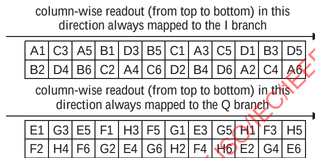
Figure 11-46—UEP mapping mode overall multiplexing and bit interleaving pattern
