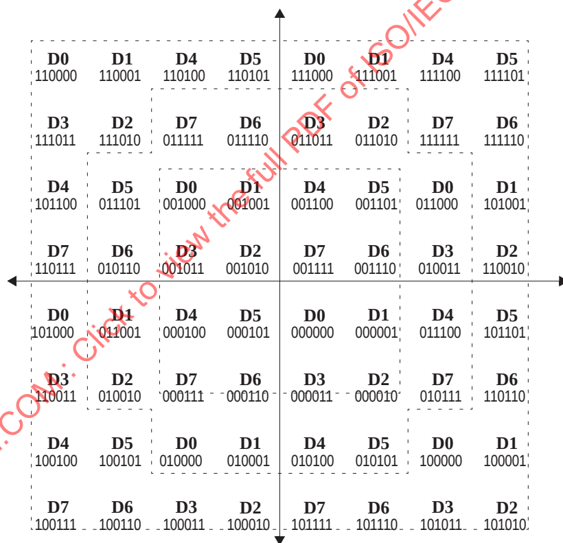
Figure 10-10—16/32/64-QAM constellation bit mappings
