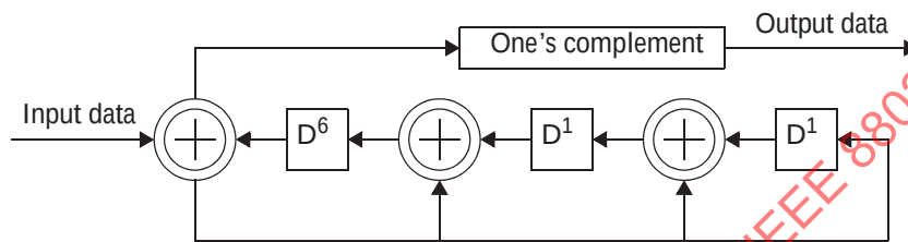
Figure 6-24—HCS implementation example for MSDU subheader
