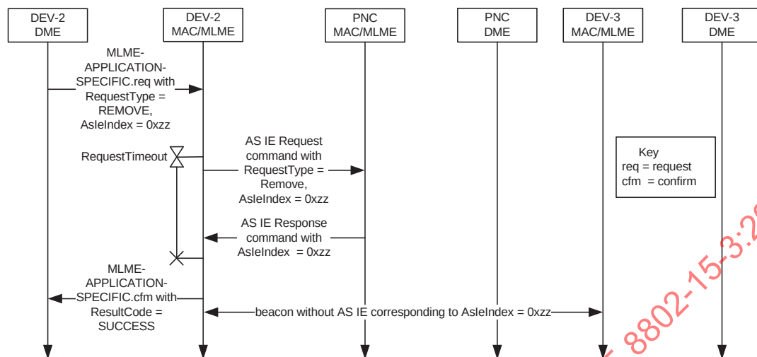
Figure 7-76—MSC for a DEV removing an AS IE from a beacon
