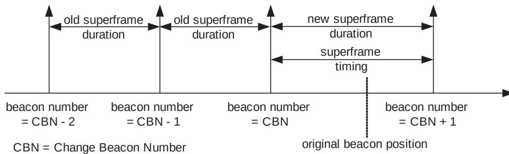
Figure 7-60—Changing superframe duration
