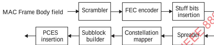
Figure 11-23—SC PHY Payload field construction process
