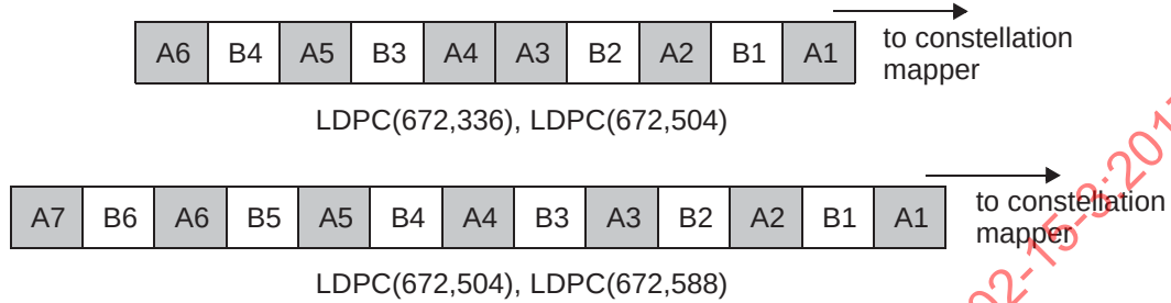
Figure 11-16—UEP bit multiplexing/interleaving
