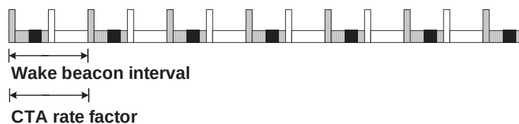
Case 2: Wake beacon interval = 2, CTA rate factor = 4
