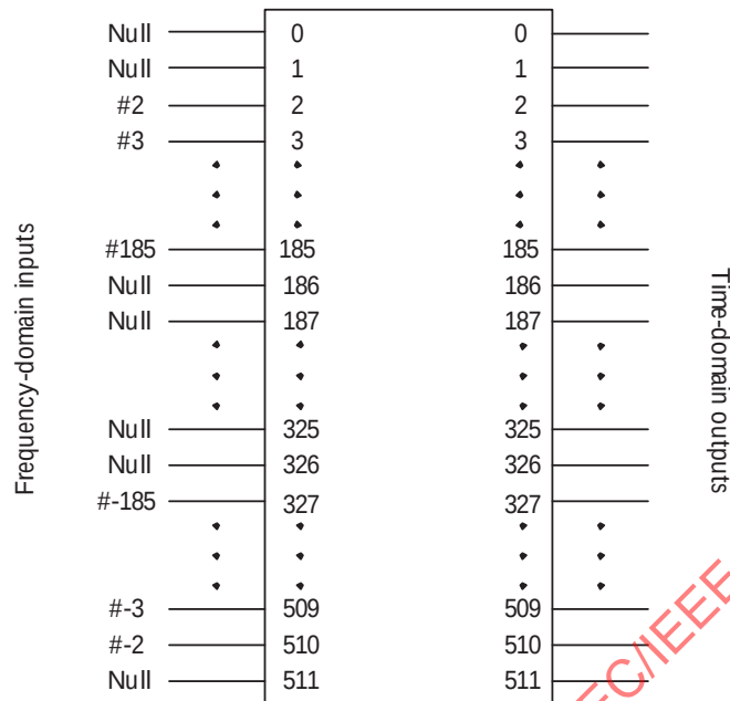
Figure 11-31—Input and output relationship of the IFFT
