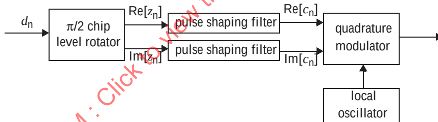
Figure 11-11—Possible \pi/2 BPSK modulator realizations
