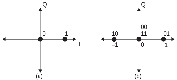
Figure 11-25—Constellation diagram for (a) OOK and (b) DAMI
