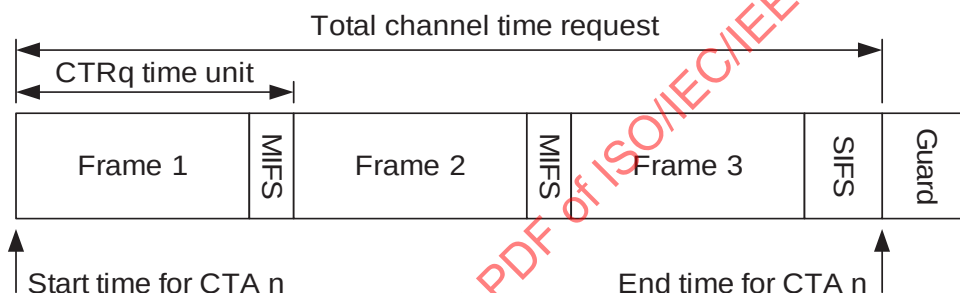
Figure 7-27—Channel time request with no ACKs
