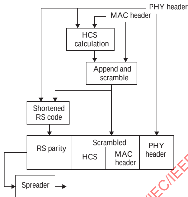
Figure 11-8—Frame header construction process for CMS
