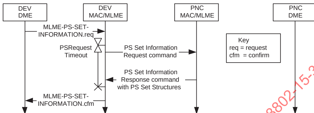
Figure 7-66—MSC for PS set information exchange
