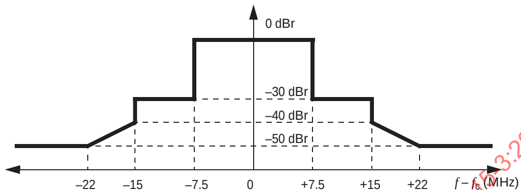
Figure 10-20—Transmit power spectral density mask
