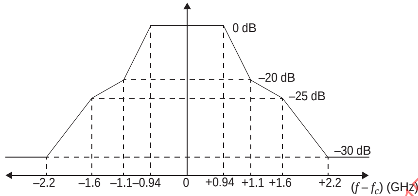
Figure 11-1—Transmit spectral mask
