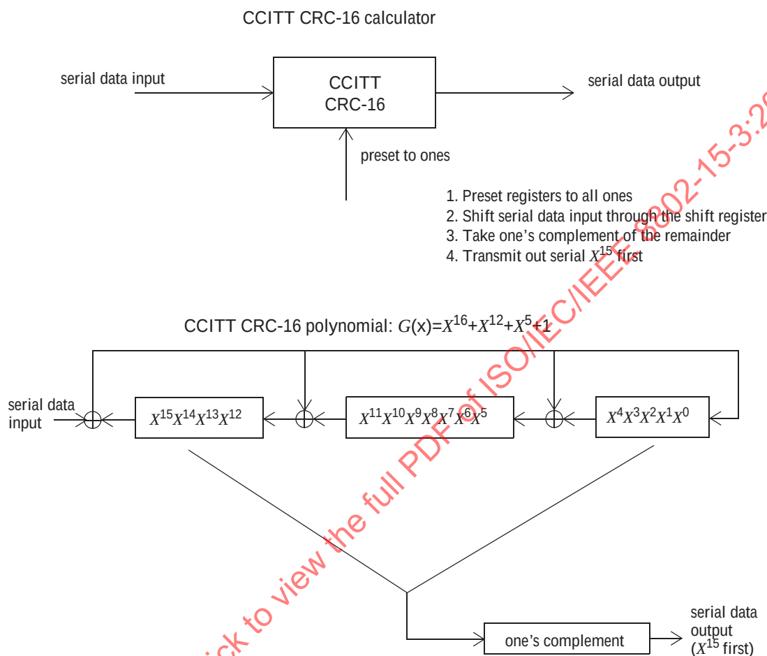
Figure 10-1—CCITT CRC-16 Implementation
