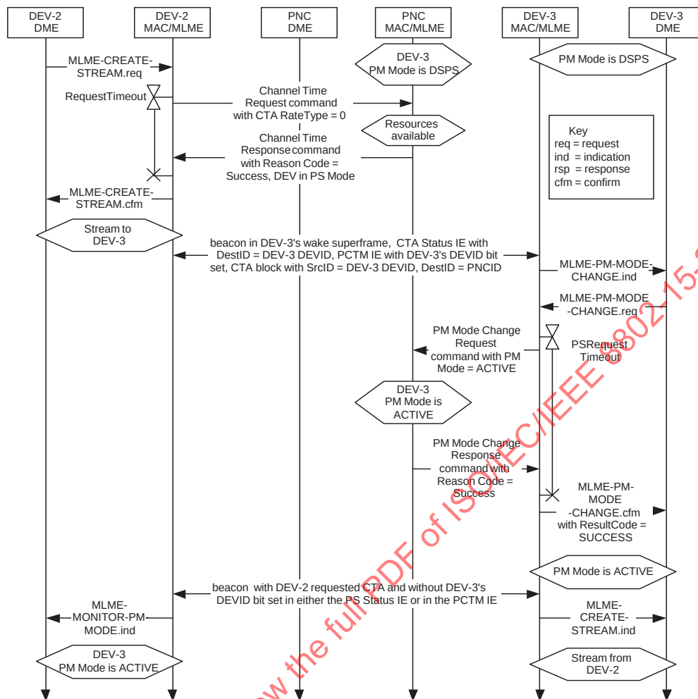
Figure 7-73—MSC showing MLME initiated PM mode change from DSPS to ACTIVE in response to a new channel time allocation
