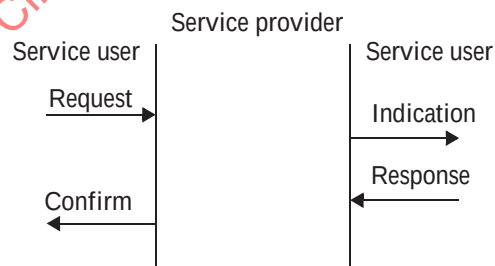
Figure 4-4—Service primitives
