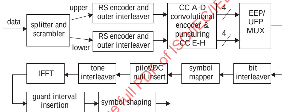
Figure 11-39—HRP reference implementation block diagram
