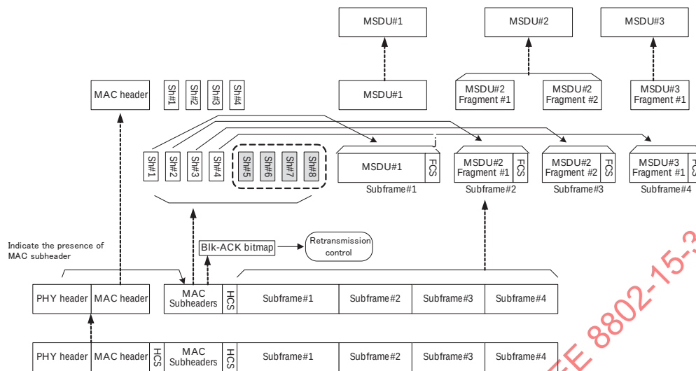
Figure 7-54—Deaggregation at target DEV
