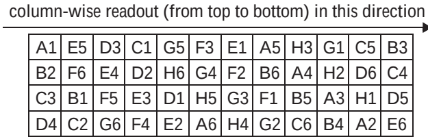
Figure 11-43—EEP multiplexing and bit interleaving pattern
