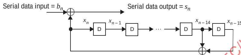
Figure 10-16—Realization of side-stream scrambler by linear feedback shift registers
