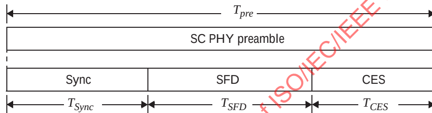
Figure 11-20—SC PHY preamble structure
