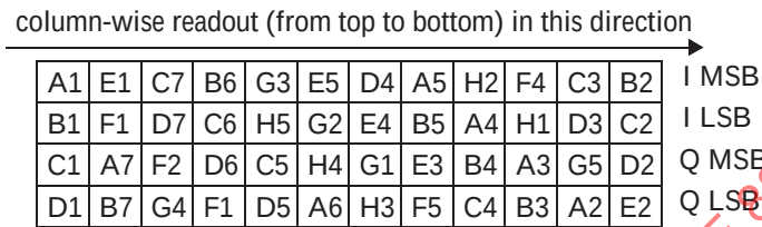
Figure 11-44—UEP coding mode first half cycle multiplexing and bit interleaving pattern
