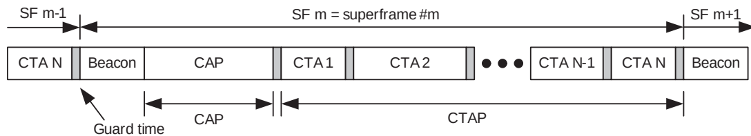
Figure 7-21—Superframe structure
