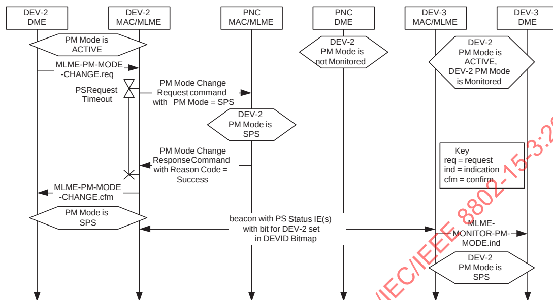
Figure 7-70—MSC showing DME initiated PM mode change from ACTIVE to an SPS mode
