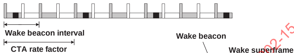
Case 3: Wake beacon interval = 2, CTA rate factor = 8
