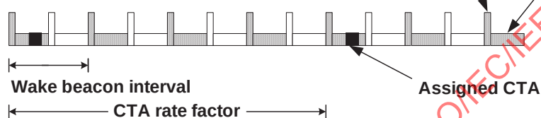
Case 4: Wake beacon interval = 4, CTA rate factor = 8
