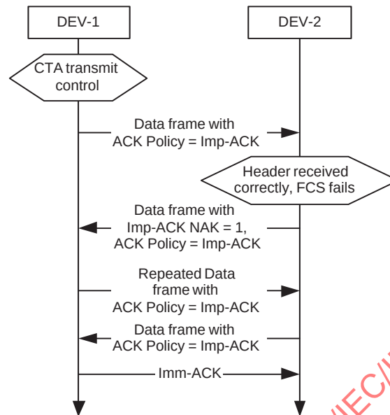
Figure 7-57—Example of the use of Imp-ACK where one of the frames fails FCS verification
