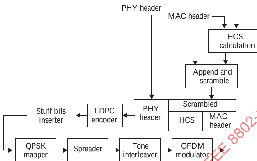
Figure 11-35—HSI main frame header encoding process
