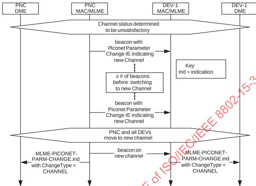
Figure 7-62—MSC for changing the piconet's channel
