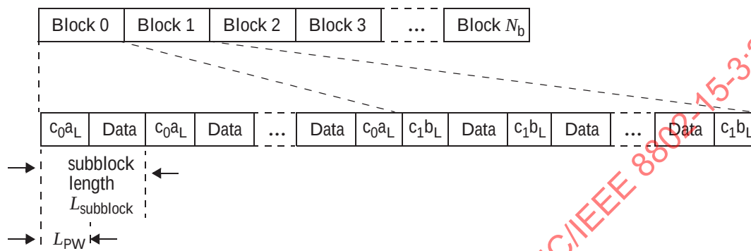
Figure 11-24—Frame format with pilot word
