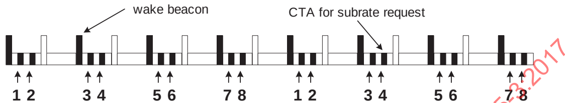
Figure 7-65—Minimum superframe loading of CTAs for 8 DEVs requesting wake beacon interval = 2 and CTA rate factor = 8
