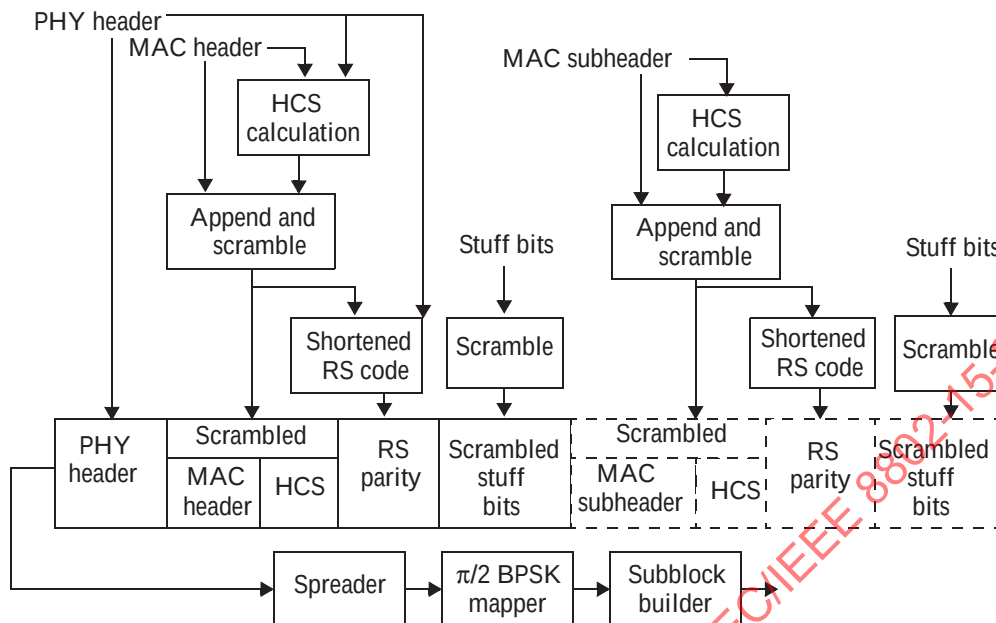
Figure 11-21—Frame header construction process
