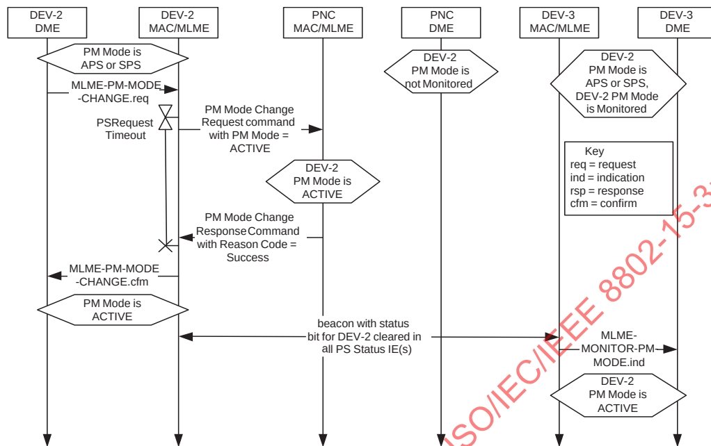
Figure 7-72—MSC showing DME initiated PM mode change from any PS mode to ACTIVE
