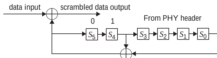
Figure 11-41—LRP scrambler reference implementation
