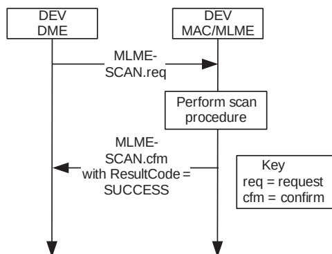
Figure 7-2—MSC for scan operation
