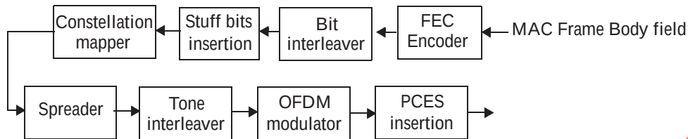
Figure 11-38—PHY Payload field construction process
