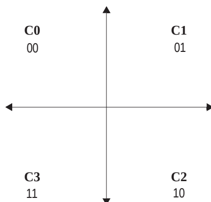
Figure 10-9—QPSK constellation bit mappings
