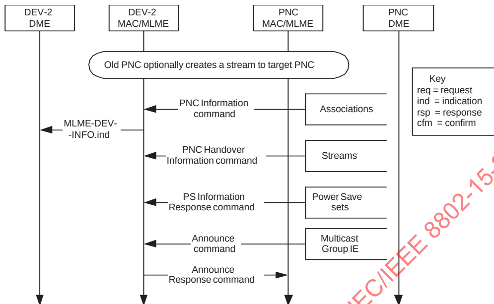
Figure 7-5—Handover information transfer MSC
