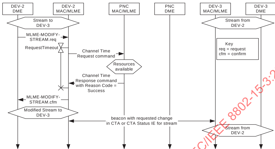
Figure 7-32—MSC for modifying a stream
