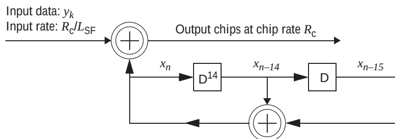
Figure 11-14—PRBS generation by LFSR
