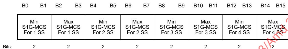
Figure 9-589cc—Basic S1G-MCS and NSS Set
