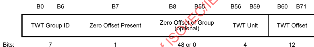
Figure 9-589ay—TWT Group Assignment field format
