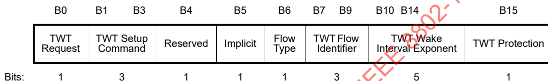
Figure 9-589ax—Request Type field format
