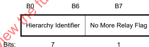
Figure 9-589bn—Relay Control field format
