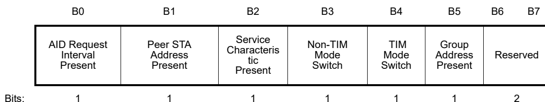
Figure 9-589an—AID Request Mode field format
