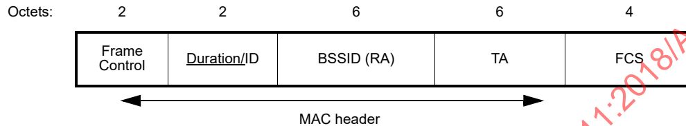
Figure 9-23—PS-Poll frame
