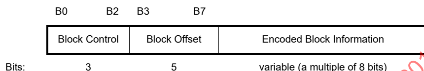
Figure 9-127e—Encoded Block subfield
