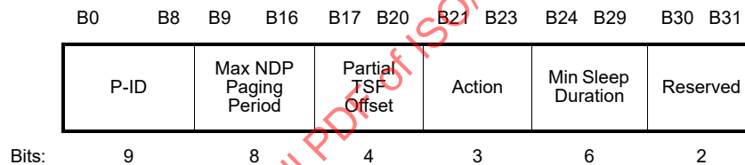
Figure 9-589az—NDP Paging field format
