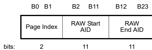
Figure 9-589ah—RAW Group subfield
