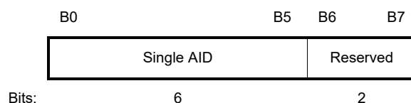
Figure 9-127h—Encoded Block Information (Single AID mode)
