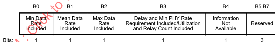
Figure 9-589bu—Relay Discovery Control field format
