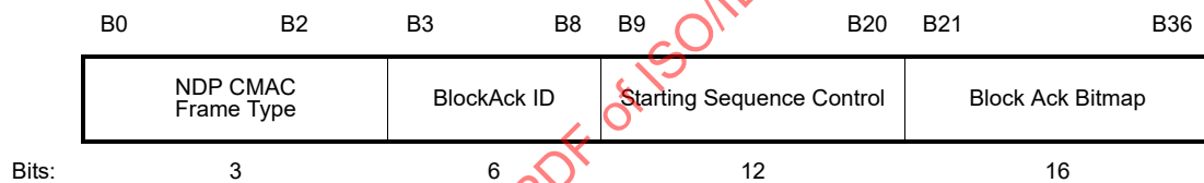
Figure 9-775—NDP CMAC frame body field of the NDP_2M BlockAck frame
