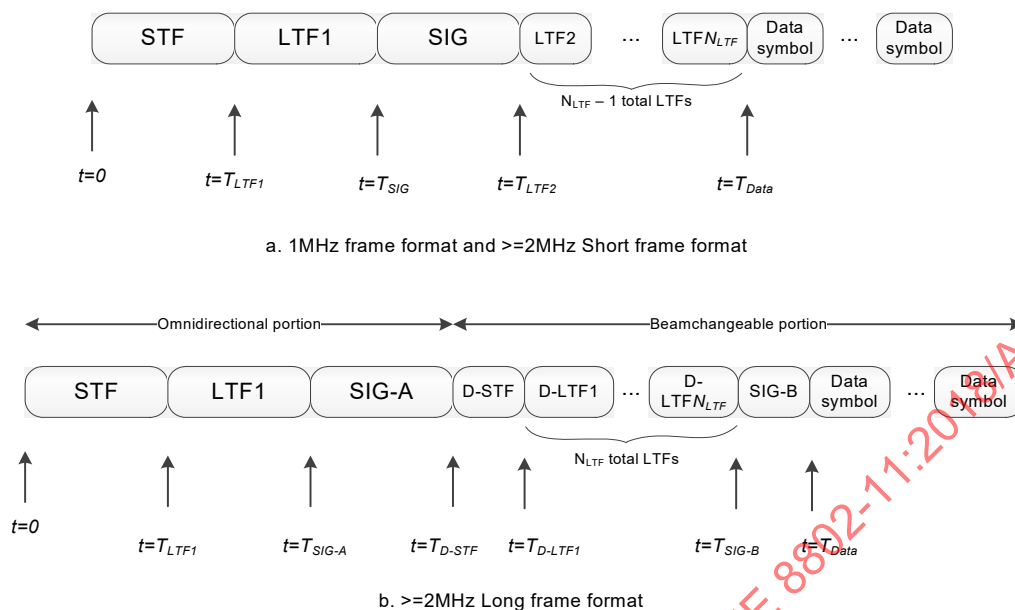
Figure 23-5—Timing boundaries for S1G PPDU fields
