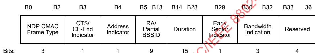
Figure 9-765—NDP CMAC frame body field of the NDP_2M CTS frame
