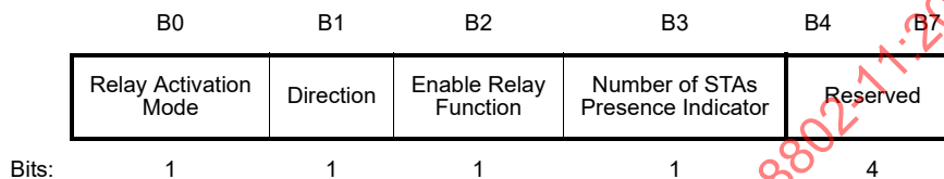
Figure 9-589br—Relay Function field format
