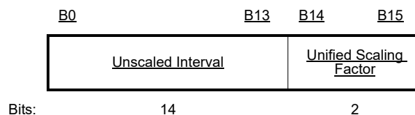
Figure 9-71a—Listen Interval field carried in an S1G PPDU
