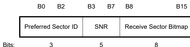
Figure 9-740c—Sector ID Index format
