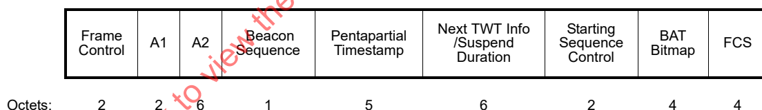
Figure 9-753—BAT frame format
