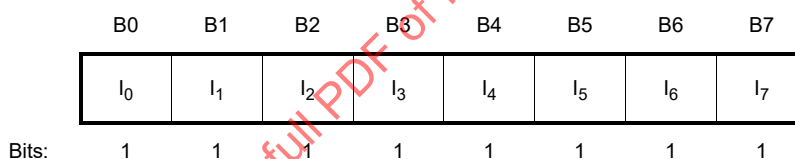
Figure 9-740d—Receive Sector Bitmap format
