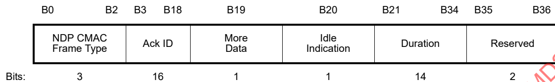
Figure 9-773—NDP CMAC frame body field of the NDP_2M PS-Poll-Ack frame
