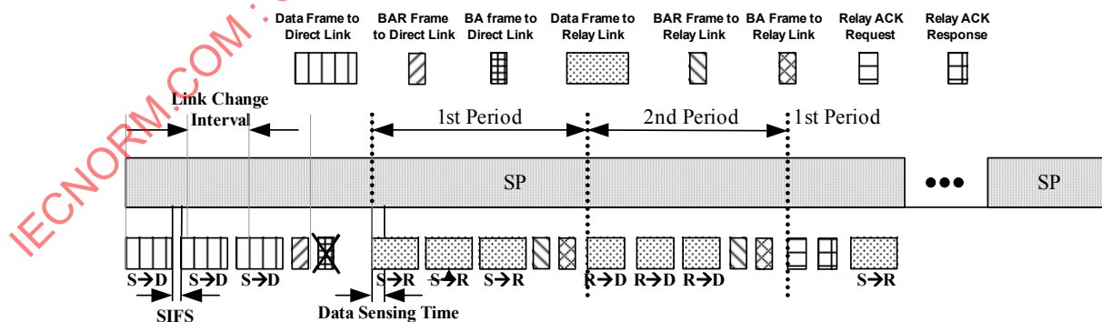
Figure 9-78—Example of the operation with HD-DF relay
