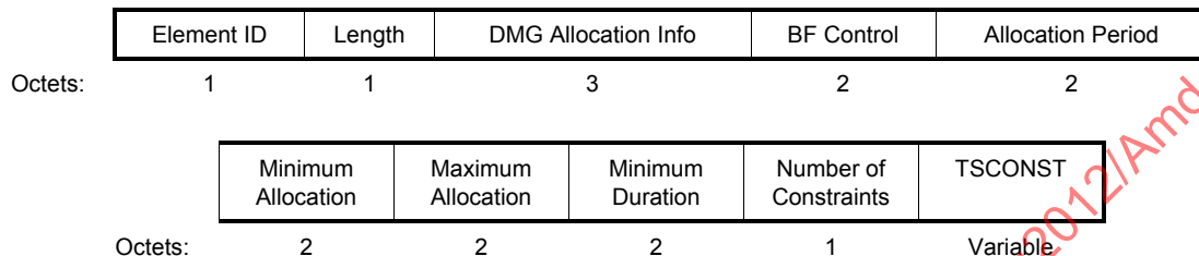
Figure 8-401ae—DMG TSPEC element format
