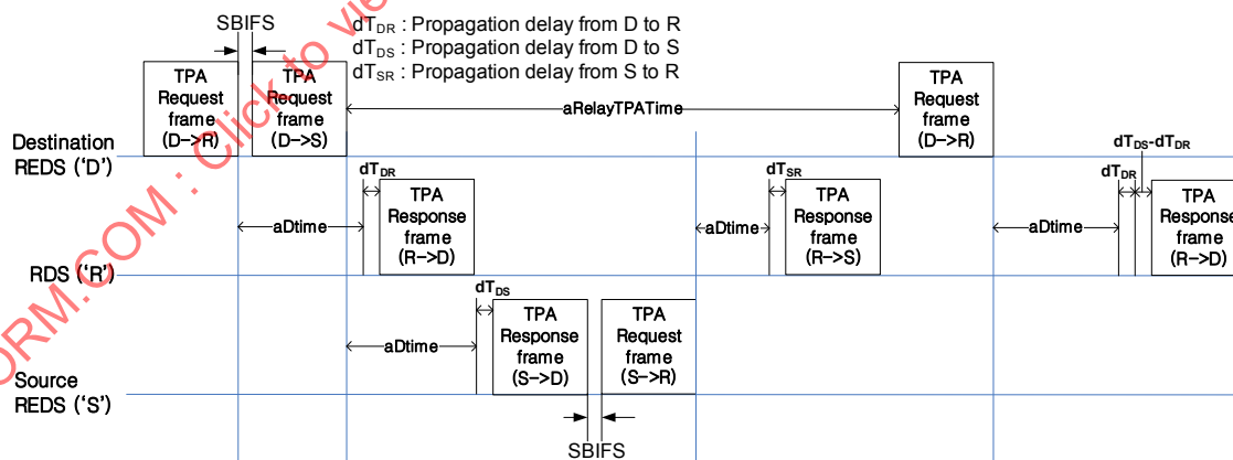
Figure 9-79—TPA mechanism
