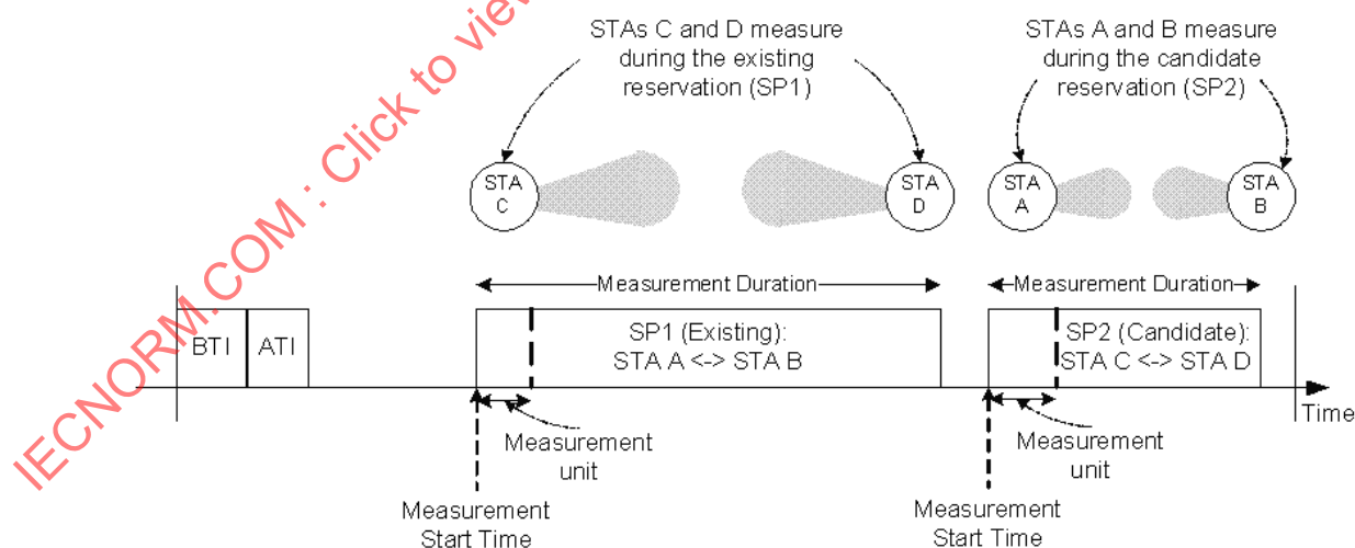
Figure 10-31—Example of spatial sharing assessment
