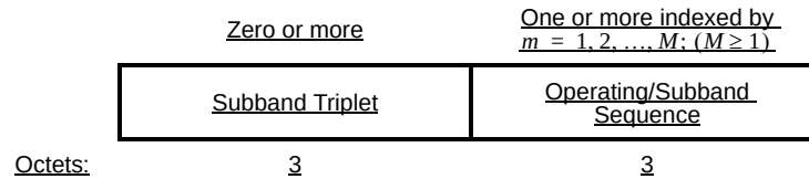
Figure 8-90c—Triplet field if dot11OperatatingClassRequired is true
