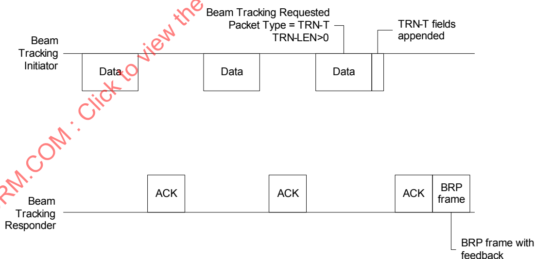
Figure 9-71—Example of a beam tracking procedure with the initiator requesting TRN-T
