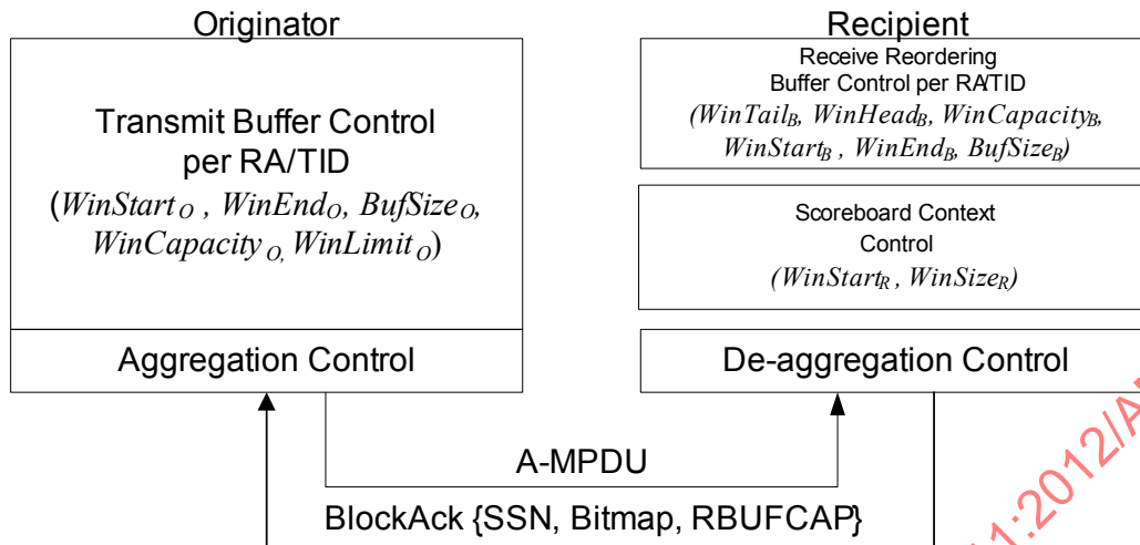
Figure 9-74—DMG Block Ack architecture
