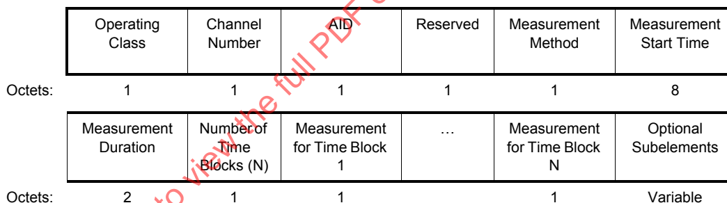
Figure 8-182a—Measurement report field format for directional channel quality report
