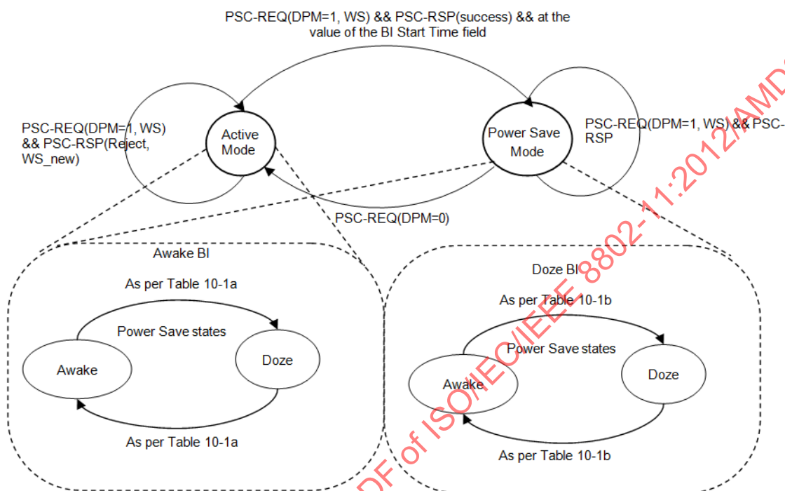
Figure 10-5a—State transition diagram of non-PCP/non-AP STA in Active and Power Save Mode
