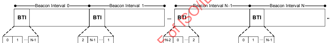
Figure 10-1a—Example of DMG Beacon transmission by PCP/AP during the BTI
