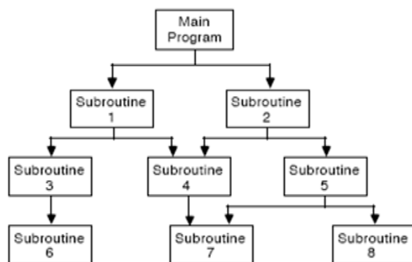
Figure 5 — Call graph
