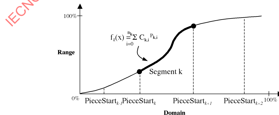
Figure B.3—Calibration curve properties
