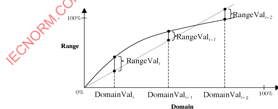
Figure B.2—Calibration table properties
