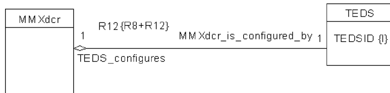
Figure 24— IEEE1451_Dot4TEDS association for IEEE1451_Dot4MMXdcr
