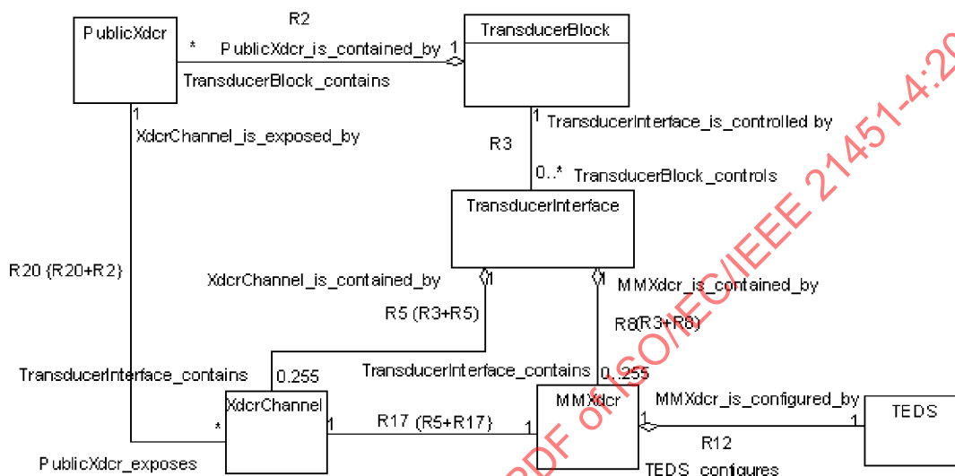
Figure 20—TBOM class diagram
