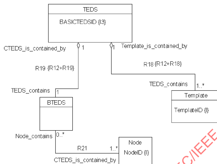
Figure 26—TEDS structural class diagram
