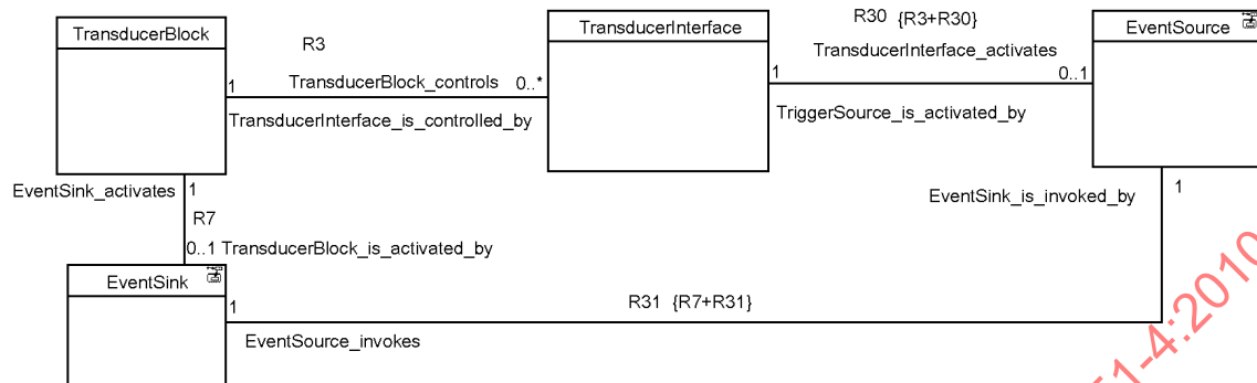
Figure 34—IEEE1451_Dot4EventSink associations
