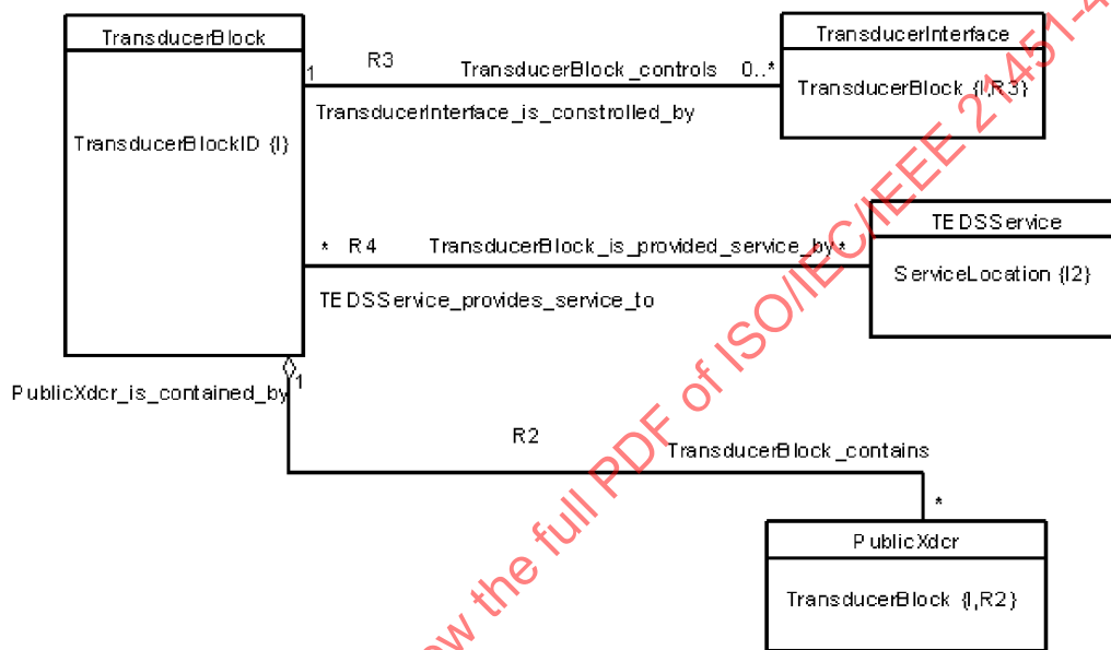
Figure 21—IEEE1451_Dot4TransducerBlock associations
