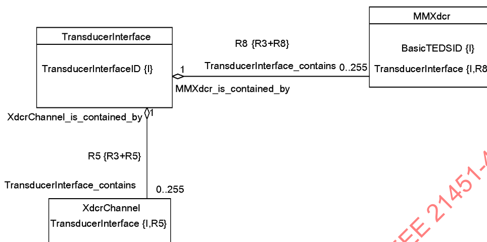
Figure 22—IEEE1451_Dot4TransducerInterface associations
