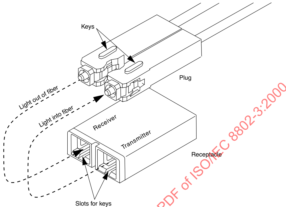
Figure 38–8—Duplex SC connector and receptacle (informative)
