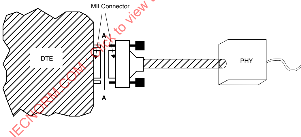
Figure 22–2—Example application showing location of conformance test
