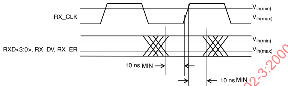
Figure 22–15—Receive signal timing relationships at the MII
