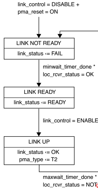
Figure 32-16—Link Monitor state diagram
