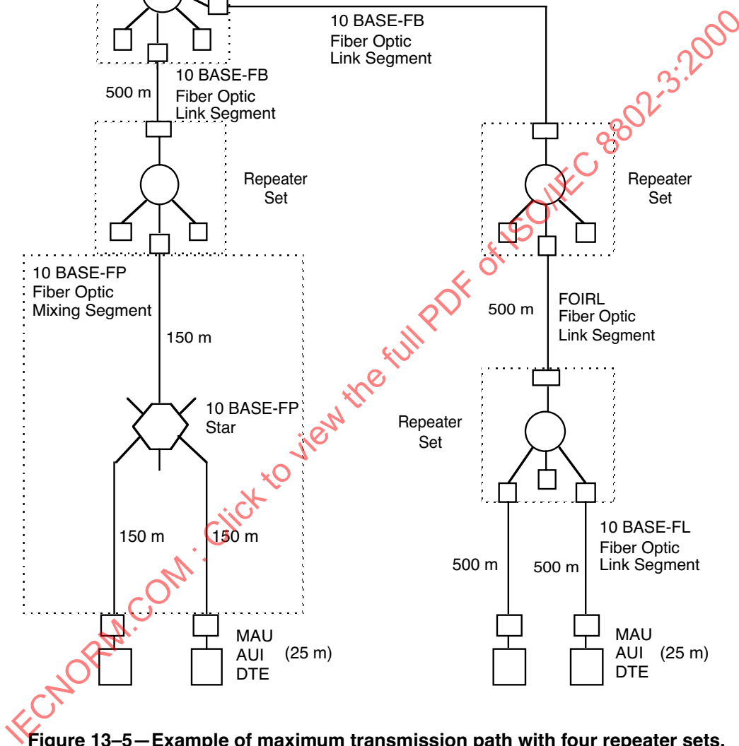
Figure 13-5—Example of maximum transmission path with four repeater sets, five segments (two 500 m 10BASE-FB, one 500 m FOIRL, one 500 m 10BASE-FL, and one 300 m 10BASE-FP)
