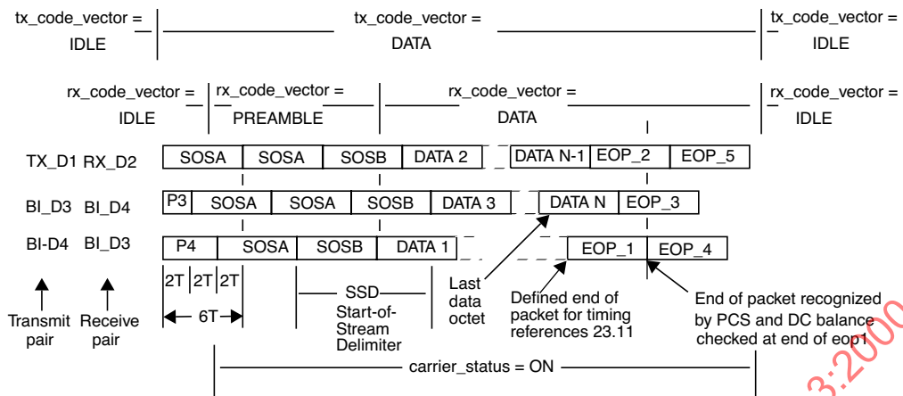
Figure 23-6—PCS sublayer to PMA sublayer frame structure
