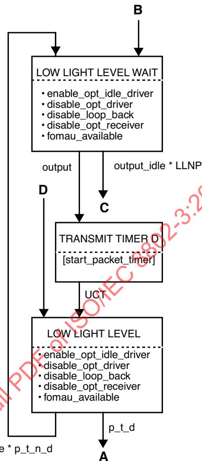
Figure 9-10— Low Light Level Detection function state diagram
