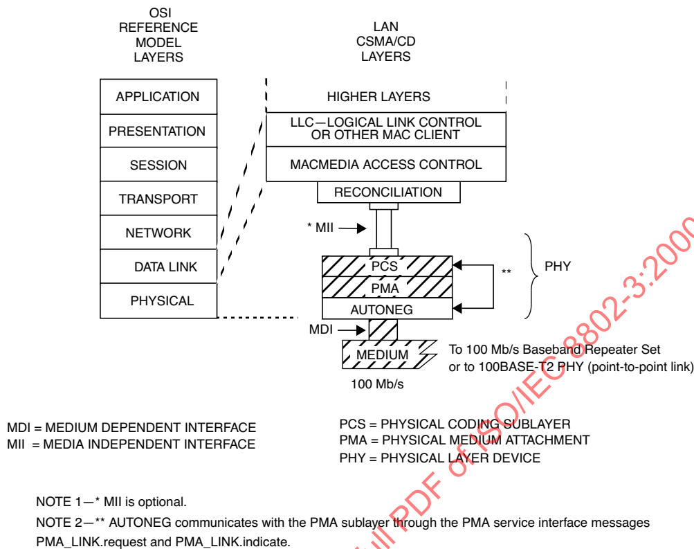
Figure 32–1 —Type 100BASE-T2 PHY relationship to the ISO/IEC Open Systems Interconnection (OSI) reference model and the IEEE 802.3 CSMA/CD LAN model
