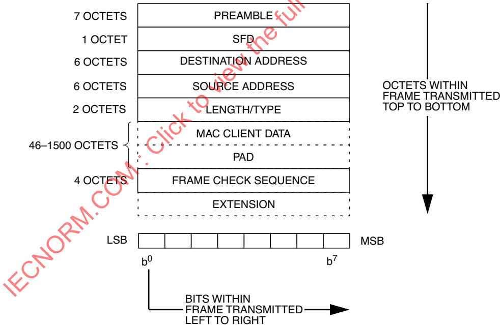
Figure 3–1 — MAC frame format
