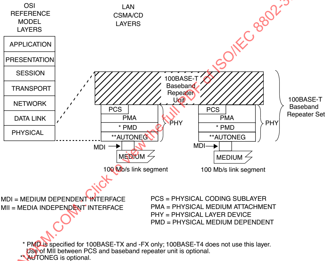
Figure 27–1 — 100BASE-T repeater set relationship to the ISO/IEC OSI reference model
