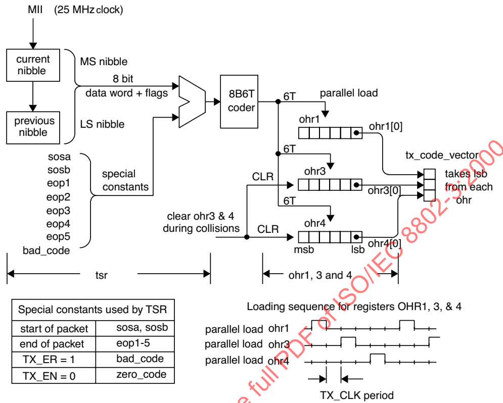
Figure 23-7—PCS Transmit reference diagram
