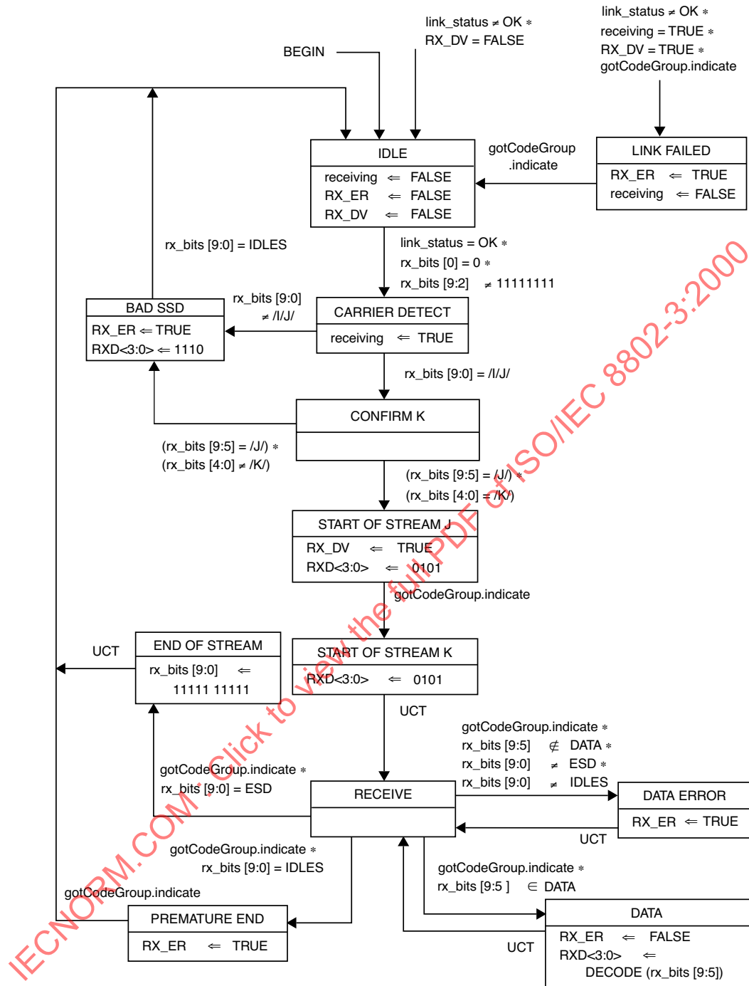
Figure 24–11 – Receive state diagram
