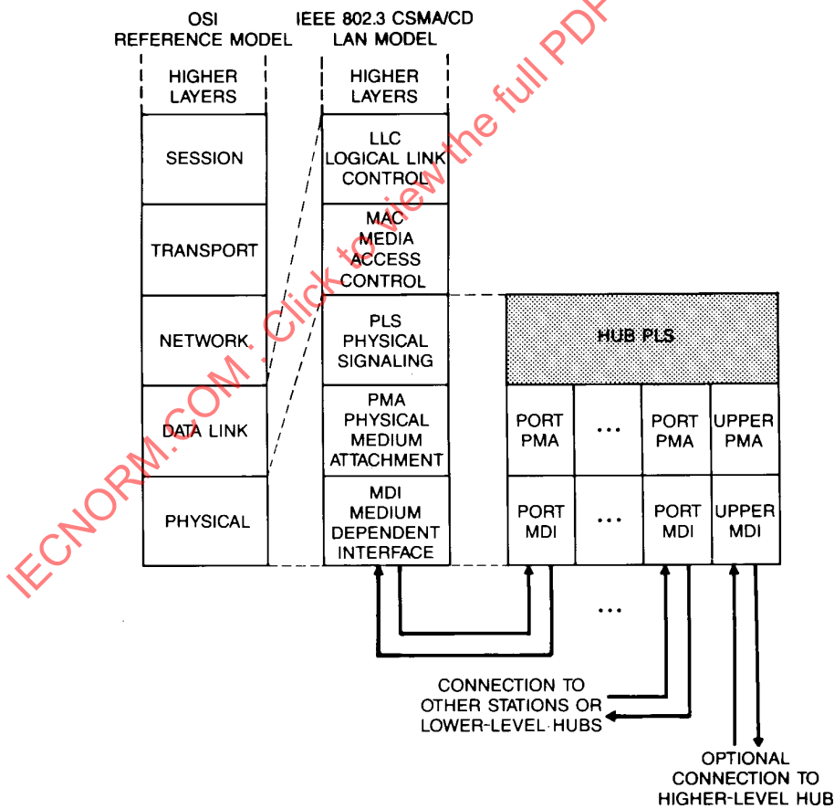
Figure 12-12—Hub relationship to the OSI reference model and the IEEE 802.3 CSMA/CD LAN model
