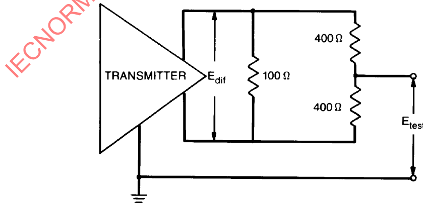
Figure 12–24—Transmitter impedance balance
