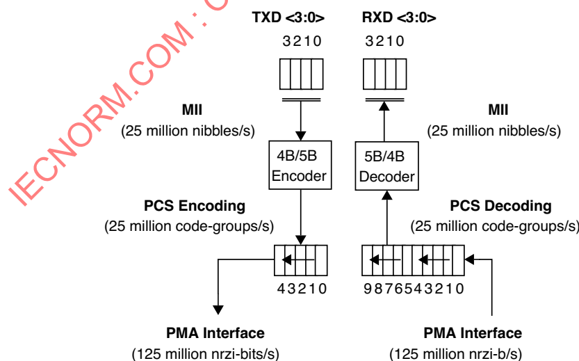
Figure 24–6—PCS reference diagram
