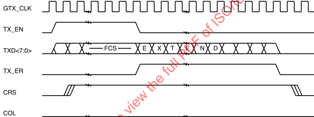
Figure 35-6—Transmission with carrier extension
