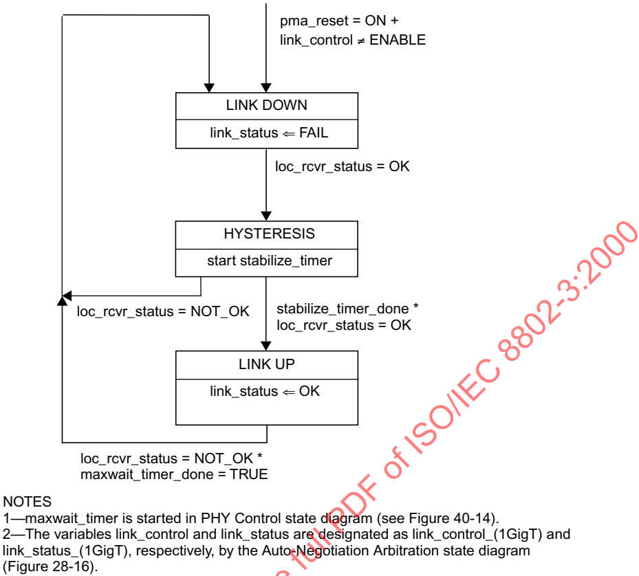
Figure 40–16—Link Monitor state diagram
