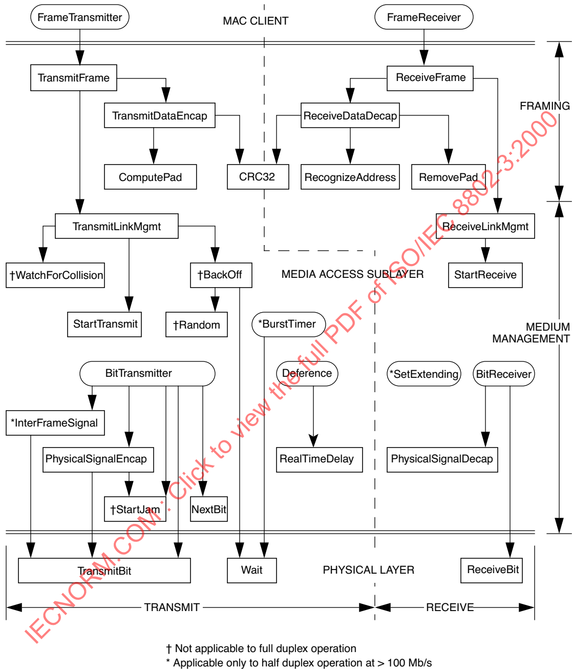
Figure 4–3—Relationship among CSMA/CD procedures
