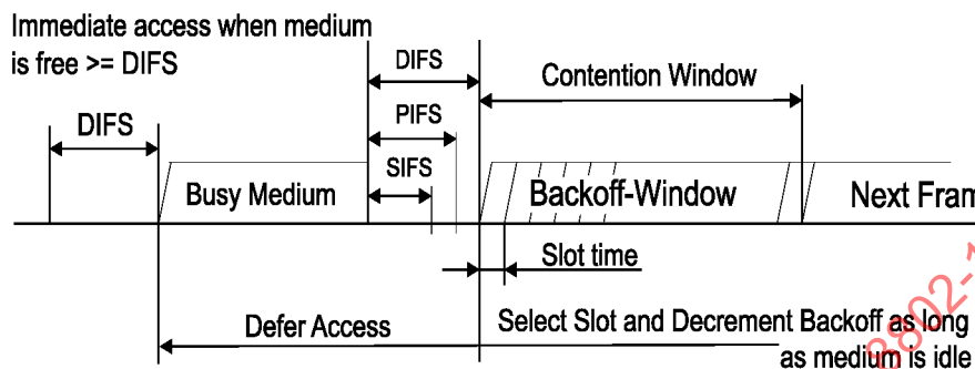
Figure 55—Basic access method
