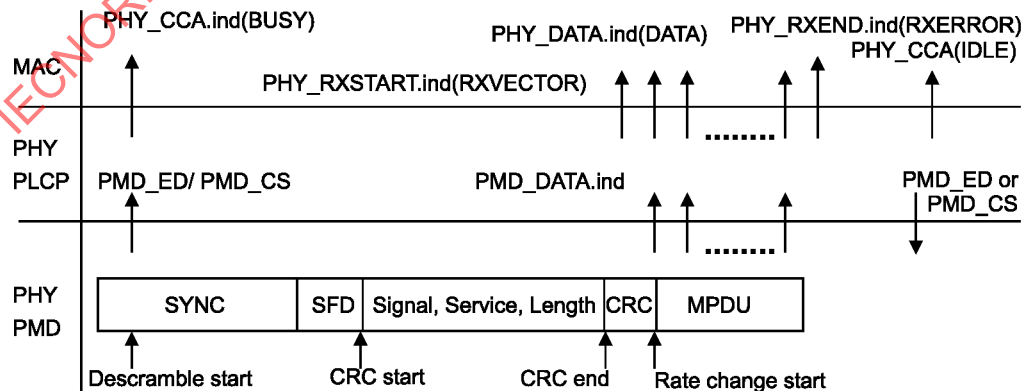
Figure 97—Receive PLCP
