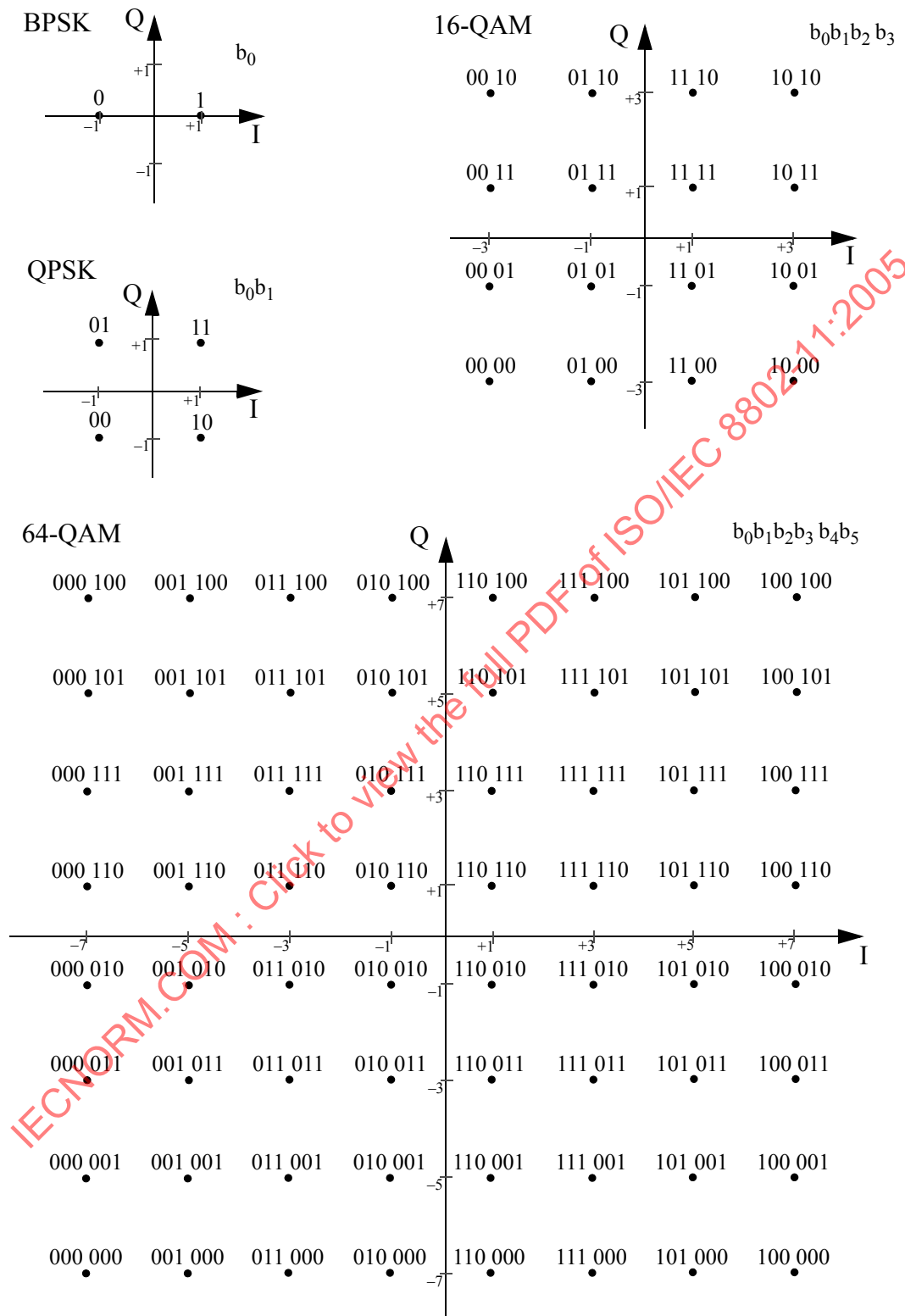
Figure 120—BPSK, QPSK, 16-QAM, and 64-QAM constellation bit encoding
