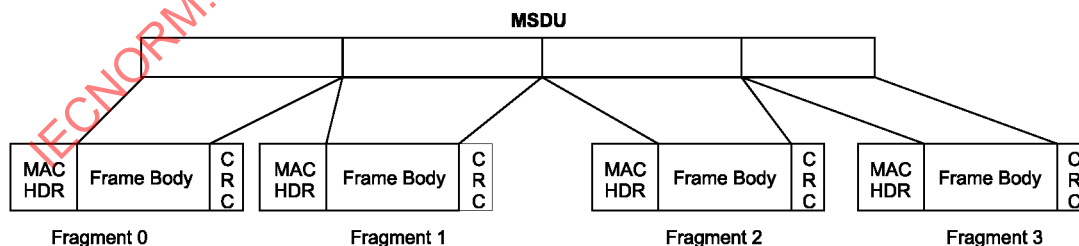
Figure 52—Fragmentation
