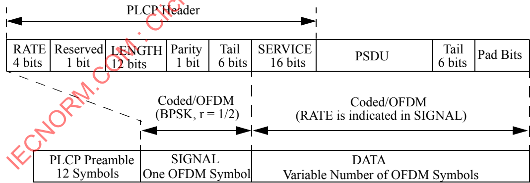
Figure 111—PPDU frame format
