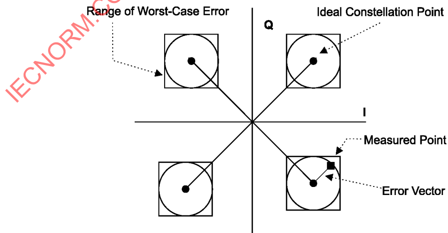
Figure 103—Modulation accuracy measurement example
