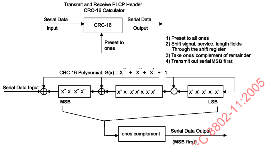
Figure 91—CRC-16 implementation
