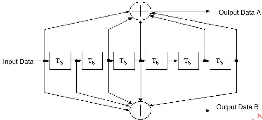
Figure 118—Convolutional encoder ( k = 7 )
