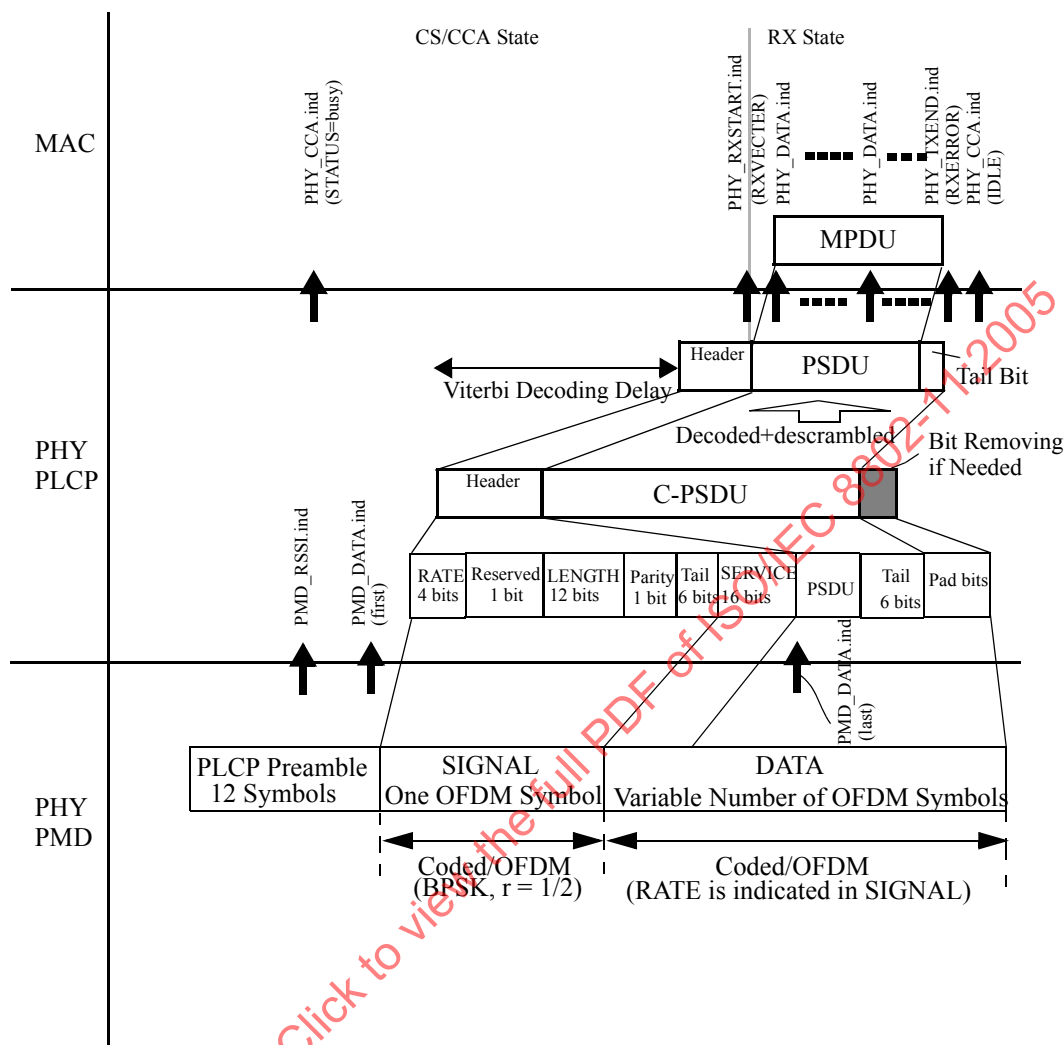
Figure 128—Receive PLCP
