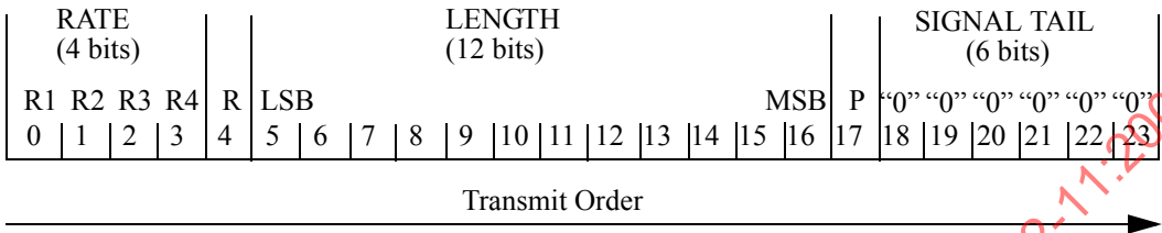
Figure 115—SIGNAL field bit assignment
