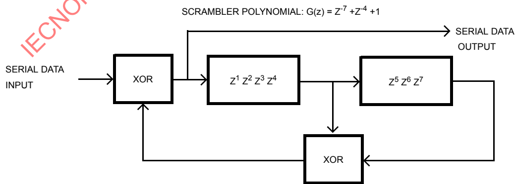
Figure 135—Data scrambler
