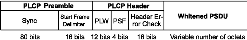
Figure 74—PLCP frame format
