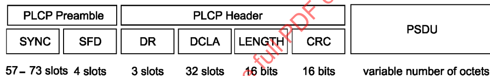
Figure 105—PPDU frame format
