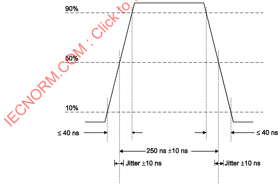
Figure 106—Basic pulse shape
