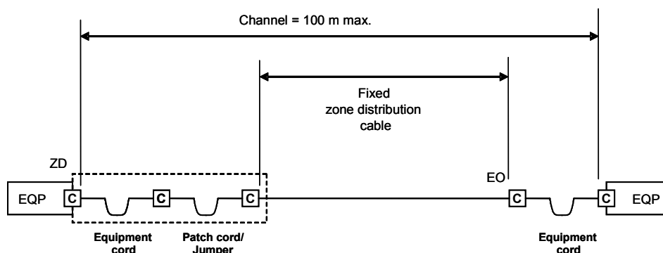
Figure 10b – Cross-connect – EO model
