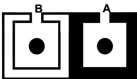
Figure 14a – IEC 61754-20 interface for one or two optical fibres
