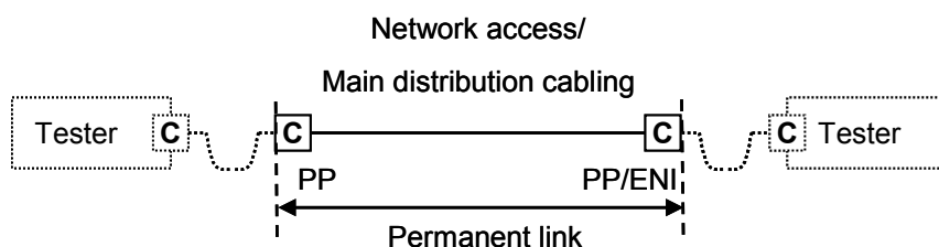
Figure A.1a – Configuration PL1
