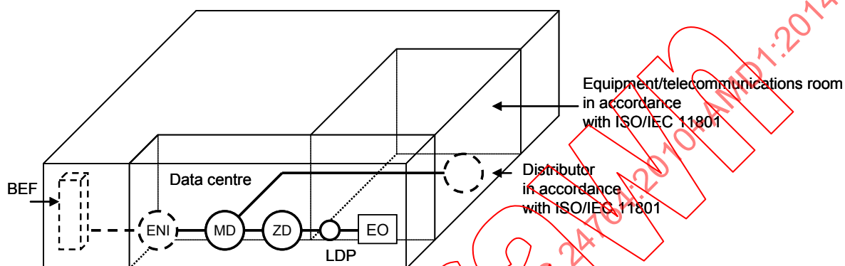
Figure 4 – Example of accommodation of functional elements
