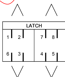
Figure 13b – IEC 60603-7 series interface for Category 7 and 7 A
