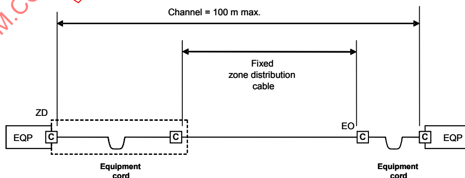
Figure 10a – Interconnect – EO model
