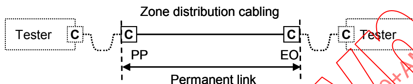
Figure A.1b – Configuration PL2
