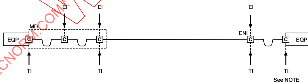
Figure 5c – Network access cabling from MD to distributor in accordance with ISO/IEC 11801
