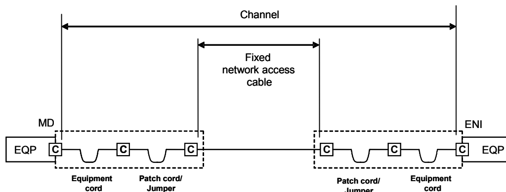
Figure 12a – Network access cabling from MD to ENI
