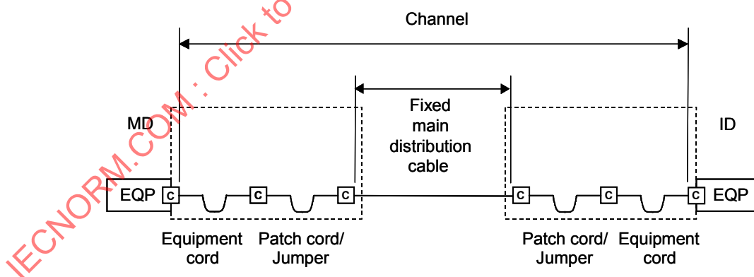
Figure C.4 – Main distribution cabling models
