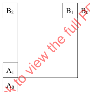
Figure 10 — Spatial motion vector neighbours
