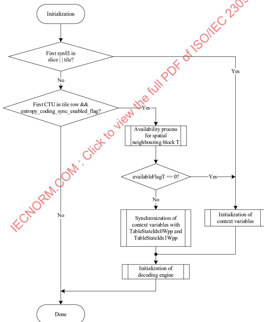
Figure 13 — Flowchart of CABAC initialization process
