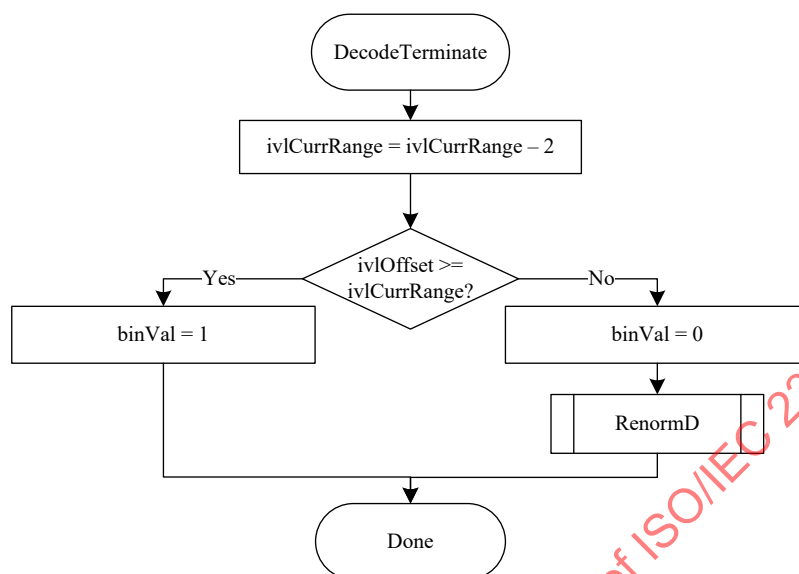
Figure 9-9 — Flowchart of decoding a decision before termination
