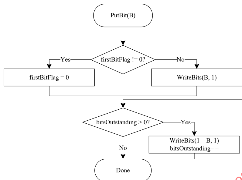
Figure 9-12 — Flowchart of PutBit(B)
