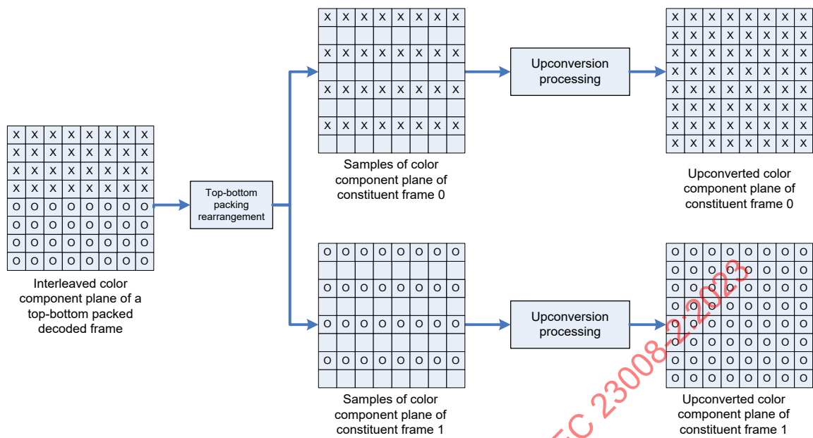
Figure D.6 — Rearrangement and upconversion of top-bottom packing arrangement with frame_packing_arrangement_type equal to 4, quincunx_sampling_flag equal to 0, and (x, y) equal to (0, 0) or (8, 4) for both constituent frames
