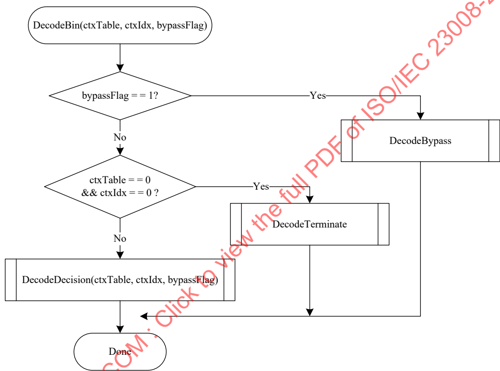
Figure 9-5 — Overview of the arithmetic decoding process for a single bin
