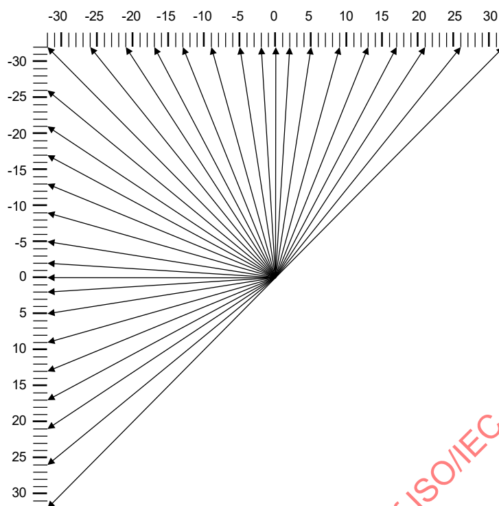
Figure 8-2 — Intra prediction angle definition
