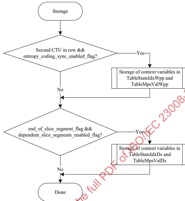
Figure 9-4 — Illustration of CABAC storage process
