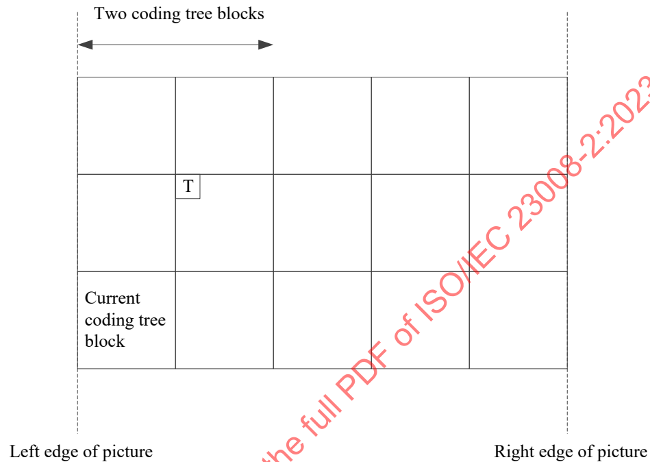
Figure 9-2 — Spatial neighbour T that is used to invoke the CTB availability derivation process relative to the current CTB
