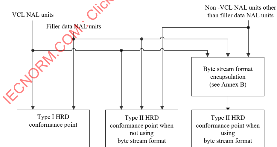
Figure C.1 — Structure of byte streams and NAL unit streams for HRD conformance checks
