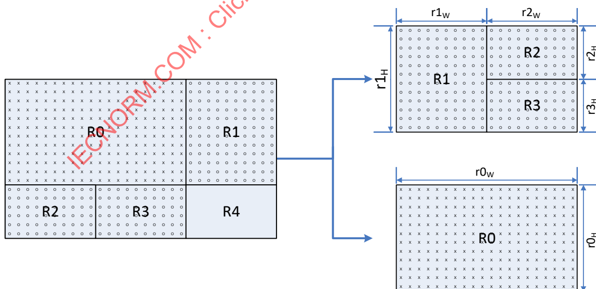
Figure D.10 — Rearrangement of a segmented rectangular frame packing arrangement
