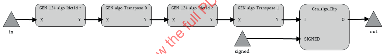
Figure B.1 — Example of networks of FU expressed using RVC FNL
