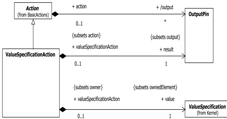
Figure 11.11 - Miscellaneous actions
