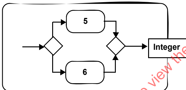
Figure 12.136 - Example ValueSpecificationAction
