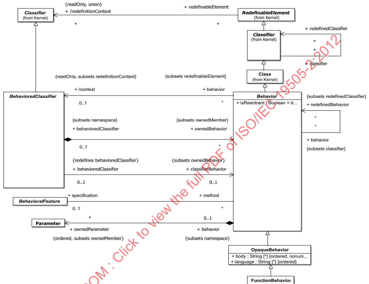
Figure 13.6 - Common Behavior
