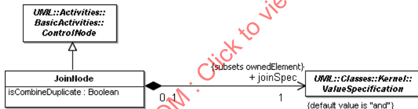
Figure 12.19 - Control nodes (CompleteActivities)
