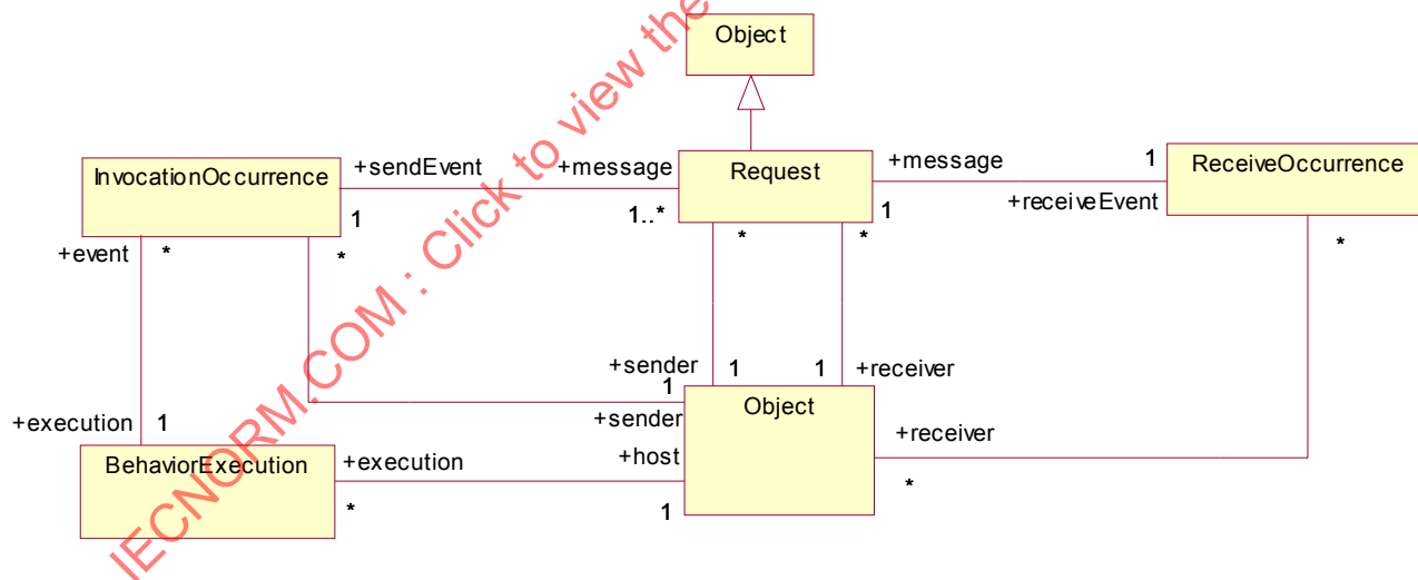
Figure 13.3 - Communication Domain Model
