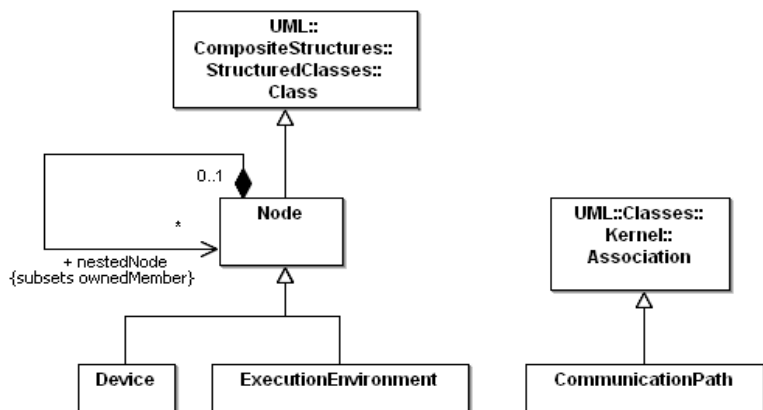
Figure 10.3 - The definition of the Node concept
