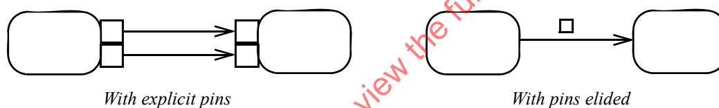
Figure 12.109 - Eliding objects flowing on the edge
