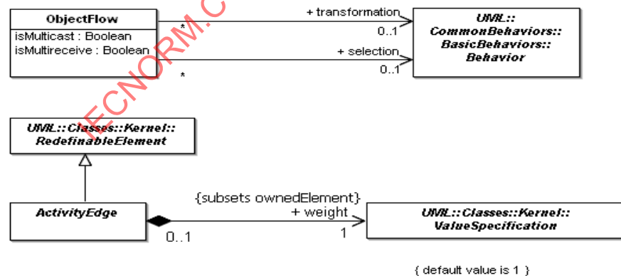
Figure 12.14 - Flows (CompleteActivities)
