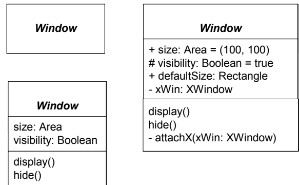
Figure 7.28 - Class notation: details suppressed, analysis-level details, implementation-level details
