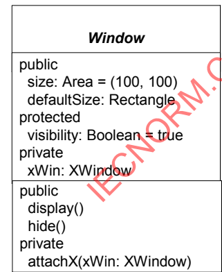
Figure 7.29 - Class notation: attributes and operations grouped according to visibility
