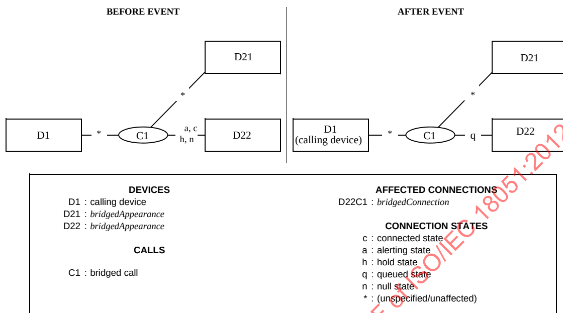
Figure 17-32 Bridged Event
