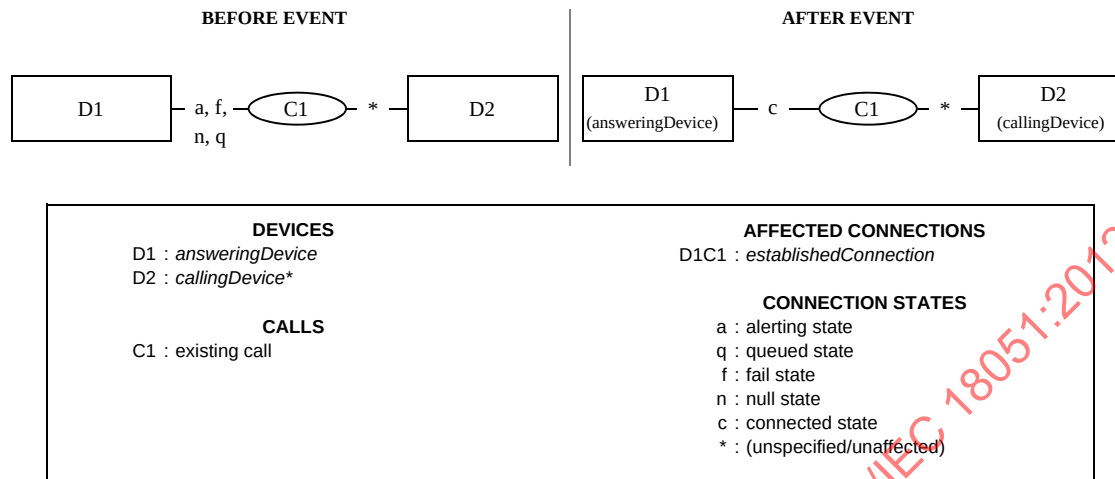
Figure 17-42 Established Event
