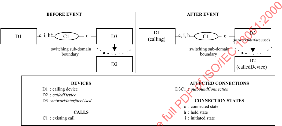
Figure 17-42 Network Capabilities Changed Event
