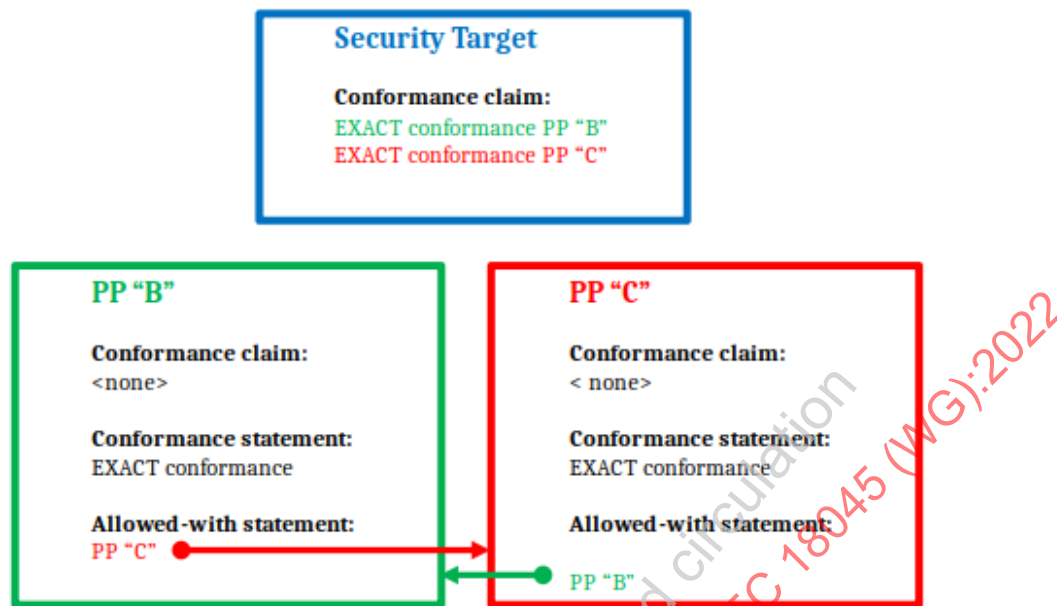
Figure 8 — Example of exact conformance relationships between an ST and PPs
