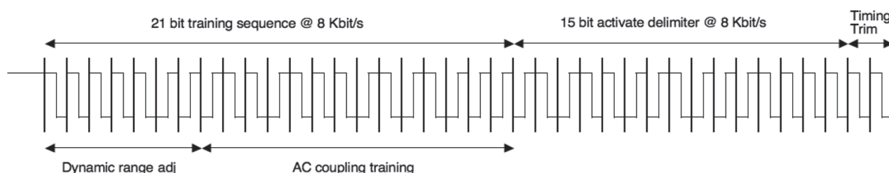
Figure 7.32 — Activation preamble
