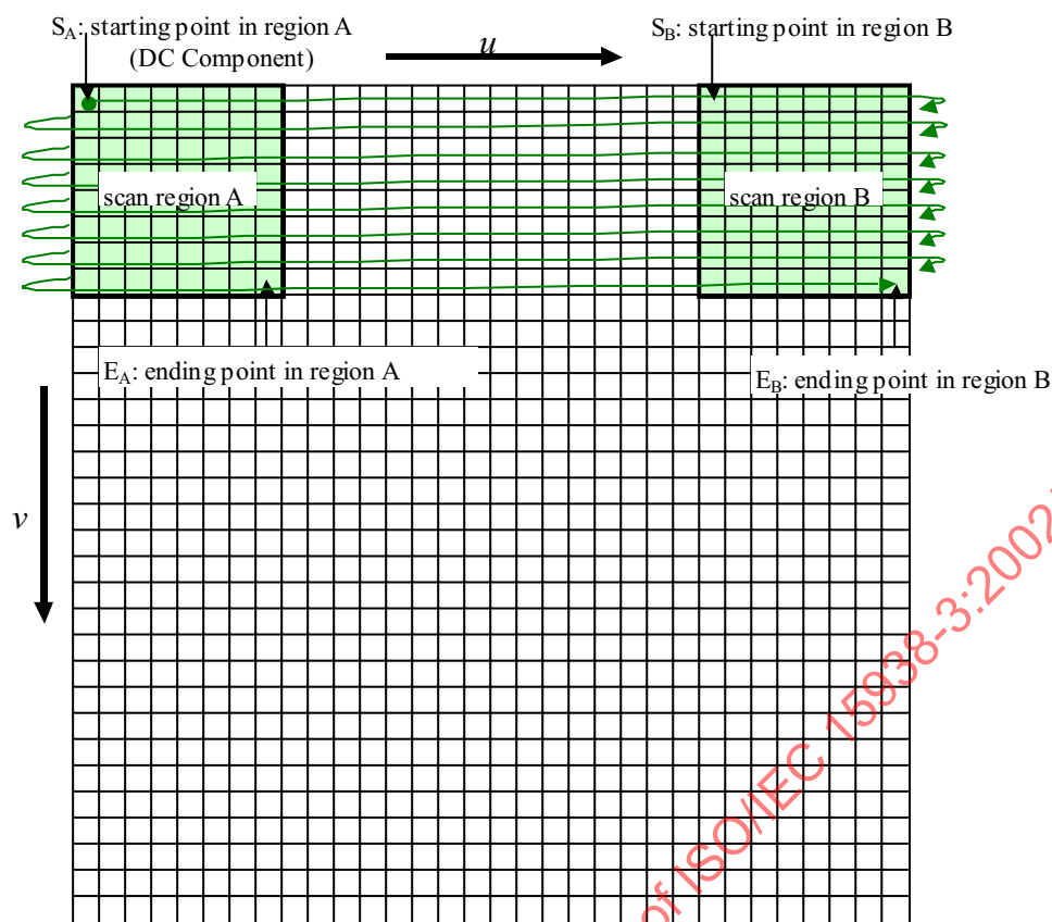
Figure Amd1-2 - Definition of scanning in the Fourier domain.
