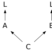
Figure 3 — Non-virtual base
