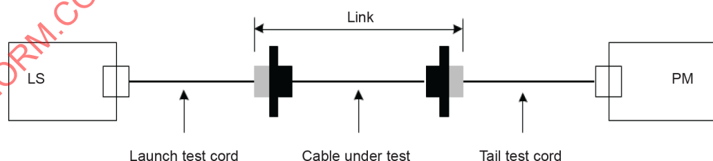
Figure E.2 – Connections to link for attenuation measurement
