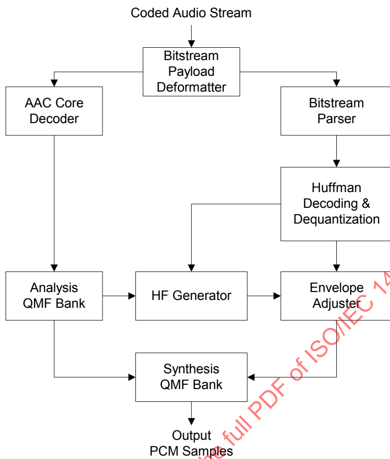
Figure 4.46 – Decoder block diagram
