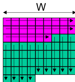
Figure 1.14 – Interleave matrix in non-rectangular case
