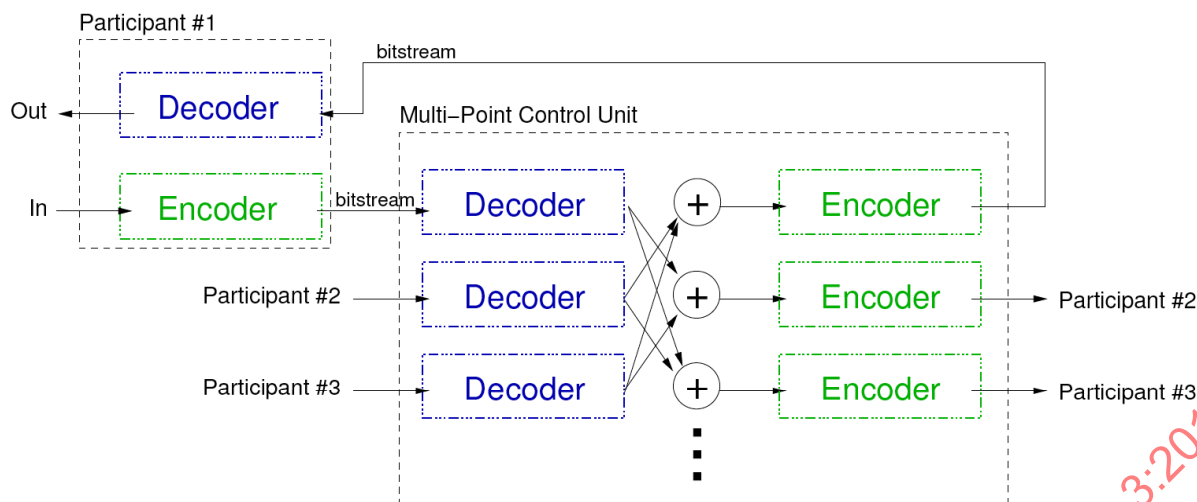
Figure 4.B.17 – Mixing of bitstreams in an MCU
