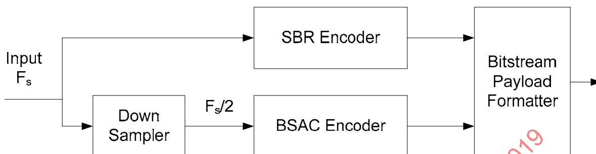
Figure 4.B.13 – Overview of the integration of ER BSAC and SBR Encoder
