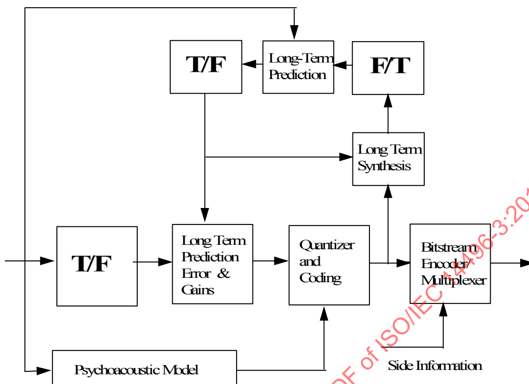
Figure 4.B.1 – Block diagram of the encoding process of Long Term Prediction
