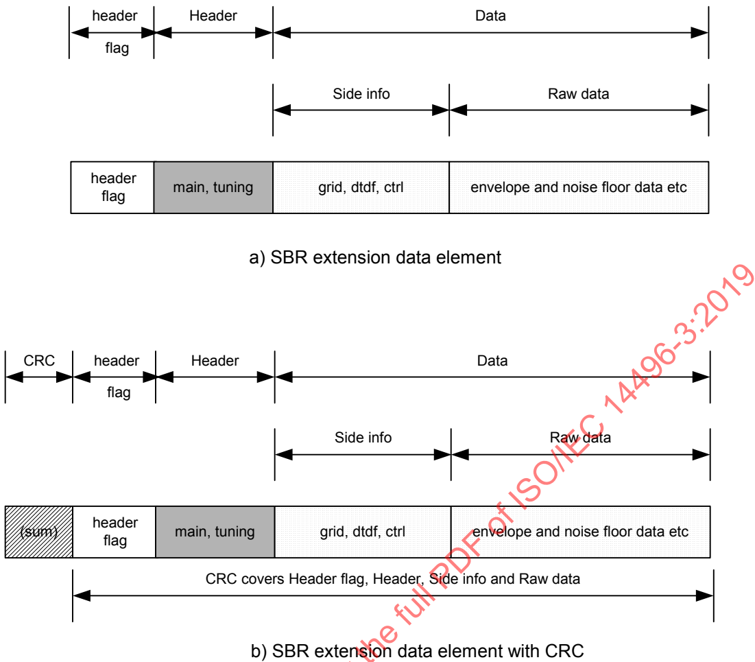
Figure 4.21 – The basic sections of the SBR extension data elements
