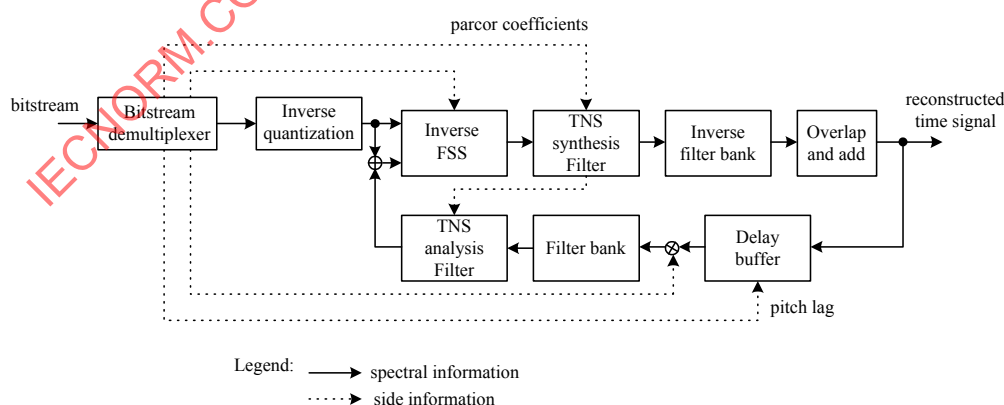
Figure 4.37 – Decoder structure
