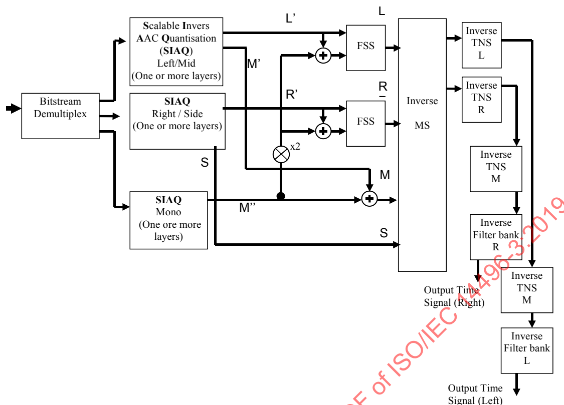
Figure 4.4 – AAC mono / AAC stereo configuration (AAC-Only-M/S)
