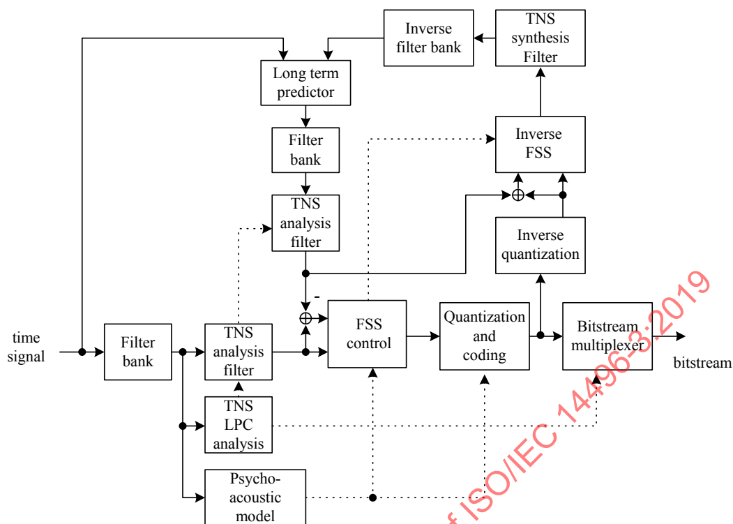
Figure 4.38 – Encoder structure
