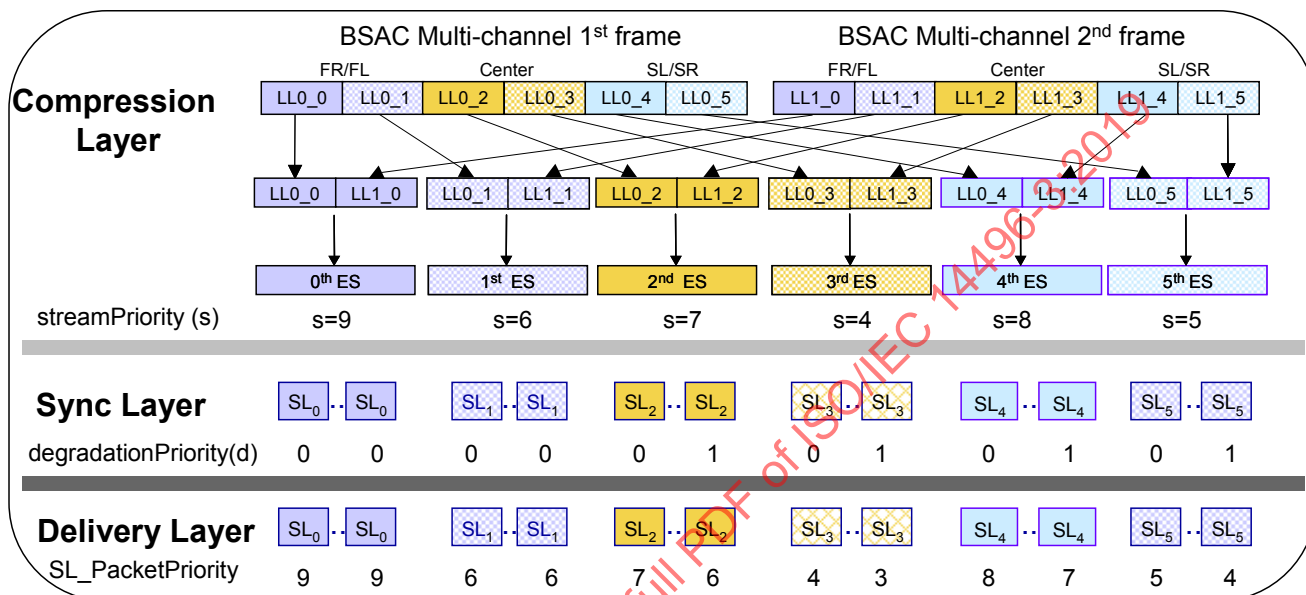
Figure 4.B.10 – Scalable transmission of BSAC multichannel payload
