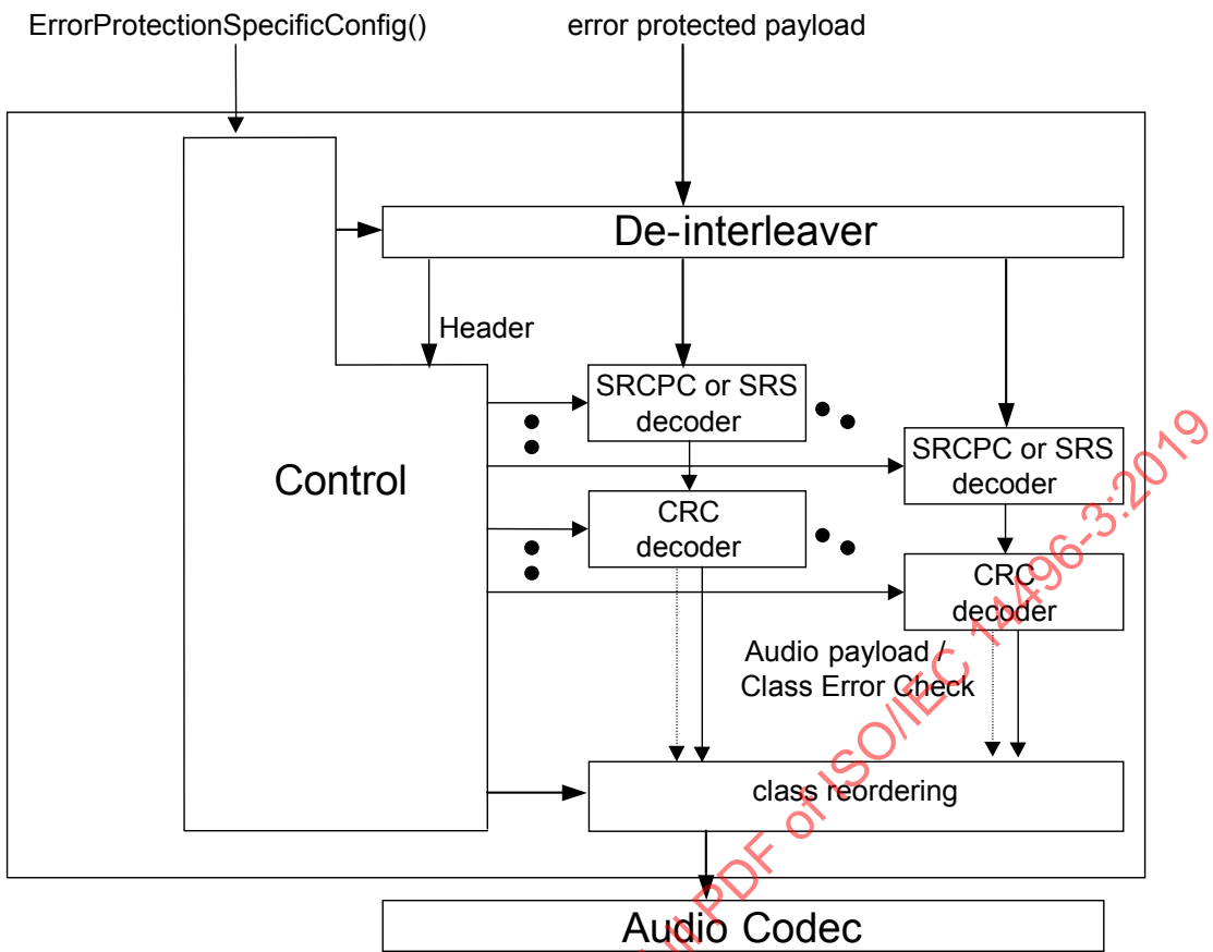
Figure 1.8 – Outline of EP decoder
