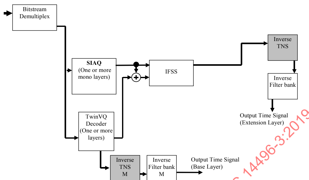
Figure 4.9 – Decoding of a TwinVQ (mono) + AAC (mono) configuration, TwinVQ does use TNS
