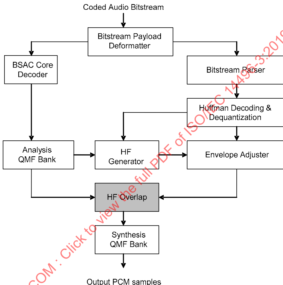
Figure 4.130 – Overview of the integration of ER BSAC and SBR decoder
