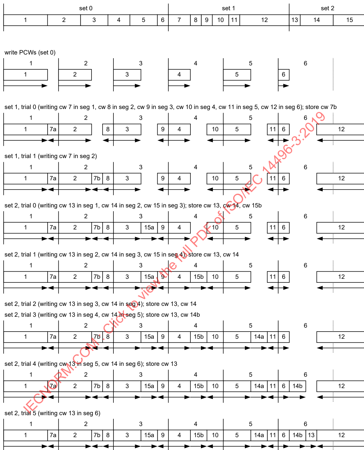
Figure 4.36 – Example for HCR encoding algorithm (only one segment width, pre-sorting has been done before)
