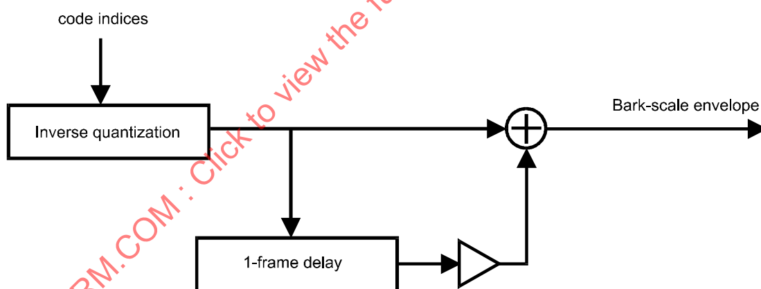
Figure 4.32 – Decoding process of the TwinVQ
