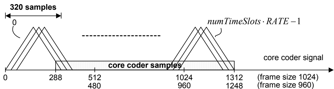
(a) core coder signal QMF analysis windowing
