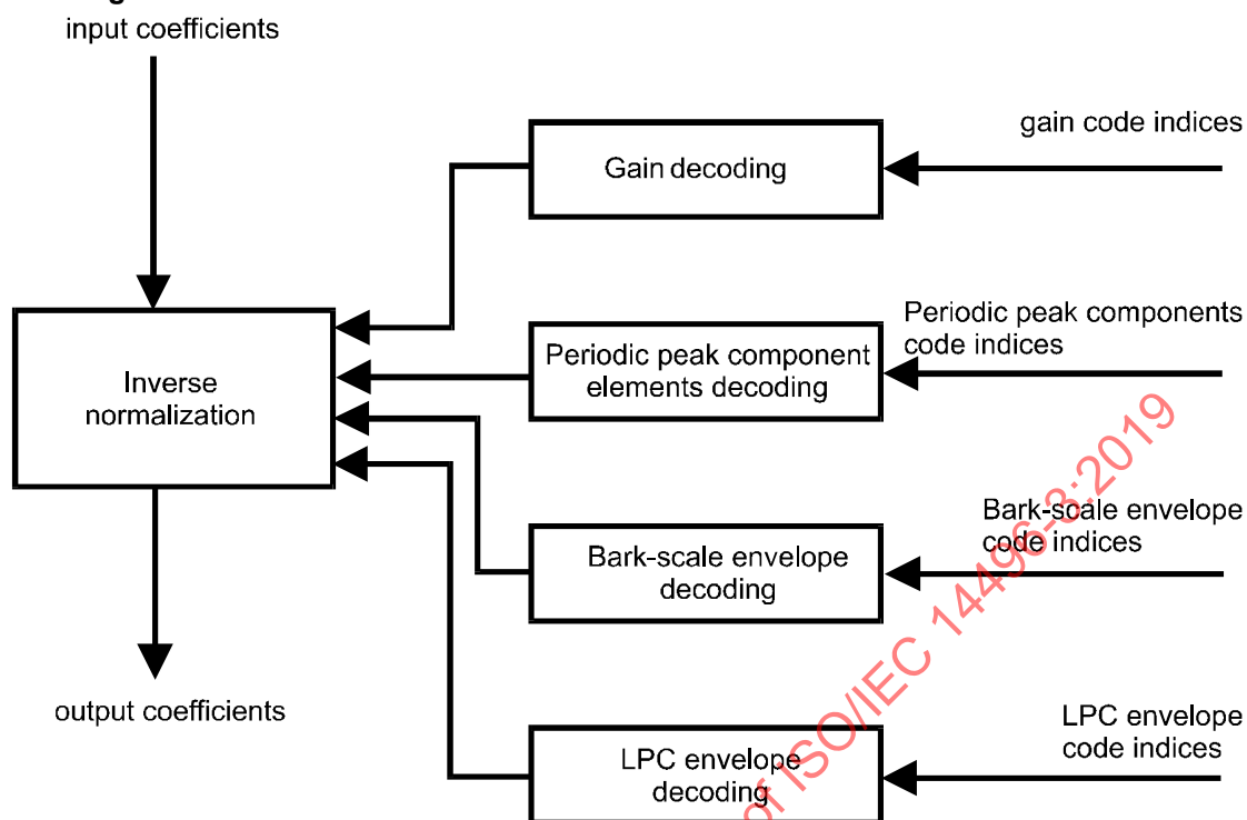
Figure 4.32 – Decoding process of the TwinVQ
