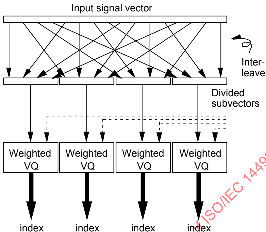
Figure 4.B.2 – Weighted interleave vector quantization.
