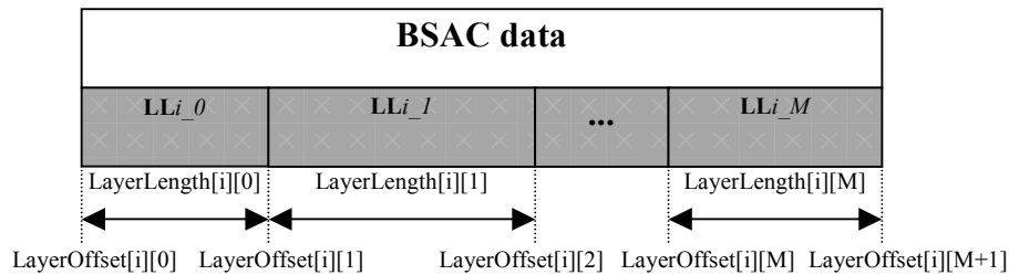
Figure 4.B.9 – The structure of the BSAC data
