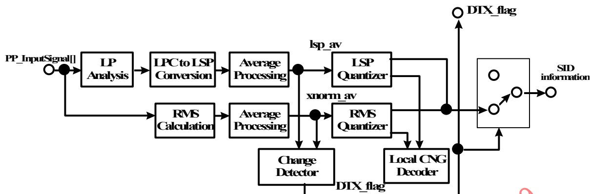
Figure 3.B.2 — DTX module
