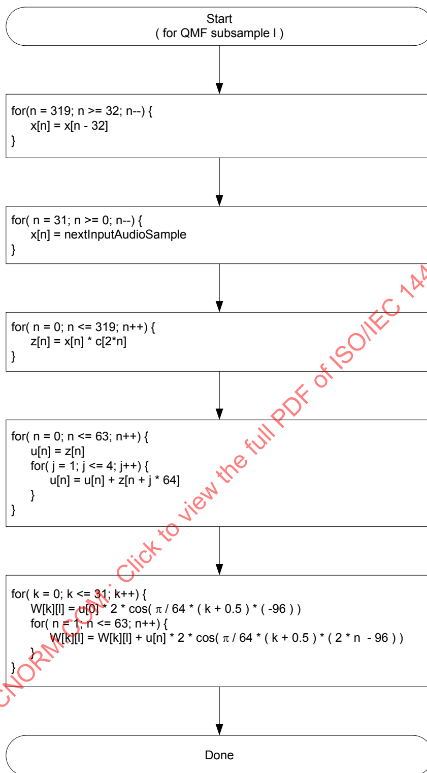
Figure 4.50 – Flowchart of decoder real-valued analysis QMF bank
