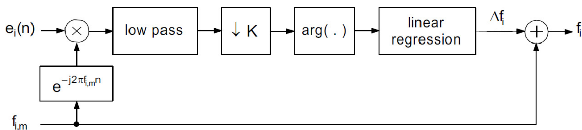
Figure 7.A.4 — High accuracy frequency estimation
