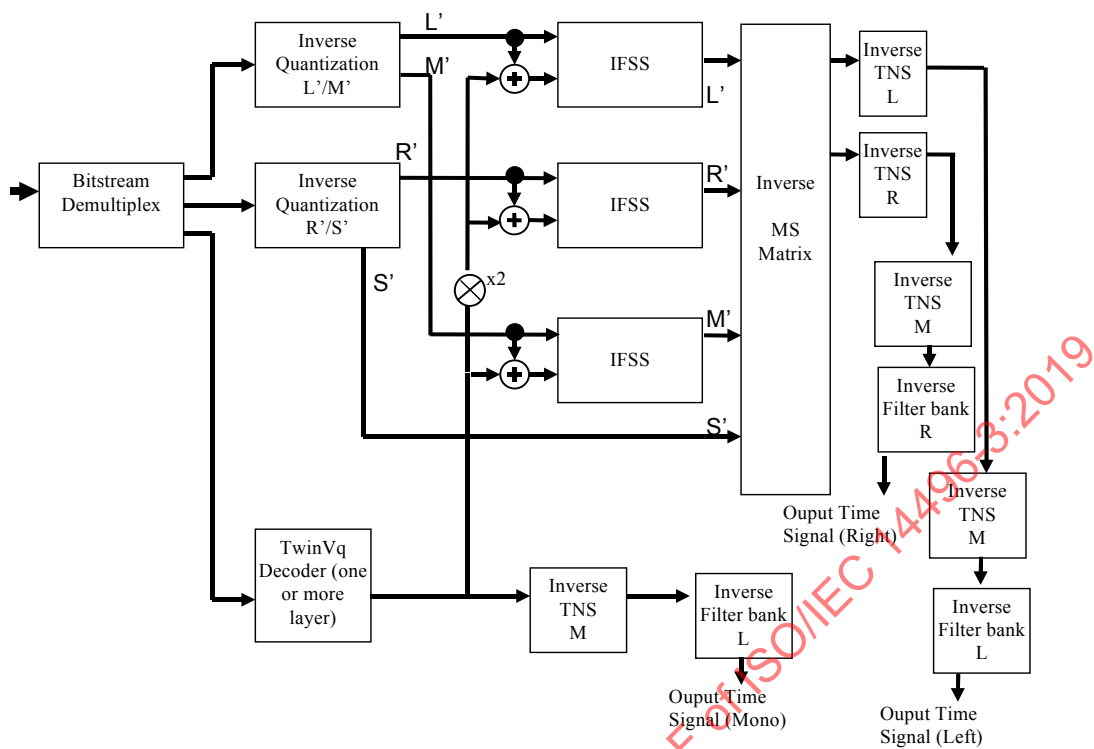
Figure 4.15 – Decoding of a TwinVQ (mono) + AAC (stereo) configuration, if TNS is used in the first TwinVQ layer
