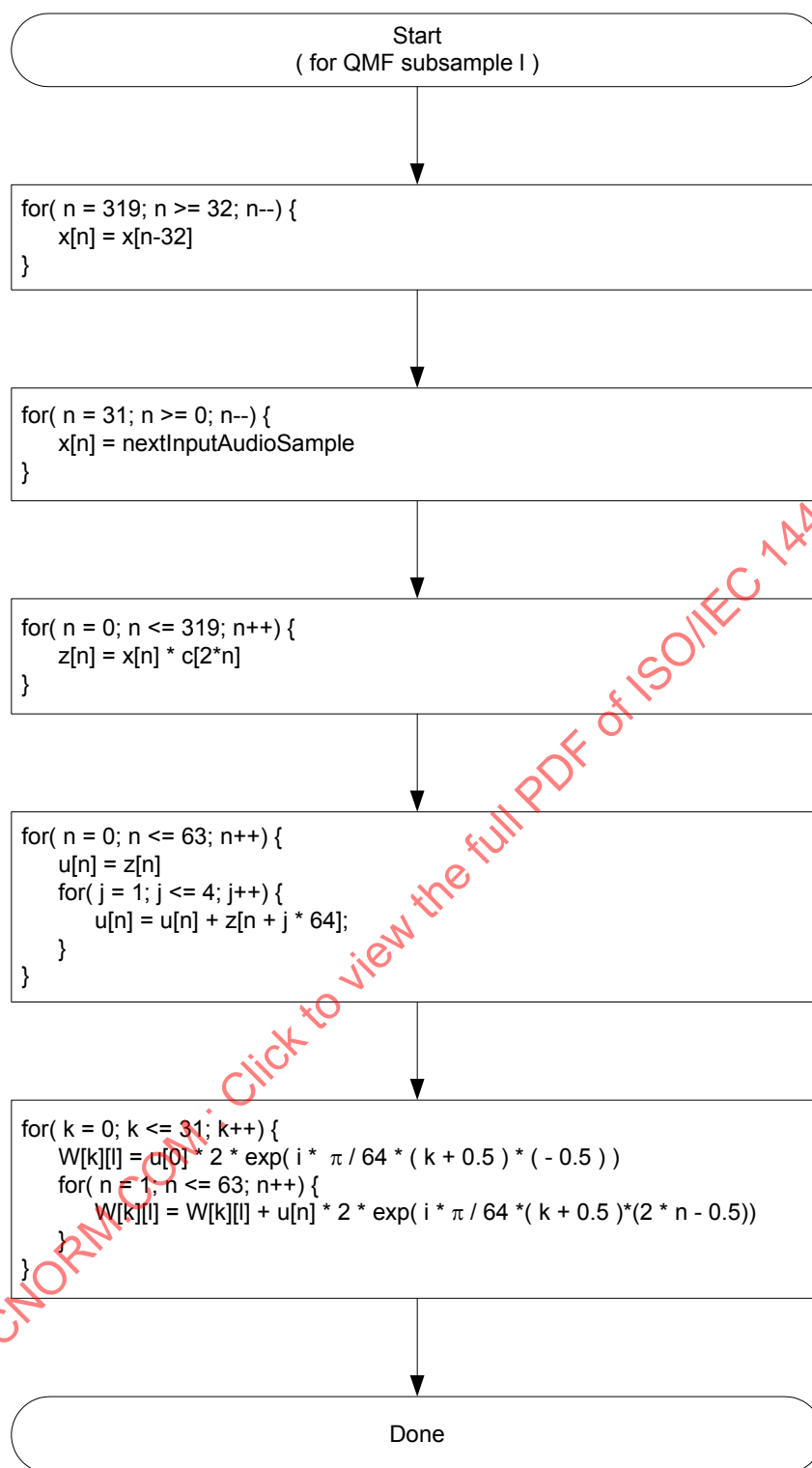
Figure 4.42 – Flowchart of decoder analysis QMF bank
