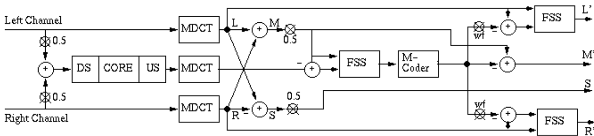
Figure 4.B.5 – Core + mono GA + stereo GA
