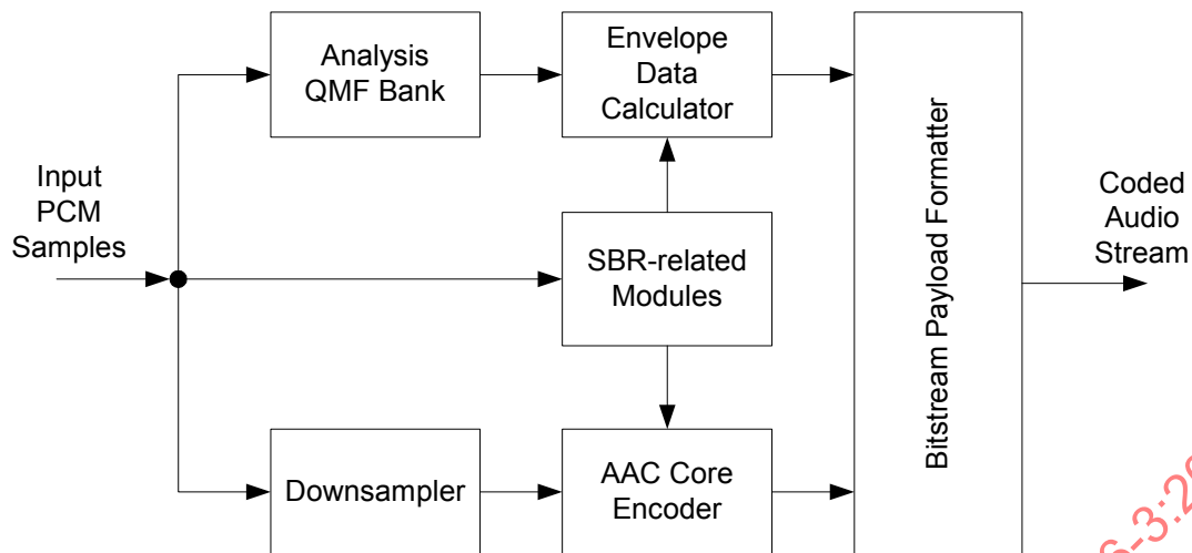
Figure 4.B.15 – Encoder overview
