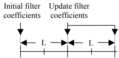
Figure 8.18 — In order to set the initial states of the filter, the final states after the generation of an interval of 2L samples are copied into the initial states for the generation of the next interval of 2L samples
