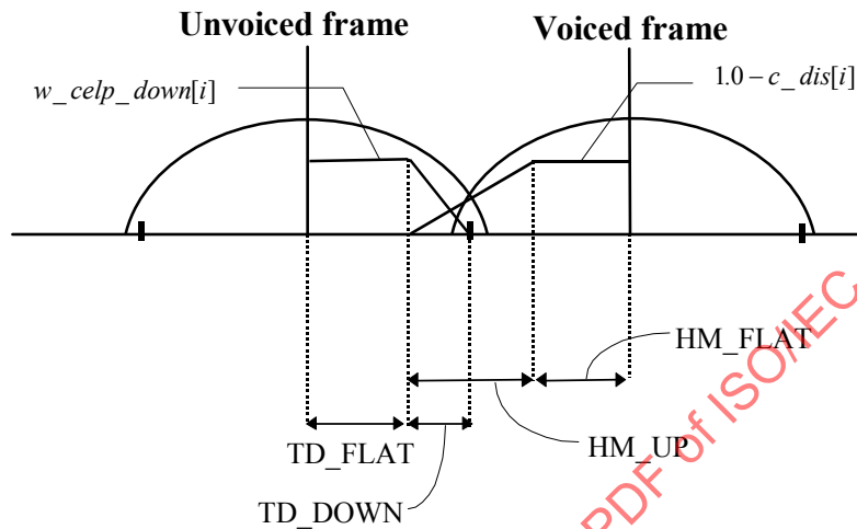
Figure 2.11 — Synthesis window for unvoiced/voiced
