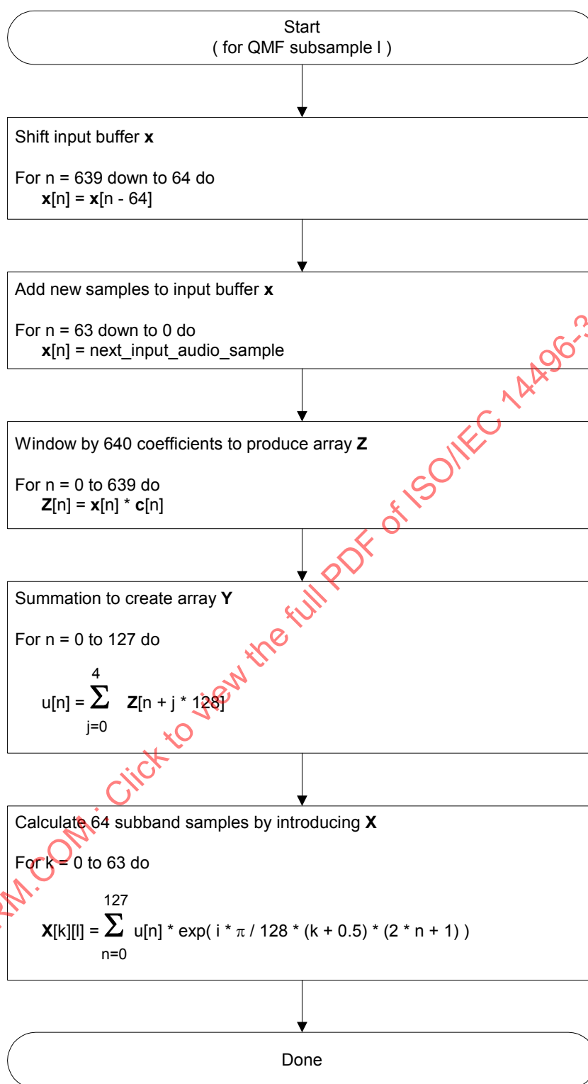
Figure 4.B.16 – Flowchart of encoder analysis QMF bank
