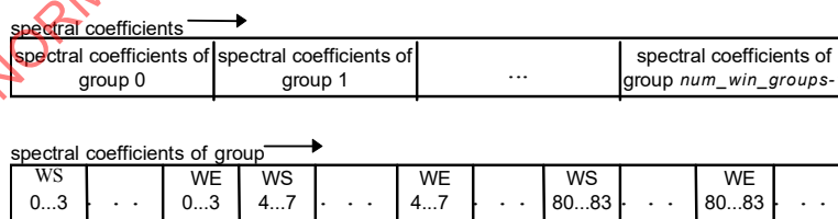
Order of spectral data for EIGHT_SHORT_SEQUENCE
