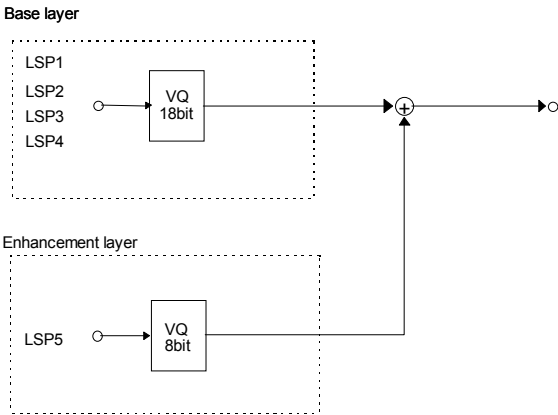
Figure 2.5 — LSP decoder
