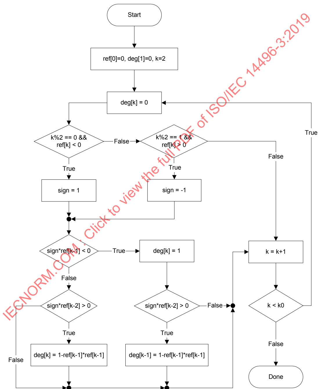
Figure 4.53 – Flowchart of the calculation of the aliasing degree
