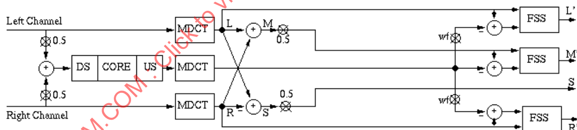
Figure 4.B.4 – Core + stereo GA
