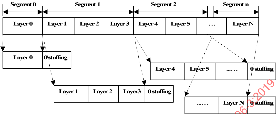
Figure 4.28 – Decoding of SBA bitstream payload
