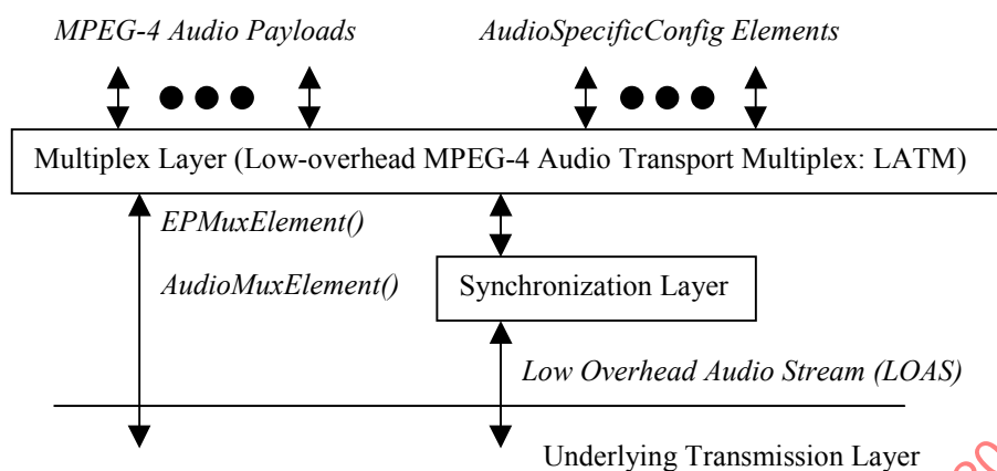
Figure 1.3 – Concept of MPEG-4 Audio Transport
