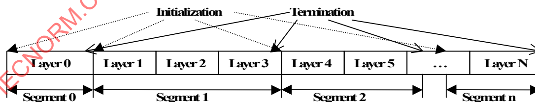
Figure 4.27 – The structure of SBA coded bitstream payload
