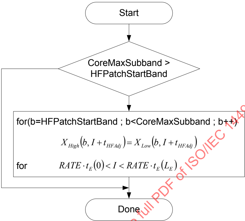
Figure 4.131 – Flowchart of HF-Overlap
