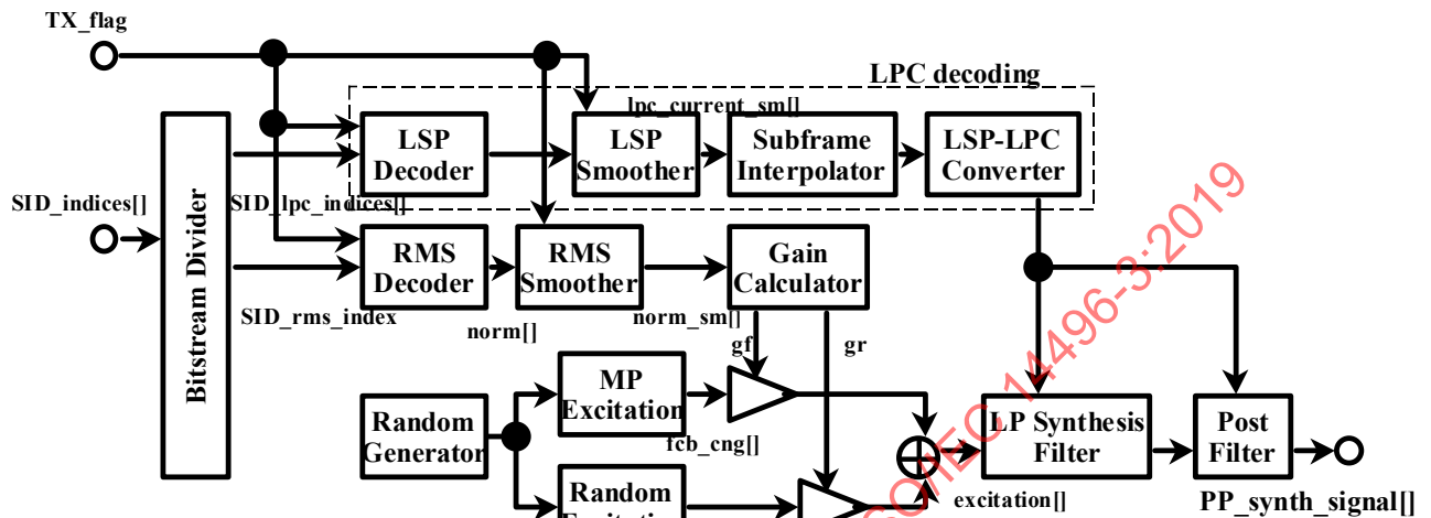
Figure 3.11 — CNG module
