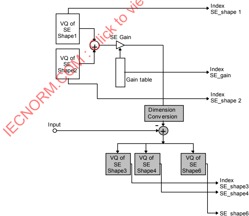
Figure 2.A.2 — Vector quantization of spectral envelope
