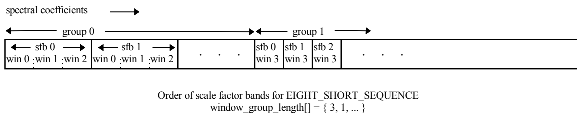
Figure 4.24 – Spectral order of scalefactor bands in case of EIGHT_SHORT_SEQUENCE
