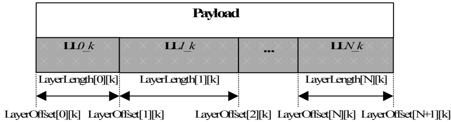
Figure 4.17 – Structure of the payload
