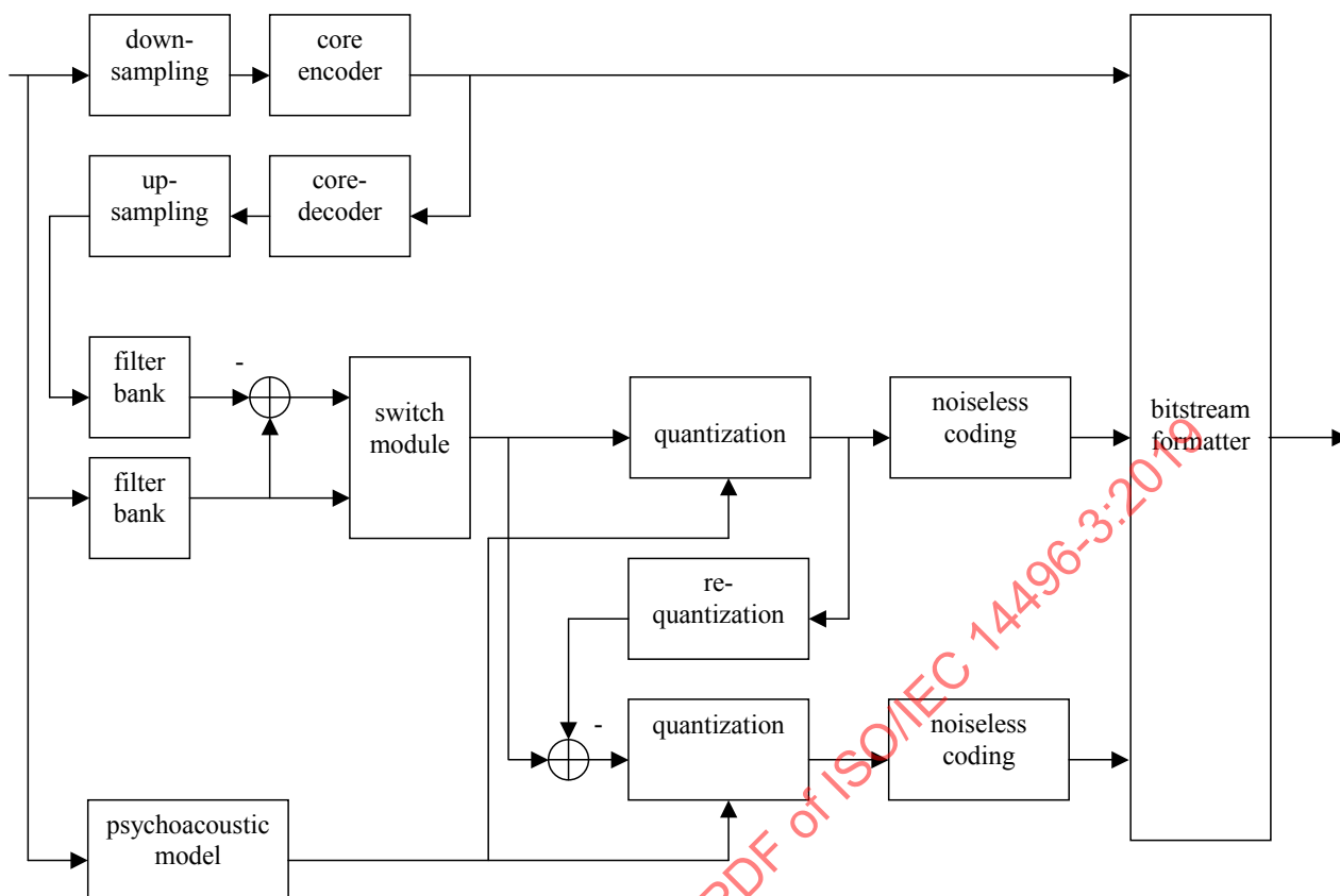
Figure 4.B.3 – Encoder process
