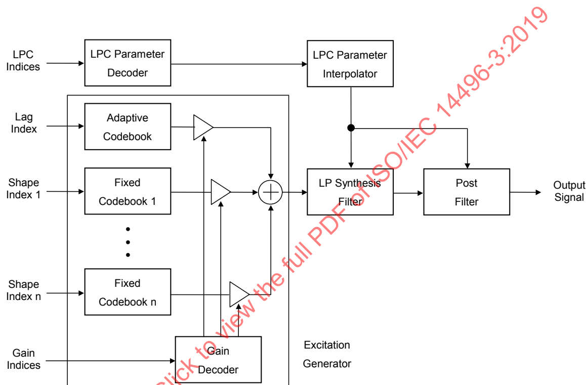
Figure 3.1 — Block diagram of a CELP decoder
