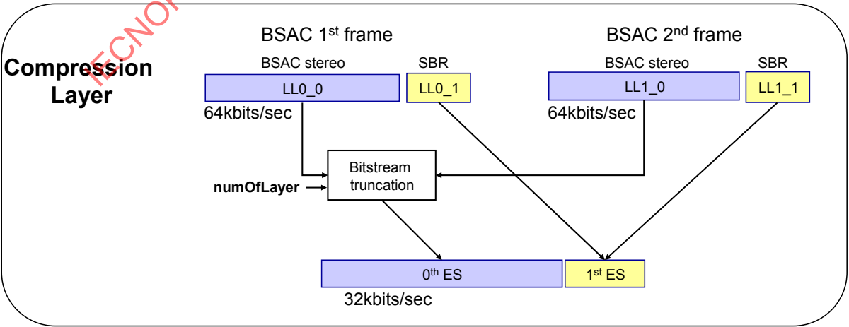
Figure 4.B.12 – Scalable transmission of BSAC and SBR payload by the bitstream truncation
