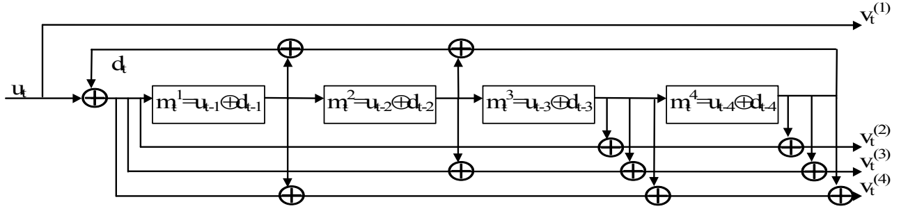
Figure 1.10 – Shift register realization for systematic recursive convolutional encoder
