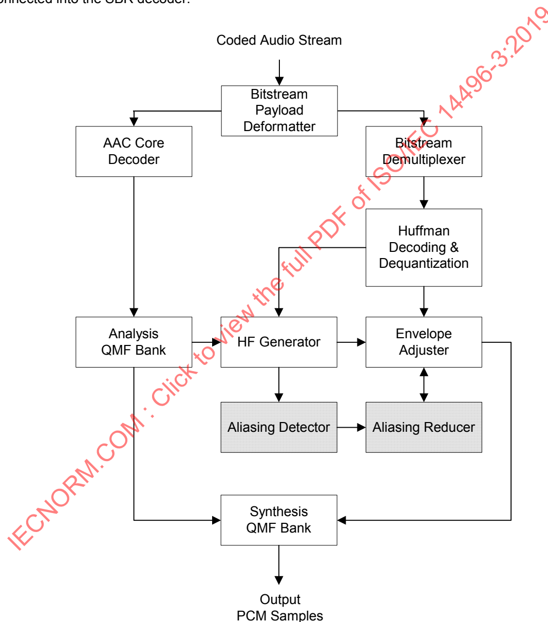
Figure 4.49 – Block diagram of the SBR low power decoder
