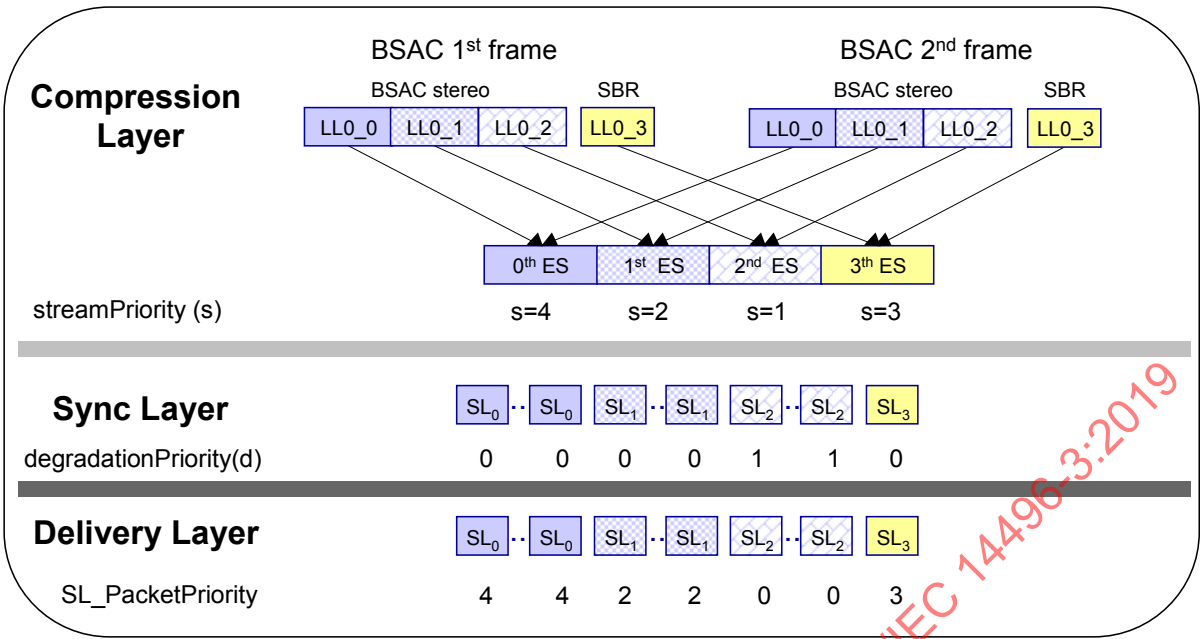
Figure 4.B.11 – Scalable transmission of BSAC and SBR payload
