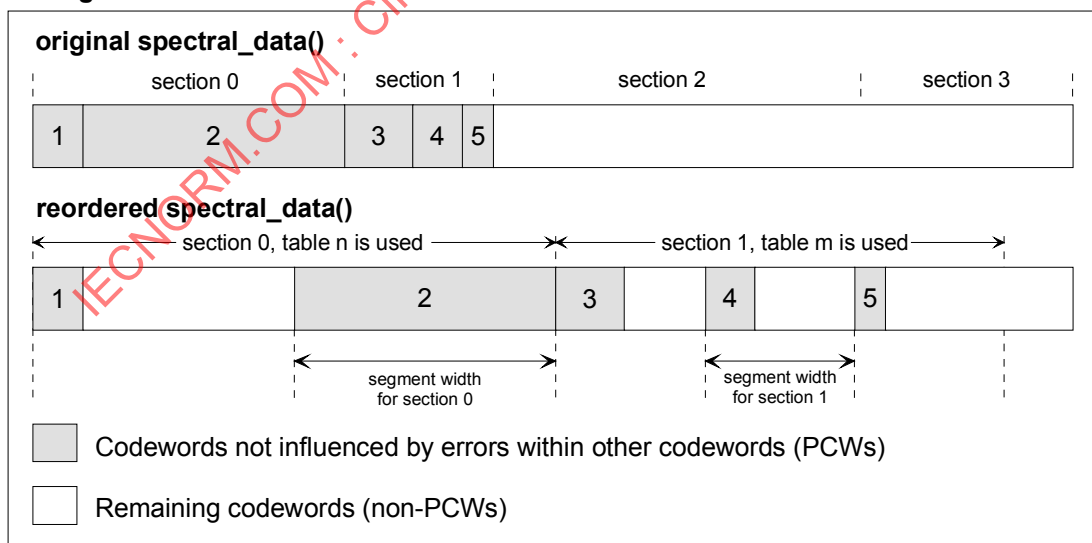
Figure 4.35 – General scheme of segmentation and arrangement of PCWs
