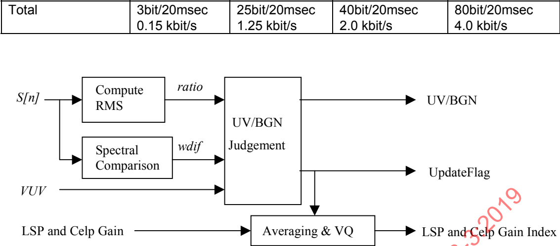
Figure 2.A.5 — Additional Blockdiagram for Encoder
