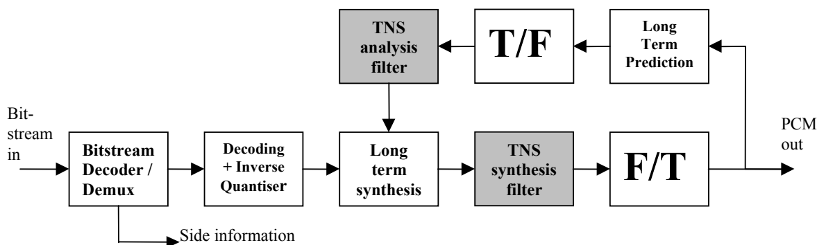
Figure 4.31 – Long Term Prediction with TNS
