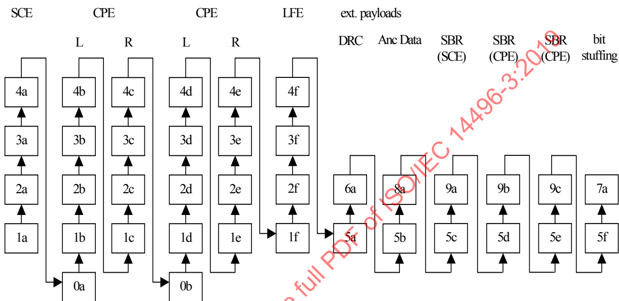
Figure 4.25 – Dependency structure in the case of error resilient multichannel AAC syntax (channelConfiguration == 6)
