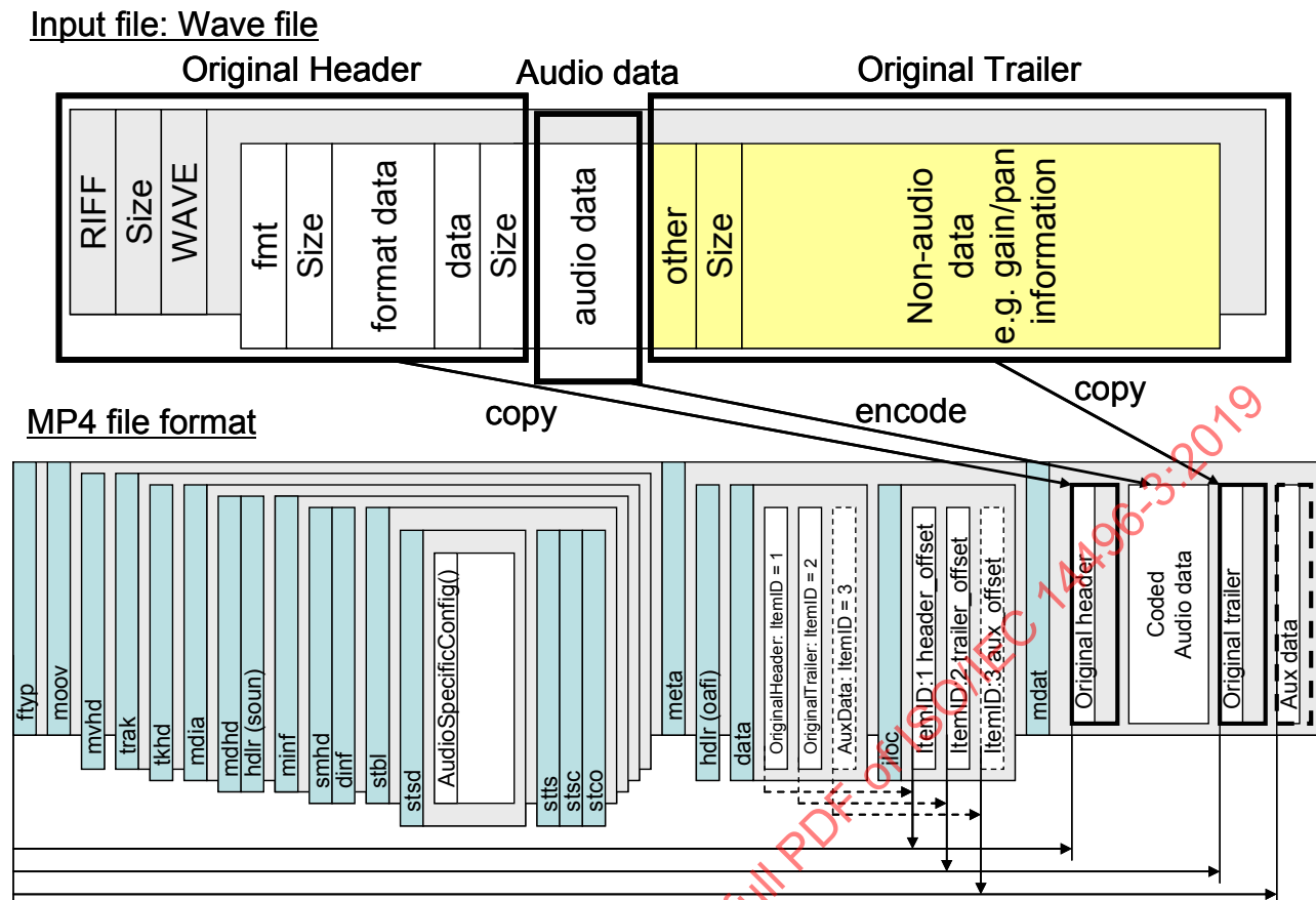
Figure 1.2 – Possible order of blocks
