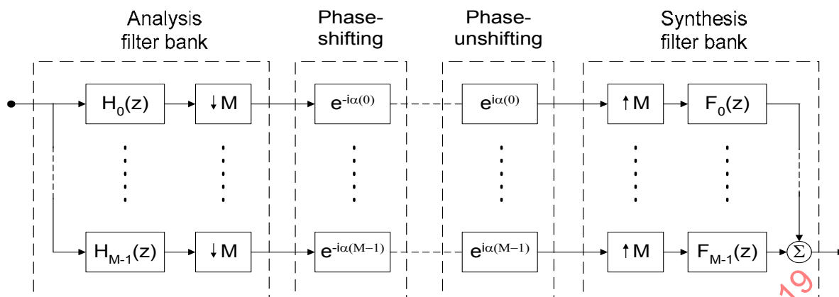
Figure 4.56 – Phase-shifting of subbands in complex-exponential modulated filter banks
