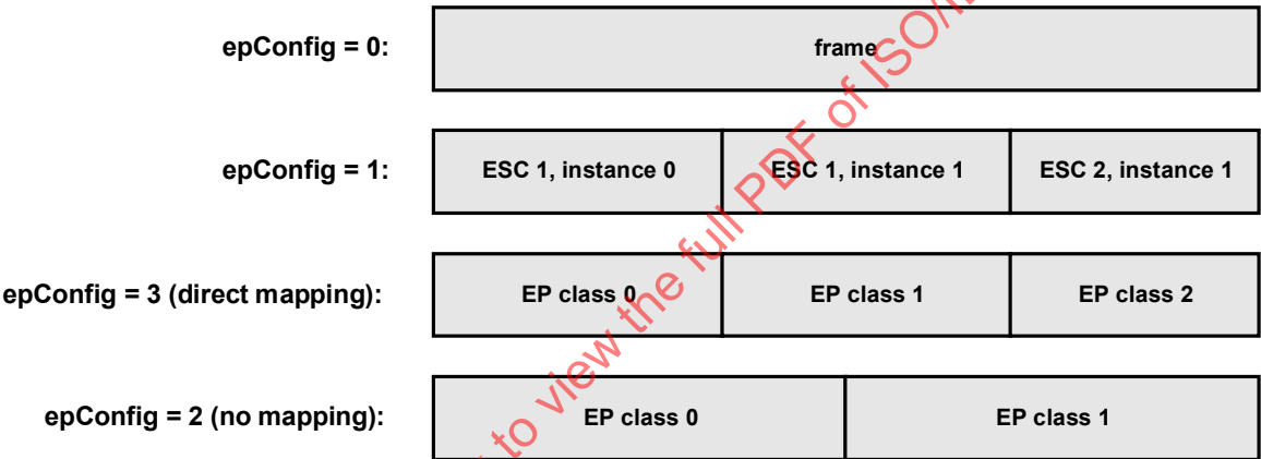
Figure 1.6 – EP classes for different epConfig values
