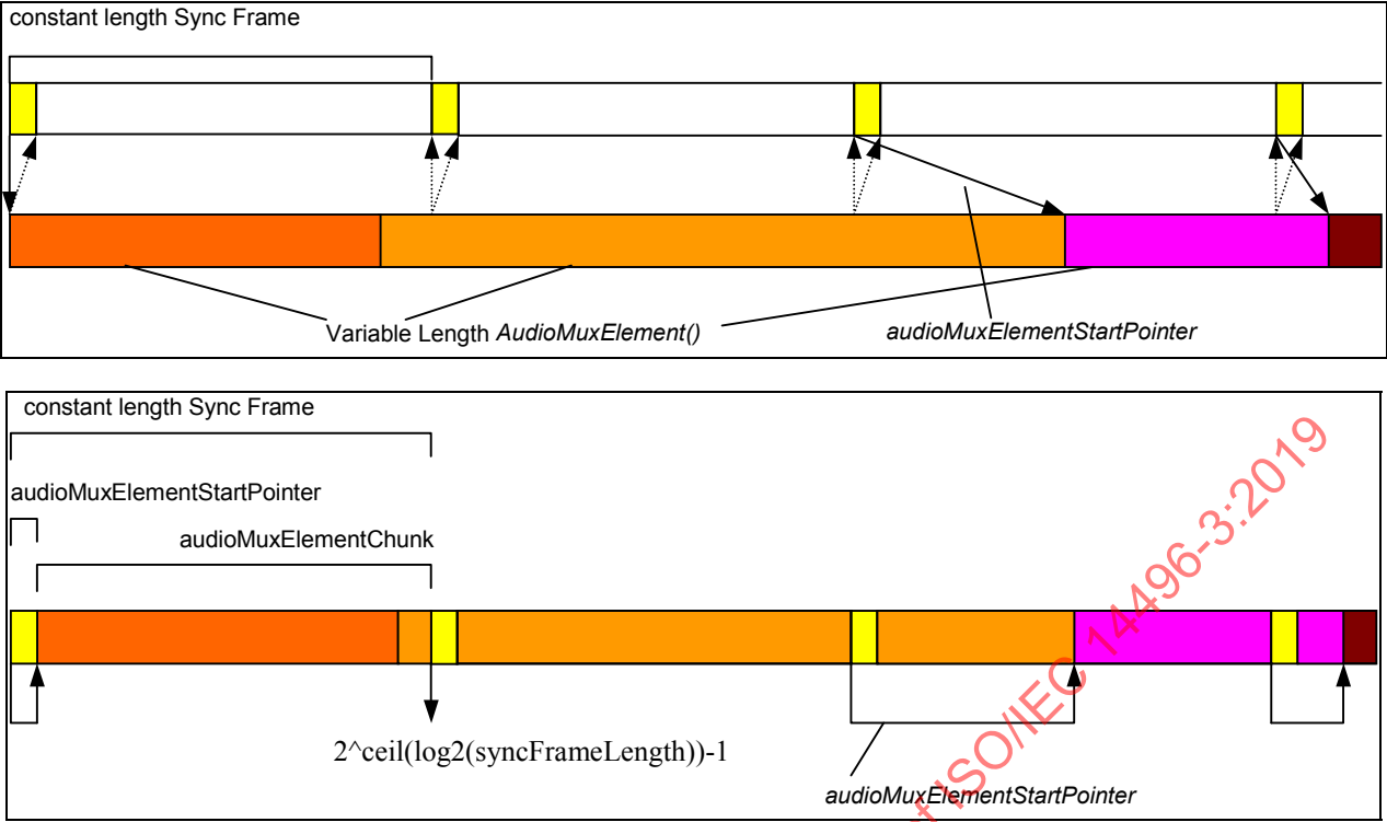
Figure 1.4 – Synchronization in AudioPointerStream()
