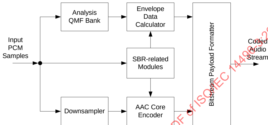
Figure 4.B.15 – Encoder overview
