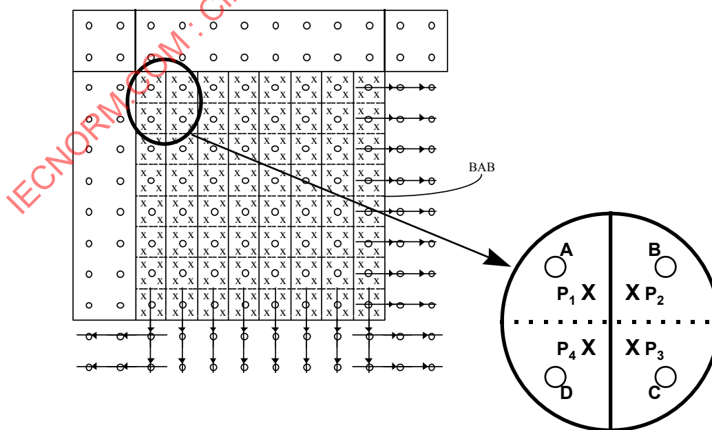
Figure 7-13 -- Upsampling
