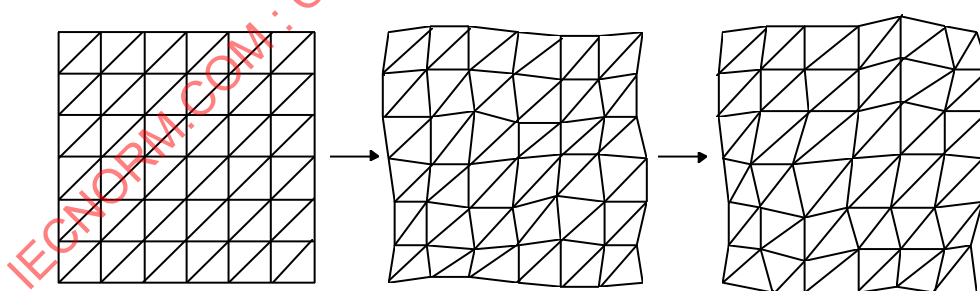
Figure 6-8 -- Mesh object with uniform triangular geometry
