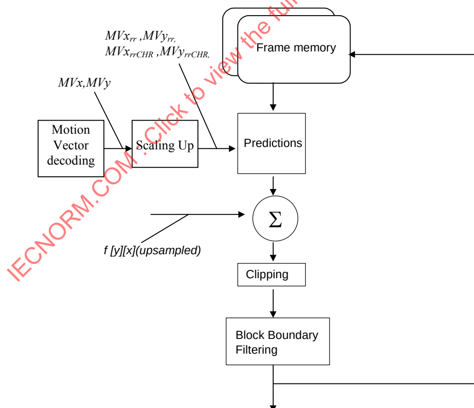
Figure V2 -19 -- Motion Compensation Decoding of Reduced Resolution VOP
