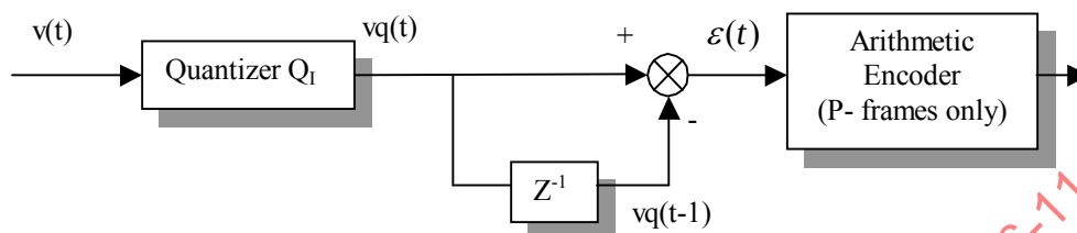
Figure 62 — BIFS Anim encoding process. Z^{-1} stands for one frame delay. The value v(t) at frame t is quantized with Quantizer Q_1 and the difference \varepsilon(t) with the previous quantized value vq(t-1) at frame t-1 is adaptively arithmetic encoded.
