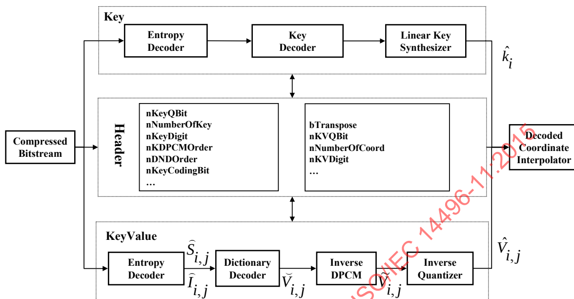
Figure 50 — Decoder for compressed coordinate interpolator
