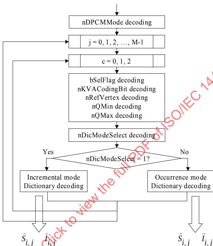
Figure 51 — Flowchart of entropy decoding
