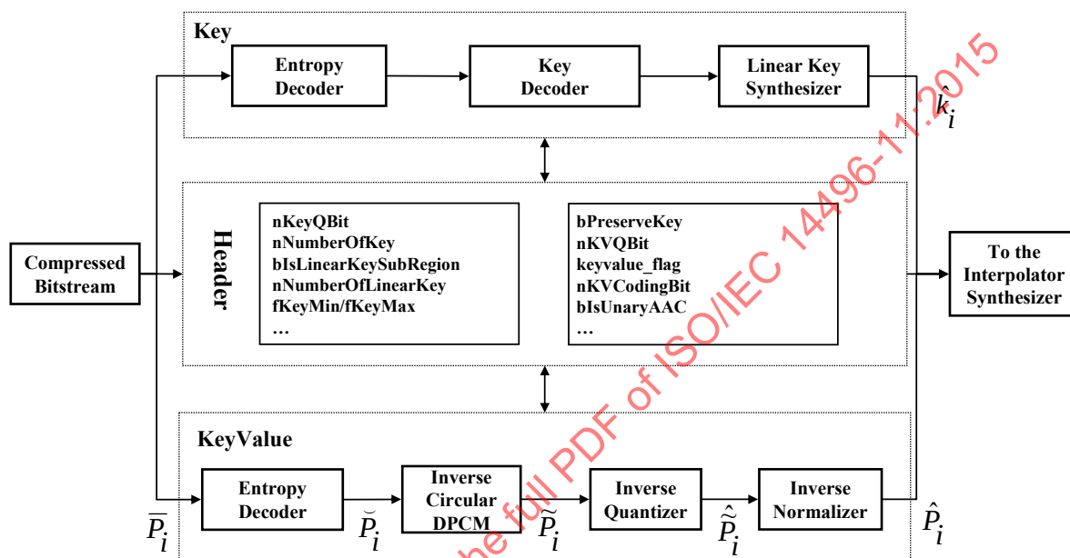
Figure 59 — Decoder structure for compressed position interpolator
