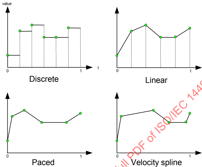
Figure 28 – Predefined types of timelines: discrete, linear, paced (constant speed), and velocity spline. The first type ( keyType 0) is not shown and is user-specified. Note how the animation paths are identical but the timelines so different.
