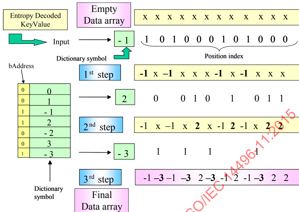
Figure 54 — An example of incremental mode decoding
