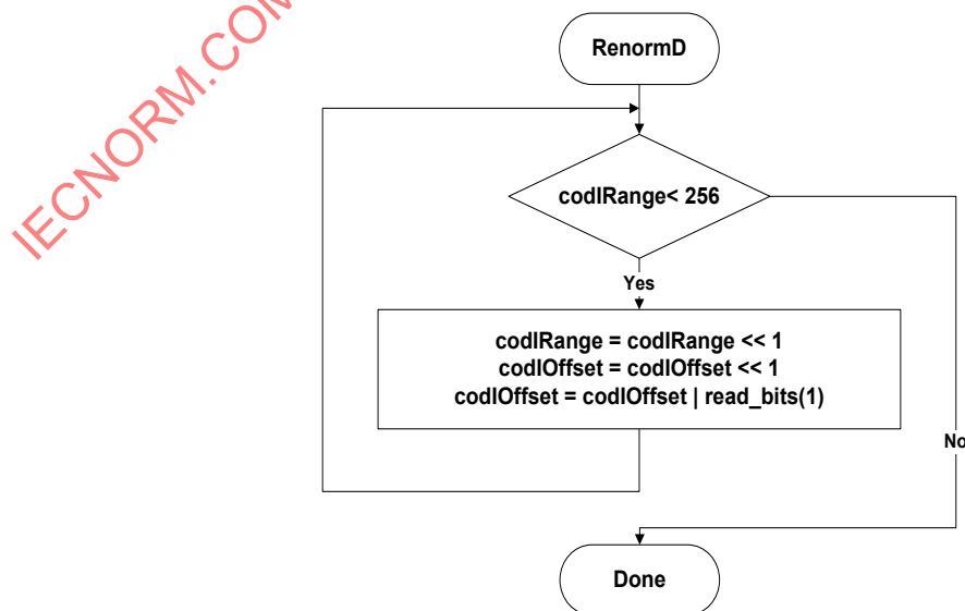
Figure 9-4 – Flowchart of renormalization
