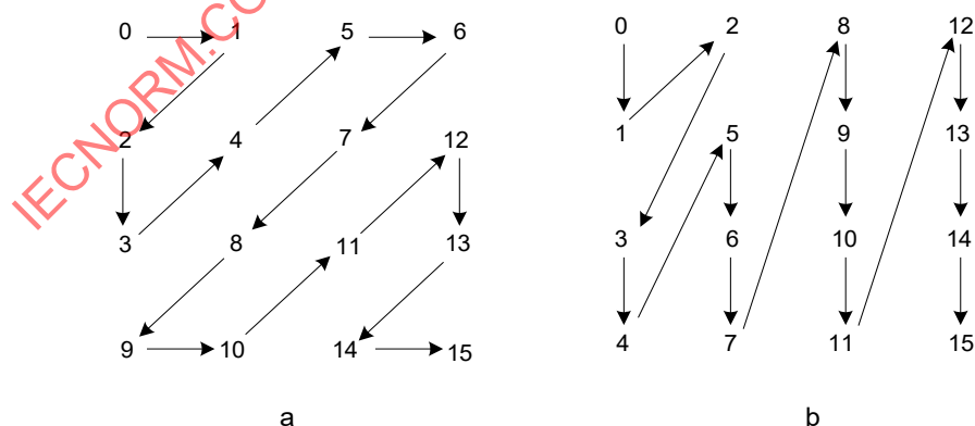
Figure 8-8 – 4x4 block scans. (a) Zig-zag scan. (b) Field scan (informative)
