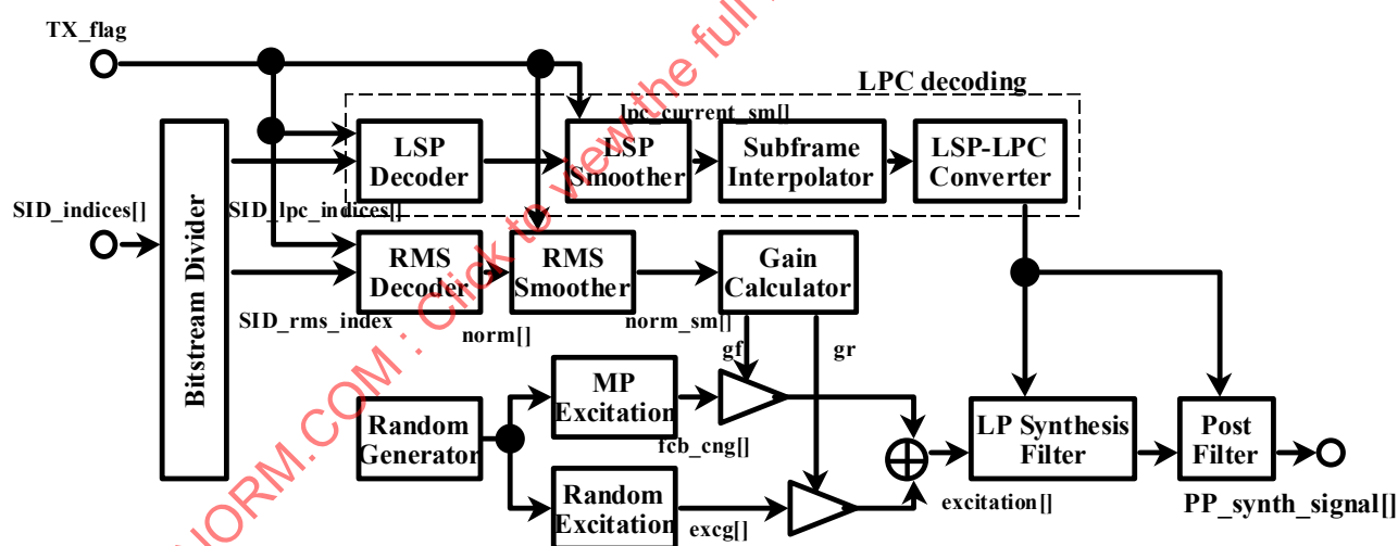
Figure 3.11 — CNG module
