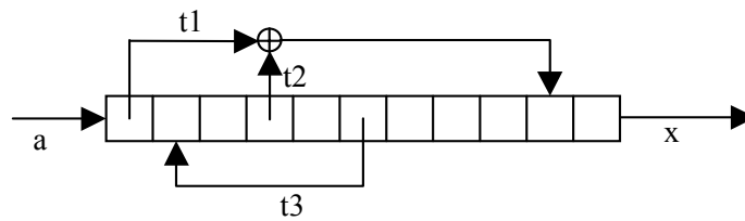
Figure 5.4 — Block diagram for 'fracdelay' example
