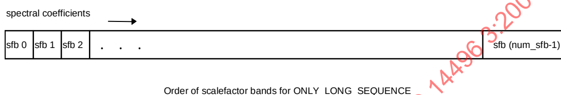
Figure 4.18 – Order of scalefactor bands for ONLY_LONG_SEQUENCE
