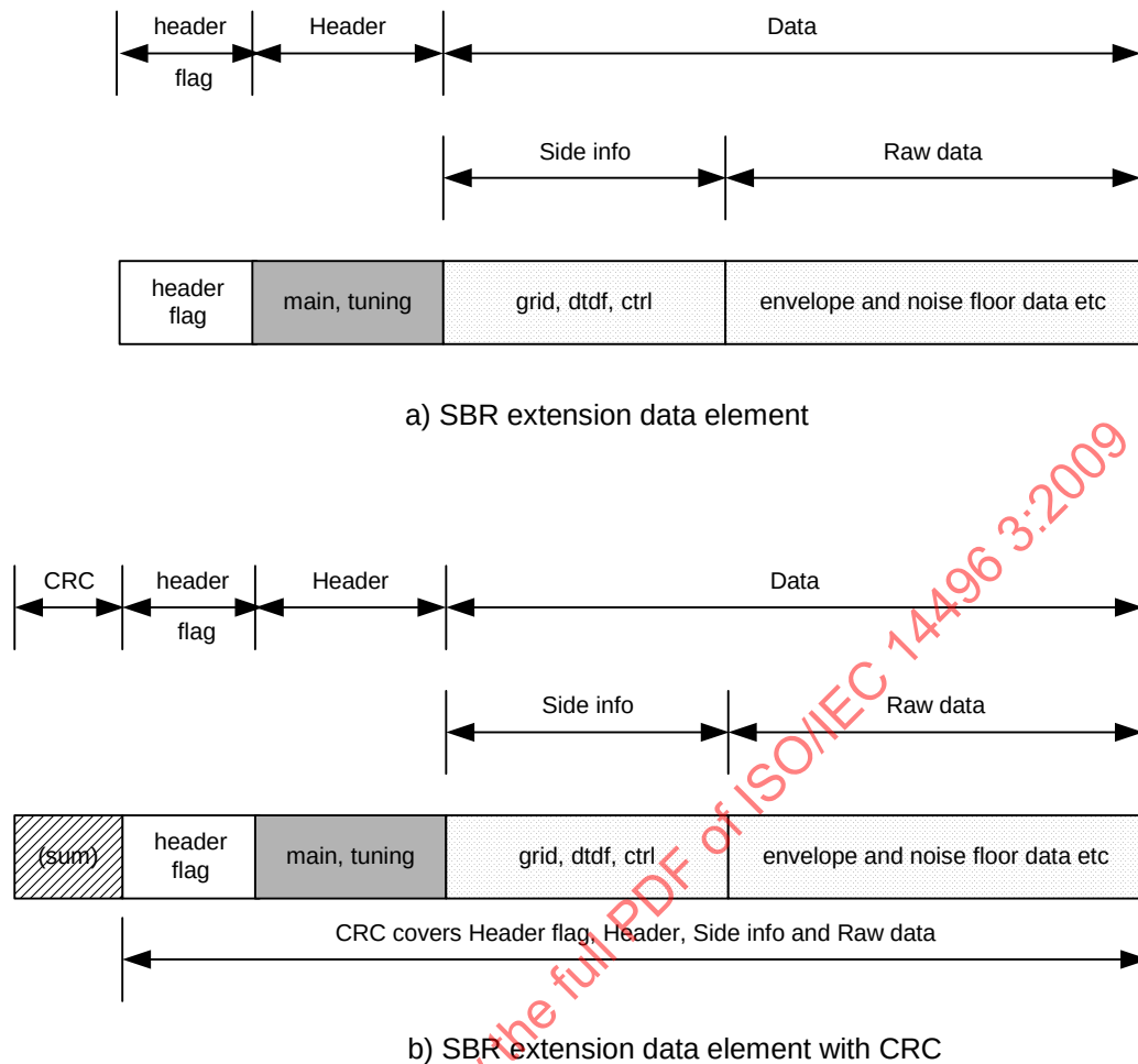
Figure 4.21 – The basic sections of the SBR extension data elements
