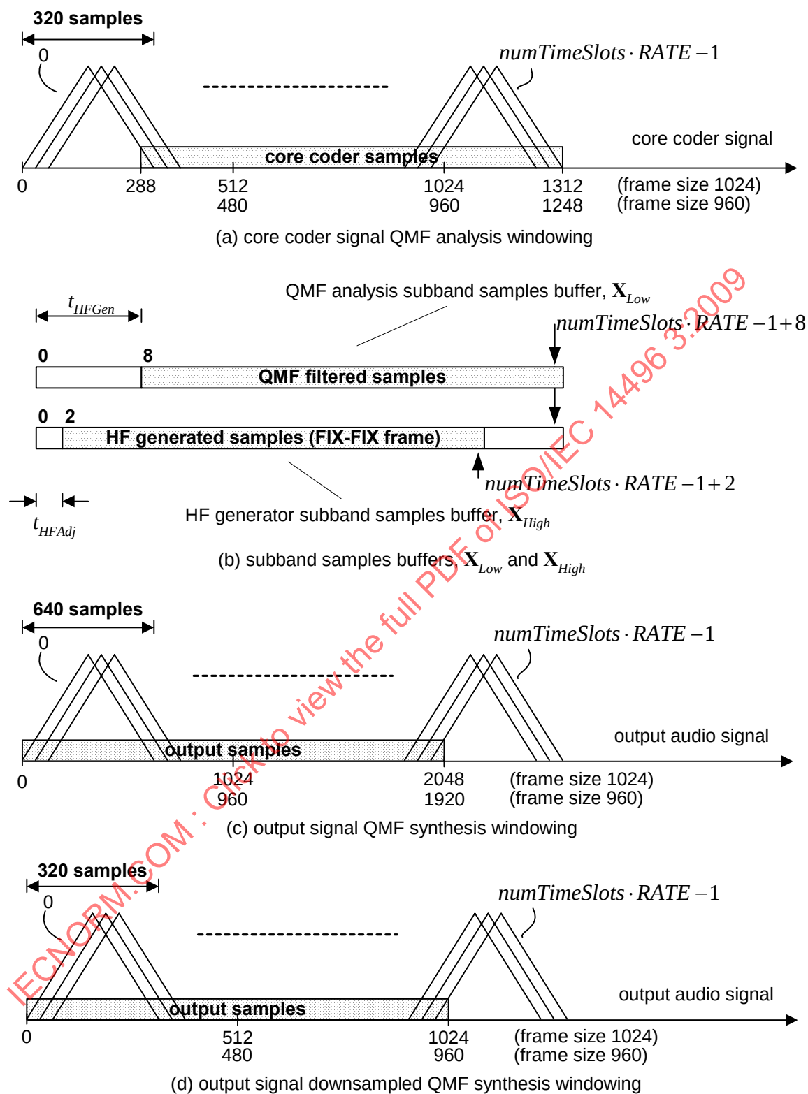
Figure 4.47 – Synchronization and timing
