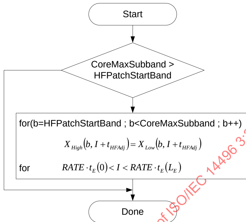
Figure 4.125 – Flowchart of HF-Overlap
