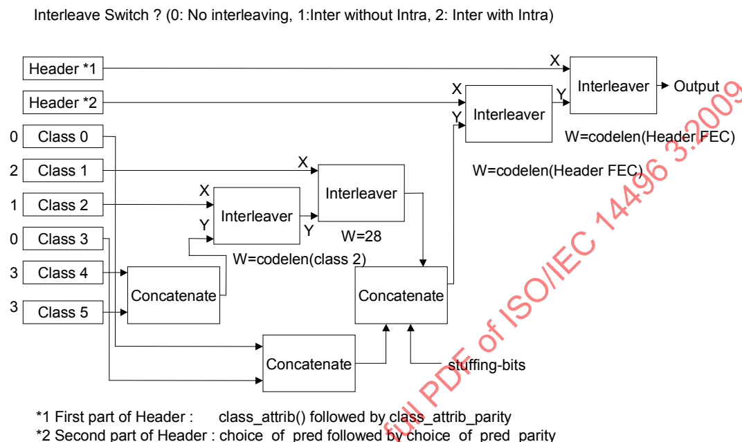
Figure 1.19 – Interleave process with class-wise control of interleaving
