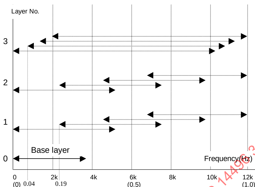
Figure 4.30 – Example of adaptive active band selection. (Sampling_Frequency=24kHz, Total bitrate=40kb/s(8+8+8+16kbps) In this case, q_{\text{sample}} = 0.43 , \text{bias} = 0.19 for layer 1 and layer 2 q_{\text{sample}} = 0.87 , \text{bias} = 0.04 for layer 3)
