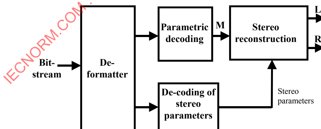
Figure 8.1 — Illustration of the integration of the stereo coding tools into the parametric decoder
