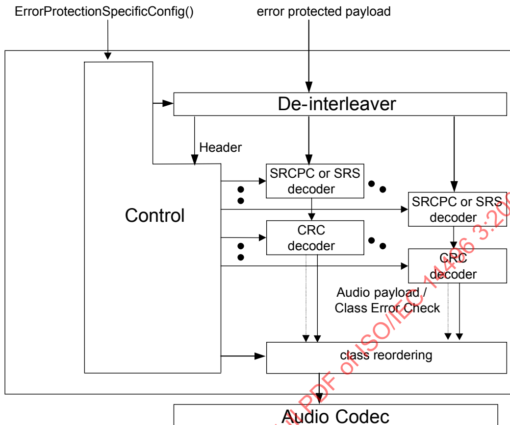
Figure 1.8 – Outline of EP decoder
