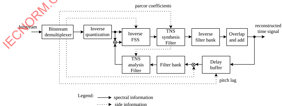
Figure 4.37 – Decoder structure
