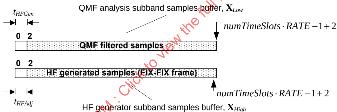
Figure 4.55 – Synchronization for low delay SBR
