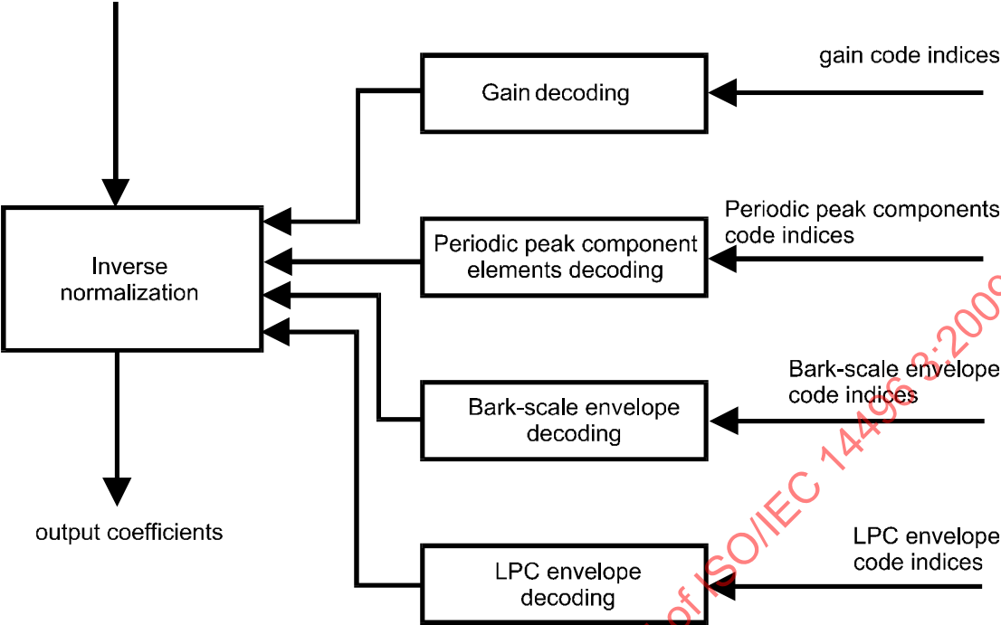
Figure 4.32 – Decoding process of the TwinVQ
