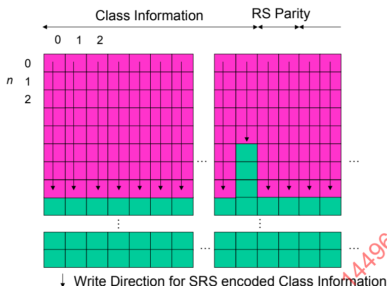
Figure 1.18 – Interleaving matrix in RS encoded class case
