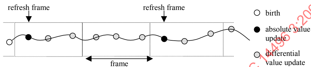
Figure 8.4 — Example for updating of a track. For every other frame, the track continuations are updated by their absolute values. In the case decoding starts at refresh_sinusoids == %0 , the differential updates will be ignored until a refresh_sinusoids == %1 or a birth is received
