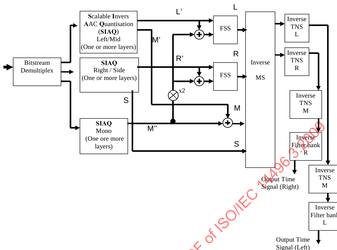
Figure 4.4 – AAC mono / AAC stereo configuration (AAC-Only-M/S)
