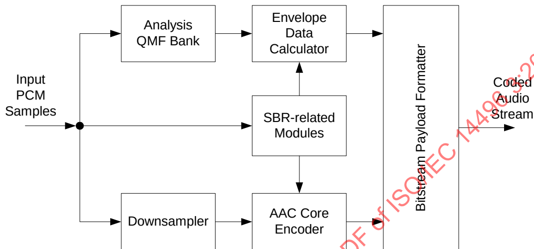
Figure 4.B.15 – Encoder overview
