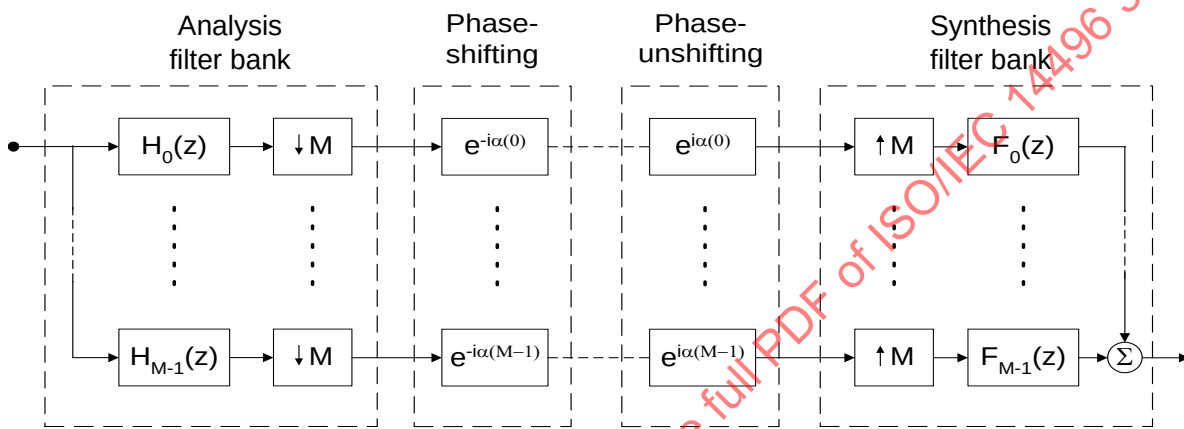
Figure 4.56 – Phase-shifting of subbands in complex-exponential modulated filter banks
