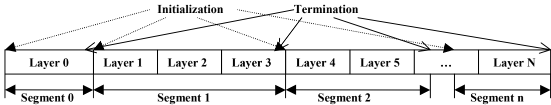
Figure 4.27 – The structure of SBA coded bitstream payload
