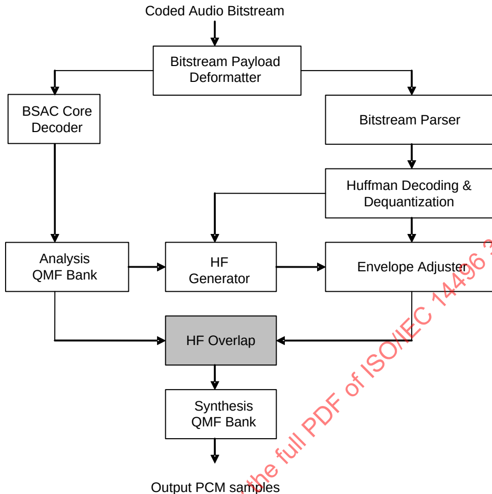
Figure 4.124 – Overview of the integration of ER BSAC and SBR decoder
