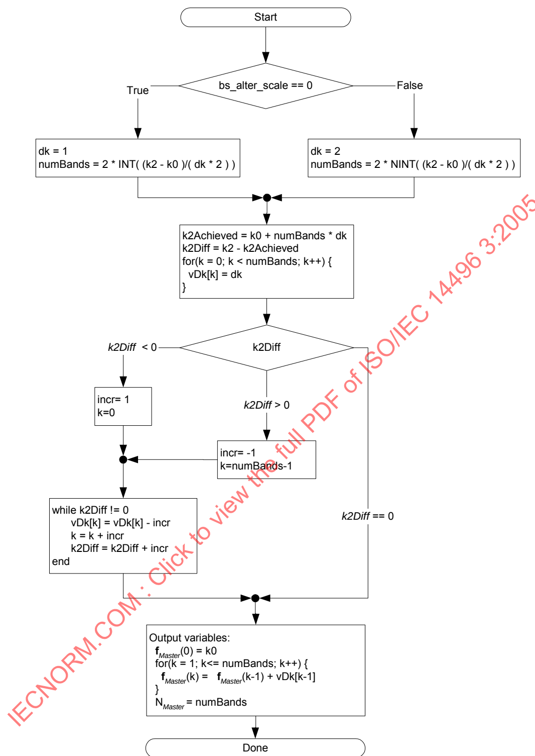
Figure 4.38 – Flowchart calculation of f_{Master} when bs\_freq\_scale = 0
