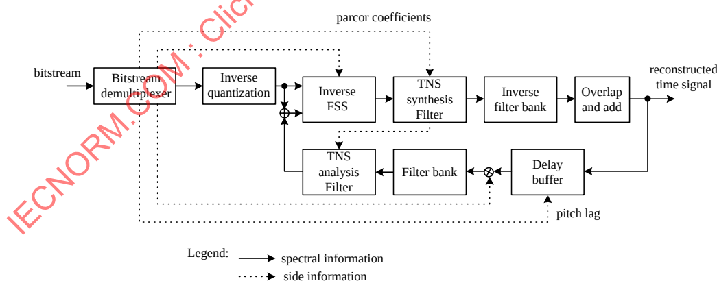
Figure 4.36 – Decoder structure
