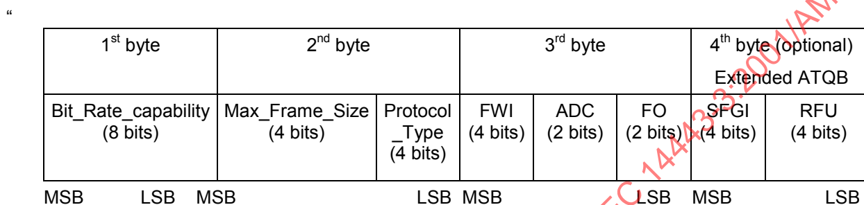
Figure 25 — Protocol Info format
