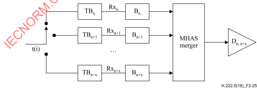
Figure 2-25 – Transport stream system target decoder for multiple audio elementary streams
