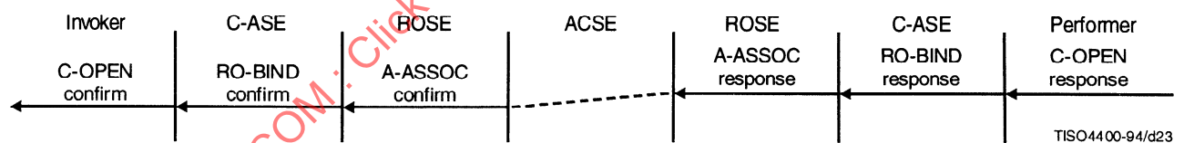
Figure 23 – Realization of a bind result using ACSE services
