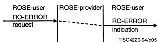
Figure 5 – RO-ERROR service primitives
