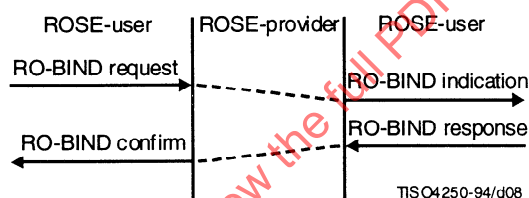
Figure 8 – RO-BIND service primitives
