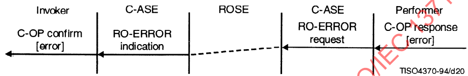
Figure 20 – Realization of performer reporting error
