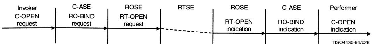
Figure 26 – Realization of a bind request using RTSE services
