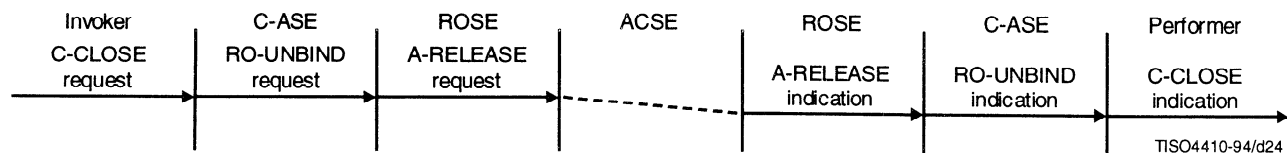
Figure 24 – Realization of an unbind using ACSE services
