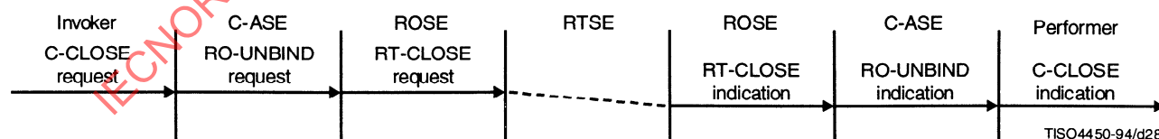
Figure 28 – Realization of an unbind request using RTSE services
