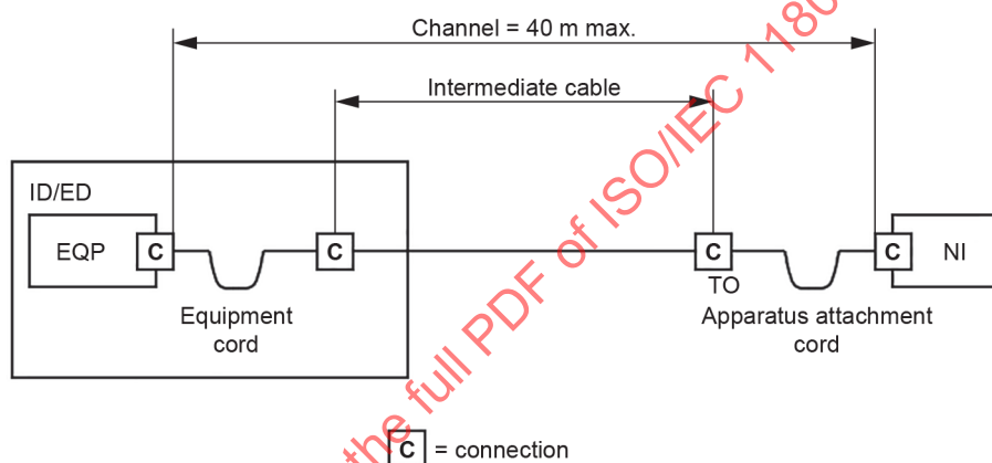
a) Interconnect – TO model balanced 1-pair cabling channel 40 m
