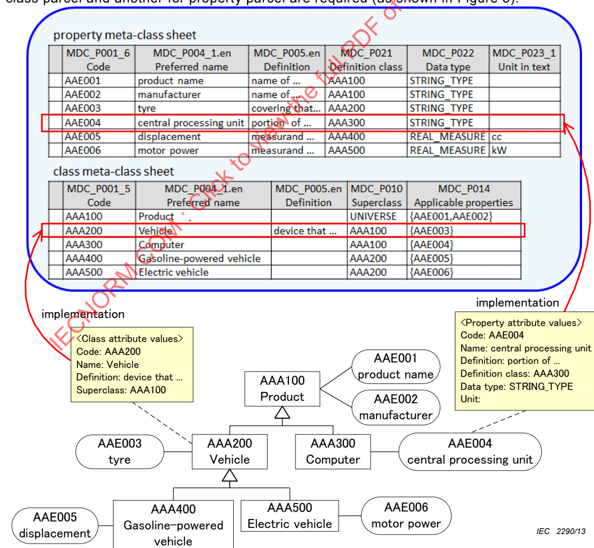
Figure 3 – Spreadsheet implementation
