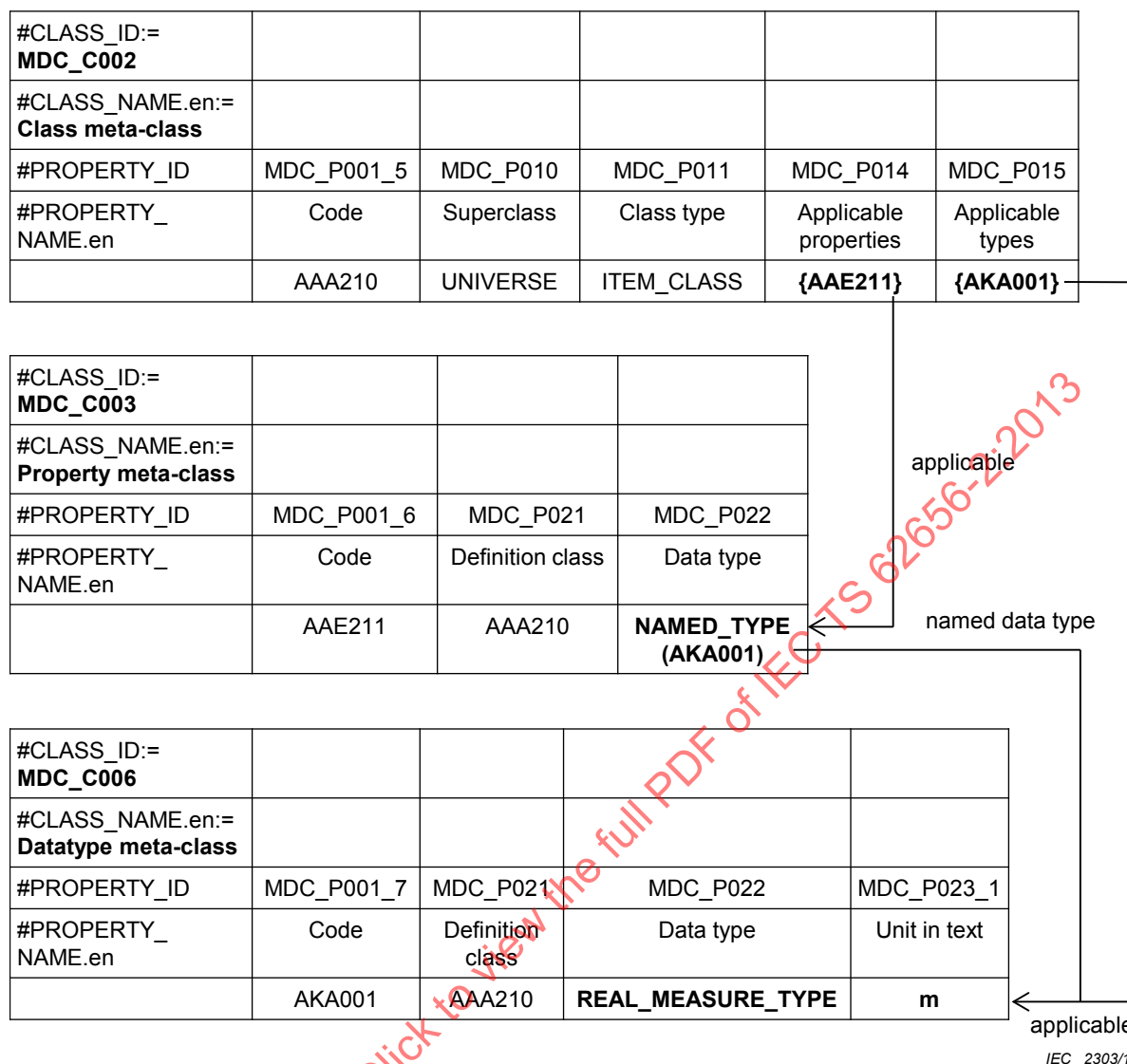
Figure 16 – Parcel implementation for named data types
