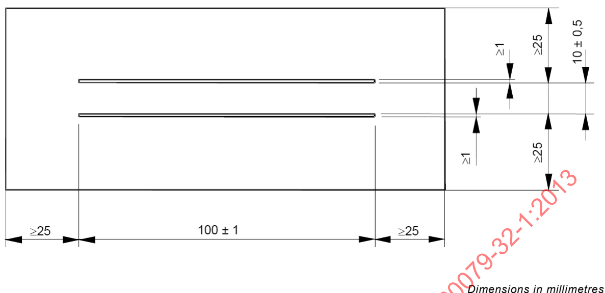
Figure G.1 – Test sample with applied electrodes
