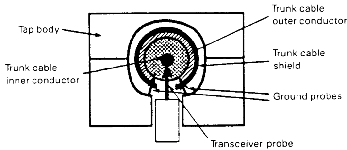
TAP CONNECTOR
