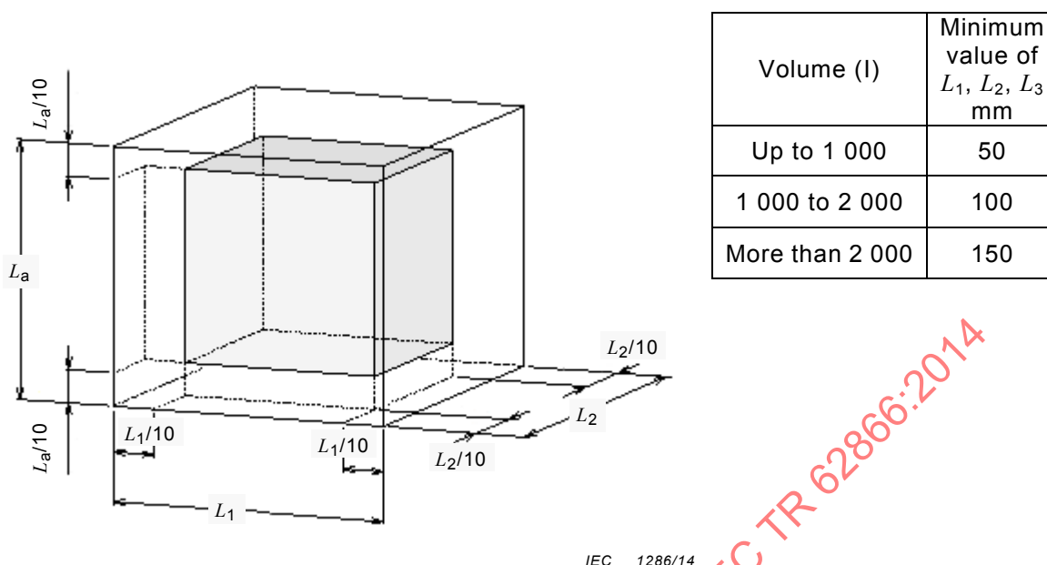
Figure 15 – Effective space in a test chamber
