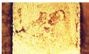
Figure 31 – Migration generated in the water drop test
